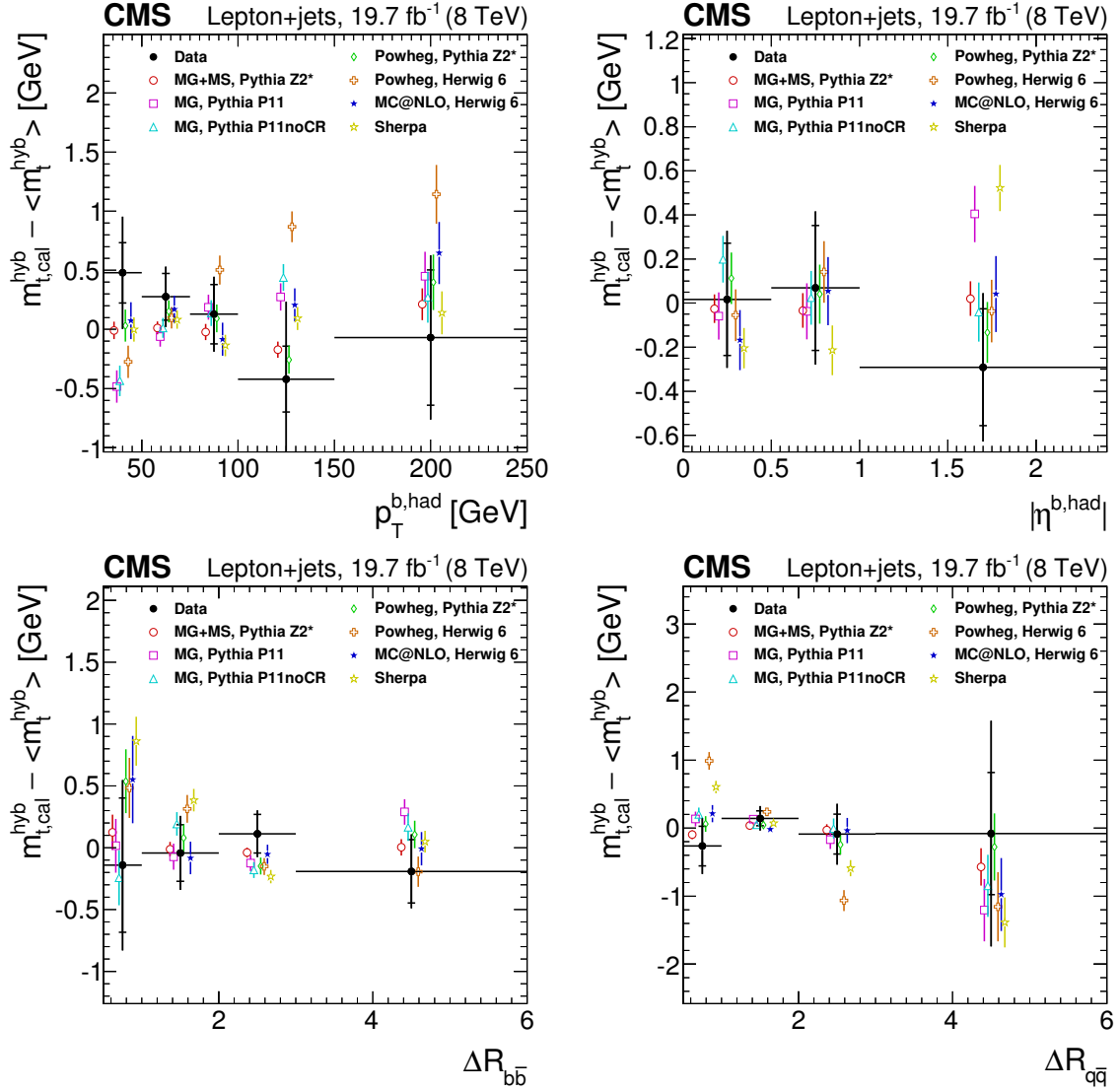
Figure 10: Measurements of m_t as a function of the p_T of the b jet assigned to the hadronic decay branch ( p_T^{b, \text{had}} ), the pseudorapidity of the b jet assigned to the hadronic decay branch ( |\eta^{b, \text{had}}| ), the \Delta R between the b jets ( \Delta R_{bb} ), and the \Delta R between the light-quark jets ( \Delta R_{q\bar{q}} ). The filled circles represent the data, and the other symbols are for the simulations. For reasons of clarity the horizontal error bars are shown only for the data points and each of the simulations is shown as a single offset point with a vertical error bar representing its statistical uncertainty. The statistical uncertainty of the data is displayed by the inner error bars. For the outer error bars, the systematic uncertainties are added in quadrature. The open circles correspond to MADGRAPH with the PYTHIA Z2* tune, the open squares to MADGRAPH with the PYTHIA Perugia 2011 tune, and the open triangles represent MADGRAPH with the PYTHIA Perugia 2011 noCR tune. The open diamonds correspond to POWHEG with the PYTHIA Z2* tune and the open crosses correspond to POWHEG with HERWIG 6. The filled stars are for MC@NLO with HERWIG 6 and the open stars are for SHERPA.
