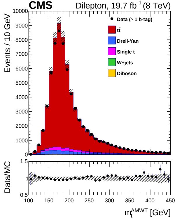
Figure 7: Distribution of m_t^{\text{AMWT}} for the collision and simulated data with m_t = 172.5 \text{ GeV} . The vertical bars show the statistical uncertainty and the hatched bands show the statistical and systematic uncertainties added in quadrature. The lower section of the plot shows the ratio of the yields between the collision data and the simulation.
