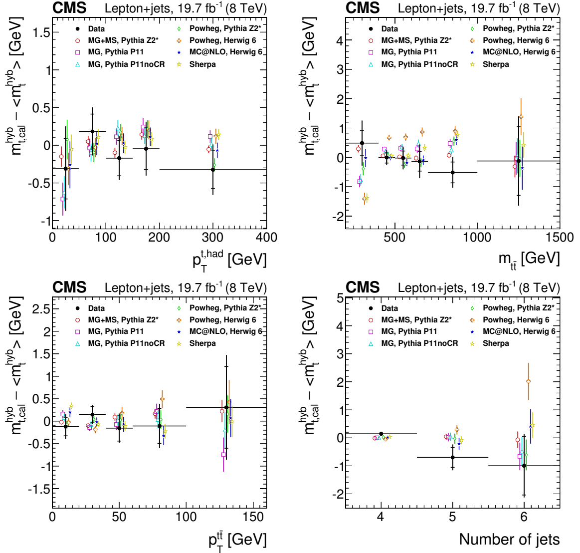
Figure 9: Measurements of m_t as a function of the transverse momentum of the hadronically decaying top quark ( p_T^{t, \text{had}} ), the invariant mass of the t\bar{t} system ( m_{t\bar{t}} ), the transverse momentum of the t\bar{t} system ( p_T^{t\bar{t}} ), and the number of jets with p_T > 30 GeV. The filled circles represent the data, and the other symbols are for the simulations. For reasons of clarity the horizontal error bars are shown only for the data points and each of the simulations is shown as a single offset point with a vertical error bar representing its statistical uncertainty. The statistical uncertainty of the data is displayed by the inner error bars. For the outer error bars, the systematic uncertainties are added in quadrature. The open circles correspond to MADGRAPH with the PYTHIA Z2* tune, the open squares to MADGRAPH with the PYTHIA Perugia 2011 tune, and the open triangles represent MADGRAPH with the PYTHIA Perugia 2011 noCR tune. The open diamonds correspond to POWHEG with the PYTHIA Z2* tune and the open crosses correspond to POWHEG with HERWIG 6. The filled stars are for MC@NLO with HERWIG 6 and the open stars are for SHERPA.
