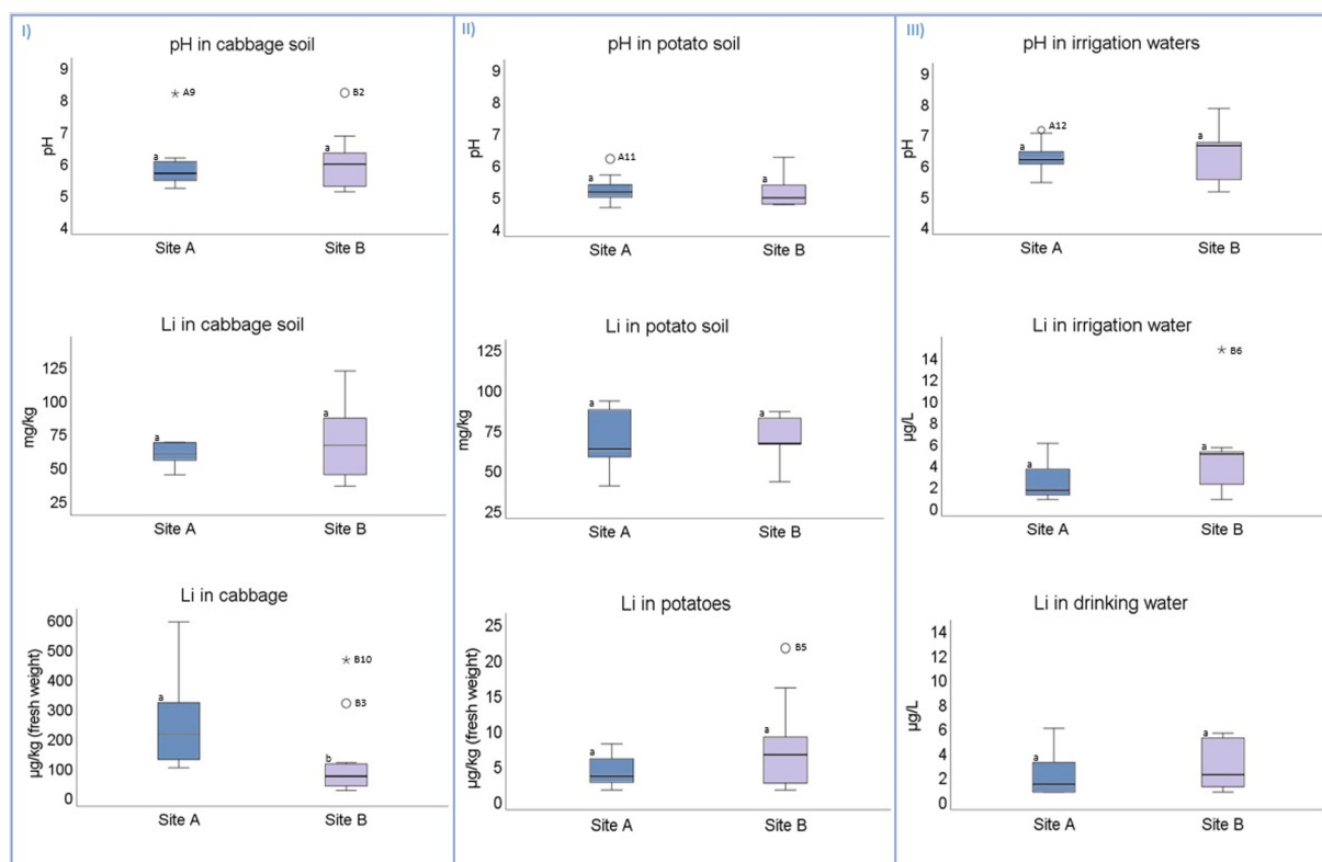
Fig. 3. Box-plots of pH values and Li concentrations in (I) cabbage related samples, (II) potato related samples, (III) drinking and irrigation water. Significant differences ( p < 0.05) between sites A and B are denoted by different lowercase letters. Outliers are denoted with \circ and extreme values with * .
