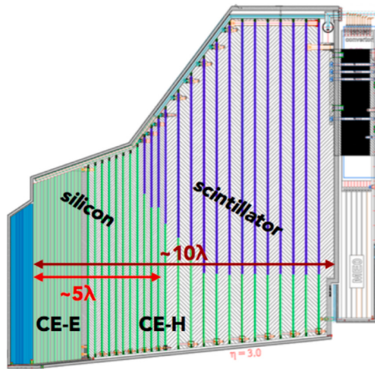
Fig. 3.6.4. Schematic drawing of the CMS HGCal design [165].
