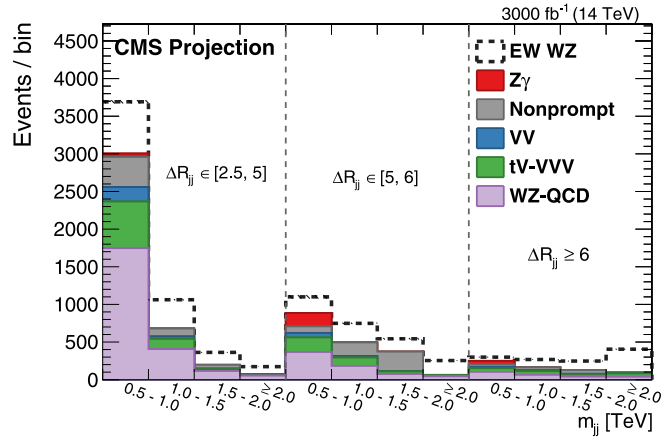
Fig. 3.1.1.3. Distribution of m_{jj} in bins of \Delta R_{jj} , i.e. the distance (in the \eta, \phi space) between jets. Source: From Ref. [107].
