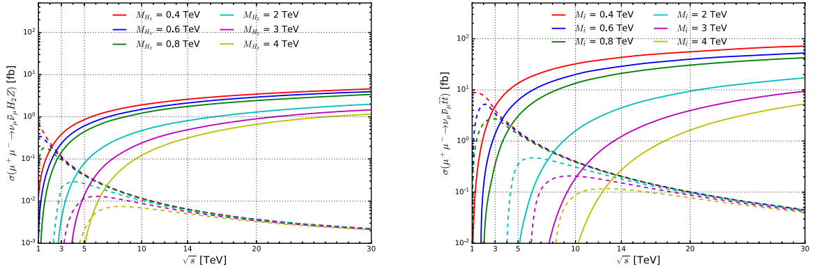
Fig. 4.5.1. Cross section [fb] via VBF (solid lines) and s -channel annihilation (dashed lines) for H_2Z associated production in the 2HDM (left) and \tau\tau pair production in the MSSM (right).
