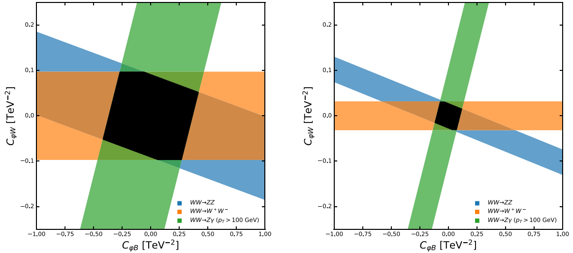
Fig. 4.4.3. Projections for the limits imposed on the Wilson coefficients C of the operators \mathcal{O}_{\varphi B} and \mathcal{O}_{\varphi W} at a future muon collider at 3 TeV (Left) and 14 TeV (Right).
