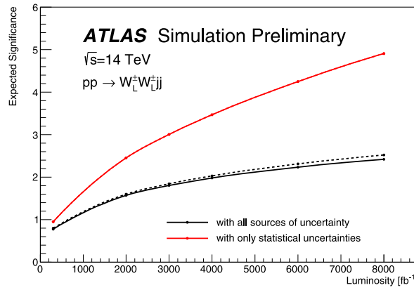
Fig. 3.1.7. Projection of the expected significance of the W^\pm W^\pm jj scattering process as function of integrated luminosity, considering all sources of uncertainty (black) or only the statistical uncertainty (red). The dashed line show the expectation for the optimistic scenario [109]. (For interpretation of the references to color in this figure legend, the reader is referred to the web version of this article.)
