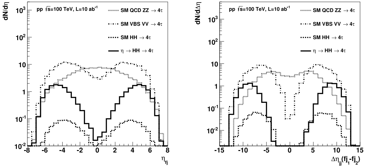
Fig. 4.6.1. Left: The pseudo-rapidity distributions of the forward jets. Right: The distribution of the difference in pseudo-rapidity of the two forward jets. Source: Figures are reproduced from Ref. [337].
