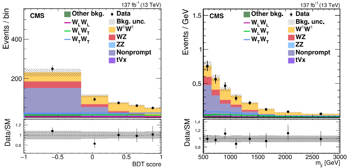
Fig. 2.1.2. Left : The distribution of the BDT discriminant used to extract the signal strength for the polarized components of the WW cross section. Right : Dijet invariant mass distribution.
