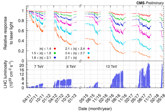
Fig. 3.6.3. Upper panel: relative ECAL response as a function of time at different \eta regions as monitored by laser calibrations since 2011. Lower panel: corresponding LHC luminosity.
