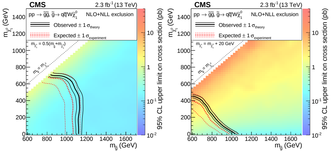
Figure 7: Exclusion regions at the 95% CL in the plane of m_{\tilde{\chi}_1^0} versus m_{\tilde{g}} for the T5qqqqWW model with m_{\tilde{\chi}_1^\pm} = 0.5(m_{\tilde{g}} + m_{\tilde{\chi}_1^0}) (left) and with m_{\tilde{\chi}_1^\pm} = m_{\tilde{\chi}_1^0} + 20 GeV (right). For a description of the notation, see Fig. 4.
