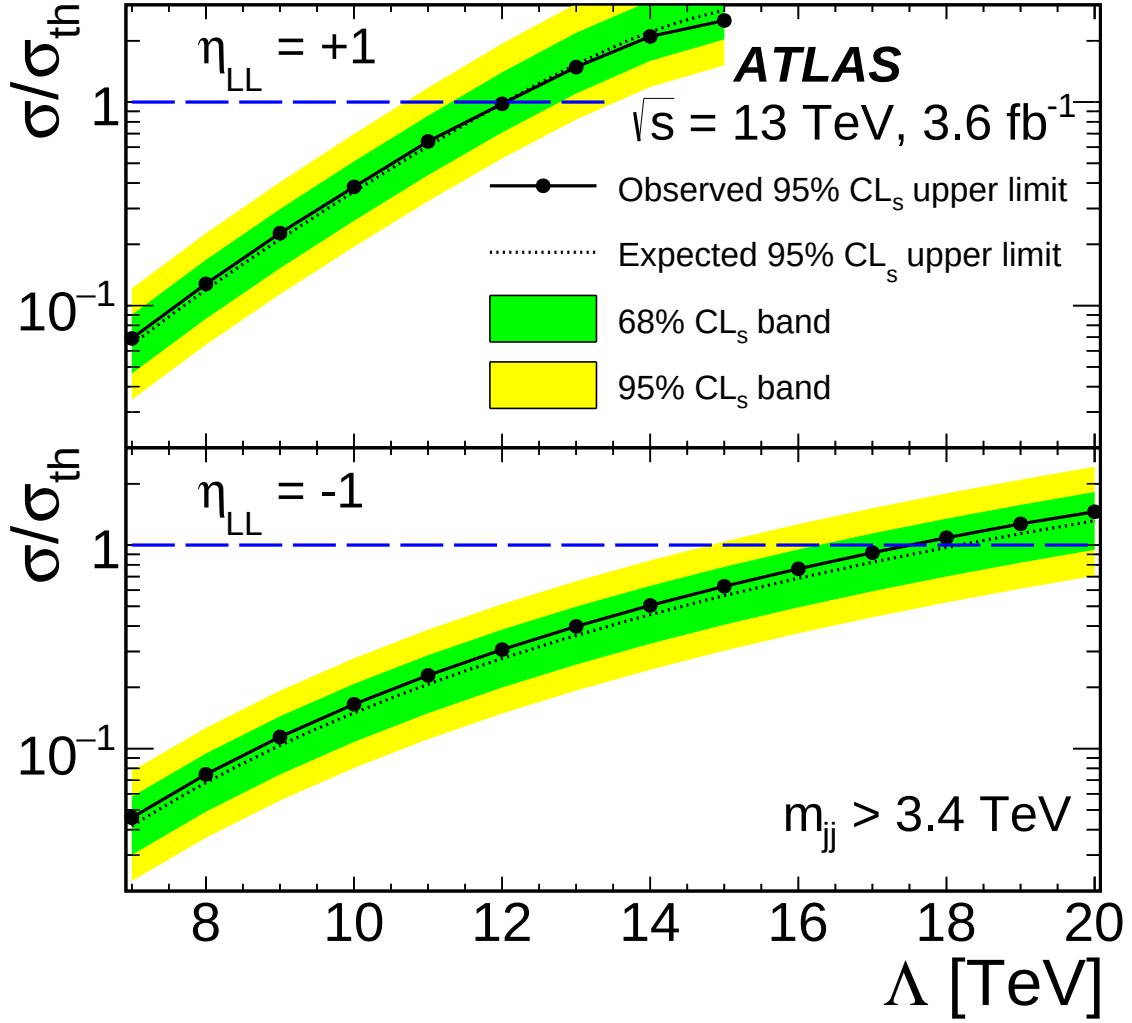
Figure 6: Ratio of the observed and expected 95% confidence-level upper limits on the cross-section in the contact interaction model to the predicted cross-section \sigma/\sigma_{th} as a function of compositeness scale \Lambda , for (top) destructive and (bottom) constructive interference with QCD processes. The crossing of the observed and expected 95% confidence-level lines with the line at signal strength of one indicates observed and expected lower limits on \Lambda , respectively.
