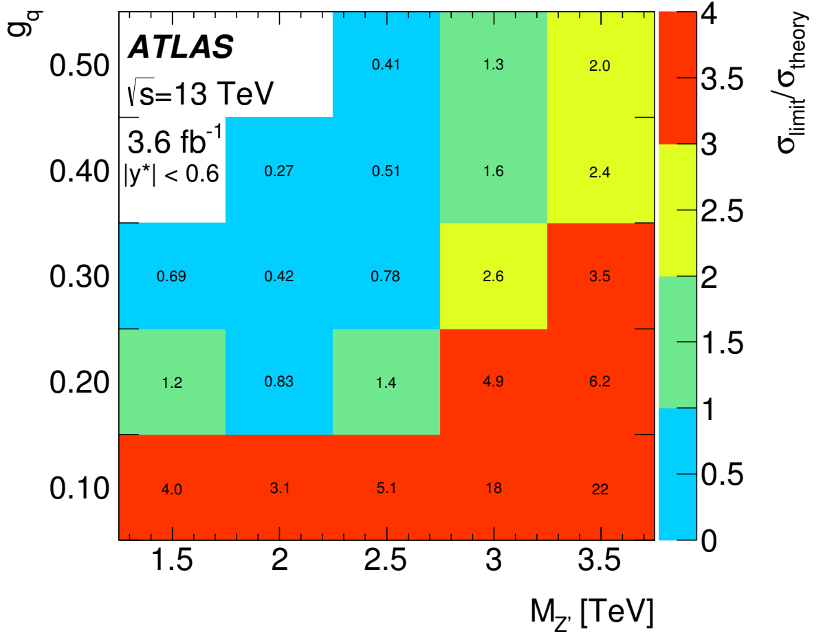
Figure 4: The ratio of 95% credibility-level upper limits to predicted cross-sections with respect to the Z' model predictions described in the text, as a function of the coupling to quarks, g_q , and the mass, M_{Z'} , obtained from the m_{jj} distribution. Since for a given mass higher couplings have higher cross sections and would therefore be excluded if lower couplings are excluded, the limits are not calculated in the white area.
