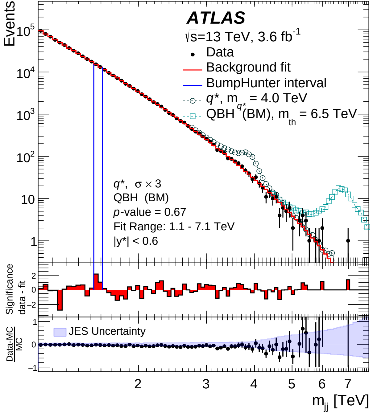
Figure 1: The reconstructed dijet mass distribution (filled points) for events with |y^*| < 0.6 and p_T > 440 (50) GeV for the leading (subleading) jets. The solid line depicts the fit to Eq. (1), as discussed in the text. Predictions for an excited quark and a quantum black hole signal predicted by the BLACKMAX generator (QBH BM) are shown above the fit, normalized to the predicted cross-section. The vertical lines indicate the most discrepant interval identified by the BUMP HUNTER algorithm, for which the p -value is stated in the figure. The middle panel shows the bin-by-bin significances of the data–fit differences, considering only statistical uncertainties. The lower panel shows the relative differences between the data and the prediction of PYTHIA 8 simulation of QCD processes, corrected for NLO and electroweak effects, and is shown purely for comparison. The shaded band denotes the experimental uncertainty in the jet energy scale calibration.
