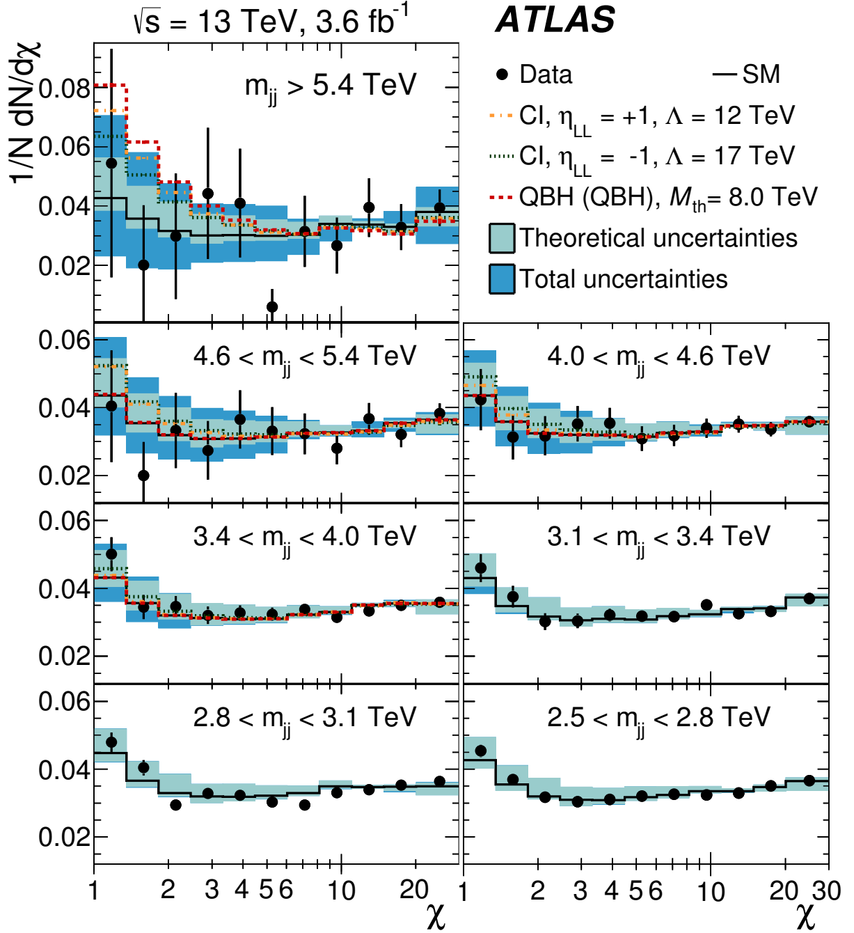
Figure 2: Reconstructed distributions of the dijet angular variable \chi in different regions of the dijet invariant mass m_{jj} for events with |y^*| < 1.7 , |y_B| < 1.1 and p_T > 440 (50) GeV for the leading (subleading) jets. Shown are the data (points), corrected NLO predictions (solid lines), and examples of the contact interaction (CI) and quantum black hole (QBH) signals discussed in the text. The theoretical uncertainties and the total theoretical and experimental uncertainties in the predictions are displayed as shaded bands around the SM prediction.
