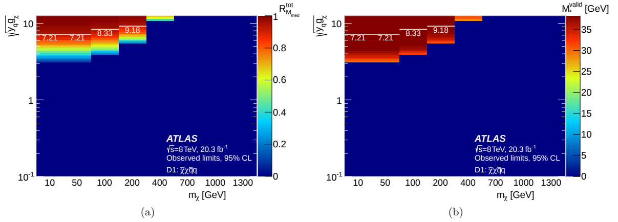
Fig. 17 (a) The fraction of valid events and (b) truncated limits for D1 at 95% CL as a function of the WIMP mass m_\chi and couplings. The white numbers correspond to the minimum coupling value for which M_*^{\text{valid}}/M_*^{\text{exp}} > 99\% . The upper perturbative coupling limit for D1 is 4\pi .
