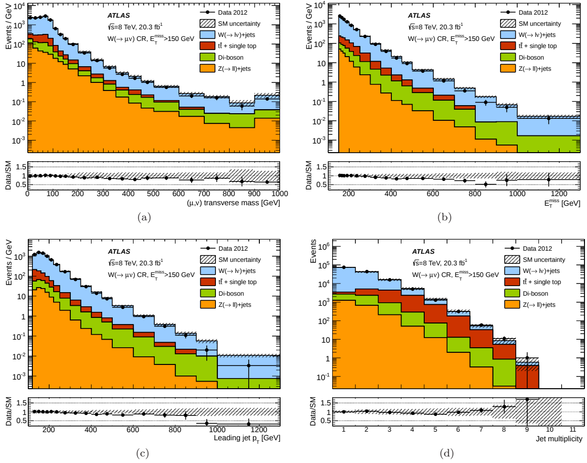
Fig. 2 Distributions of the measured (a) transverse mass of the identified muon and the missing transverse momentum, (b) E_T^{\text{miss}} , (c) leading jet p_T and (d) jet multiplicity distributions in the W(\rightarrow \mu\nu) +jets control region for the inclusive SR1 selection, compared to the background expectations. The latter include the global normalization factors extracted from the data. Where appropriate, the last bin of the distribution includes overflows. The lower panels represent the ratio of data to MC expectations. The error bands in the ratios include the statistical and experimental uncertainties on the background expectations.
