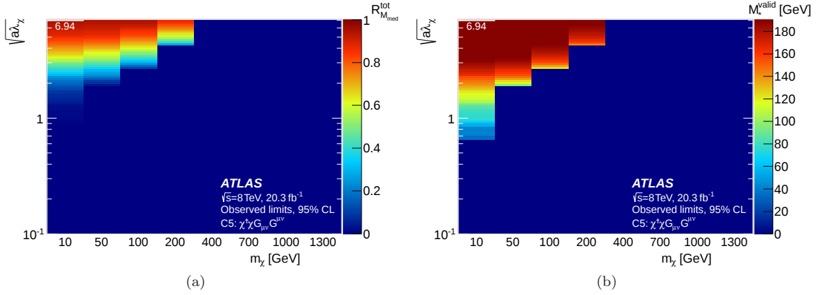
Fig. 21 (a) The fraction of valid events and (b) truncated limits for C5 at 95% CL as a function of the WIMP mass m_\chi and couplings. The white numbers correspond to the minimum coupling value for which M_*^{\text{valid}}/M_*^{\text{exp}} > 99\% . The upper perturbative coupling limit for C5 is 4\sqrt{\pi\zeta_\lambda} , where \zeta_\lambda is taken to be 1.
