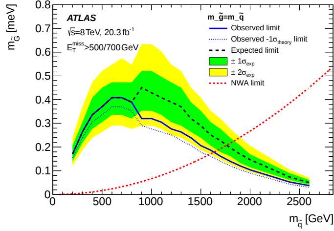
Fig. 14 Observed (solid line) and expected (dashed line) 95% CL lower limits on the gravitino mass m_{\tilde{G}} as a function of the squark mass m_{\tilde{q}} for degenerate squark/gluino masses. The corresponding dotted line indicates the impact on the observed limit of the -1\sigma LO theoretical uncertainty. The shaded bands around the expected limit indicate the expected \pm 1\sigma and \pm 2\sigma ranges of limits in the absence of a signal. The region above the red dotted line defines the validity of the narrow-width approximation (NWA) for which the decay width is smaller than 25% of the squark/gluino mass.
