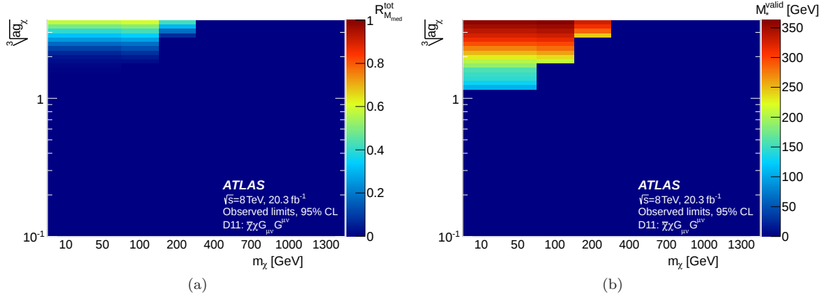
Fig. 20 (a) The fraction of valid events and (b) truncated limits for D11 at 95% CL as a function of the WIMP mass m_\chi and couplings. The white numbers correspond to the minimum coupling value for which M_*^{\text{valid}}/M_*^{\text{exp}} > 99\% . The upper perturbative coupling limit for D11 is \sqrt[3]{16\pi} .
