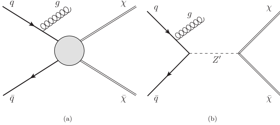
Fig. 1 Feynman diagrams for the production of weakly interacting massive particle pairs \chi\bar{\chi} associated with a jet from initial-state radiation of a gluon, g . (a) A contact interaction described with effective operators. (b) A simplified model with a Z' boson.
