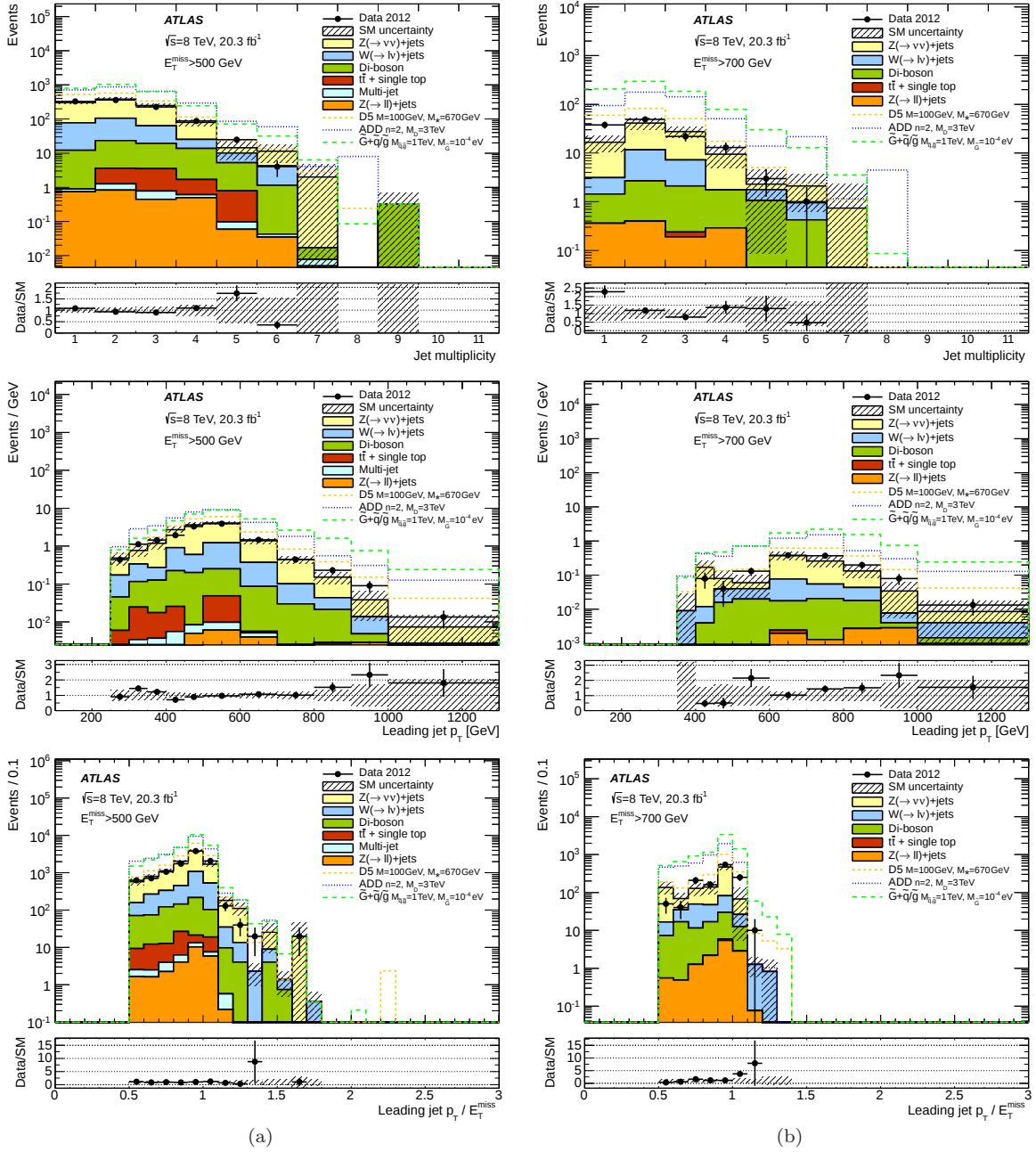
Fig. 7 Measured distributions of the jet multiplicity, leading jet p_T , and the leading jet p_T to E_T^{\text{miss}} ratio for (a) SR7 and (b) SR9 selections compared to the SM expectations. The Z(\rightarrow \nu\bar{\nu}) +jets control sample is shown as constrained by the W(\rightarrow \mu\nu) +jets control sample. Where appropriate, the last bin of the distribution includes overflows. For illustration purposes, the distribution of different ADD, WIMP and GMSB scenarios are included. The error bands in the ratios shown in lower panels include both the statistical and systematic uncertainties on the background expectations.
