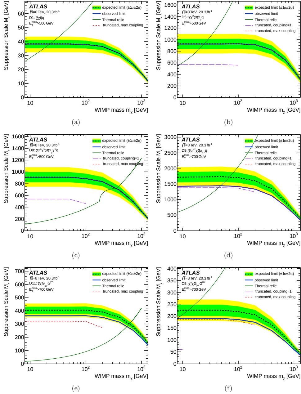
Fig. 10 Lower limits at 95% CL on the suppression scale M_* are shown as a function of the WIMP mass m_\chi for (a) D1, (b) D5, (c) D8, (d) D9, (e) D11 and (f) C5 operators, in each case for the most sensitive SR (SR7 for D1, D5, D8, SR9 for D9, D11 and C5). The expected and observed limits are shown as dashed black and solid blue lines, respectively. The rising green lines are the M_* values at which WIMPs of the given mass result in the relic density as measured by WMAP [26], assuming annihilation in the early universe proceeded exclusively via the given operator. The purple long-dashed line is the 95% CL observed limit on M_* imposing a validity criterion with a coupling strength of 1, the red dashed thin lines are those for the maximum physical coupling strength (see Appendix A for further details).
