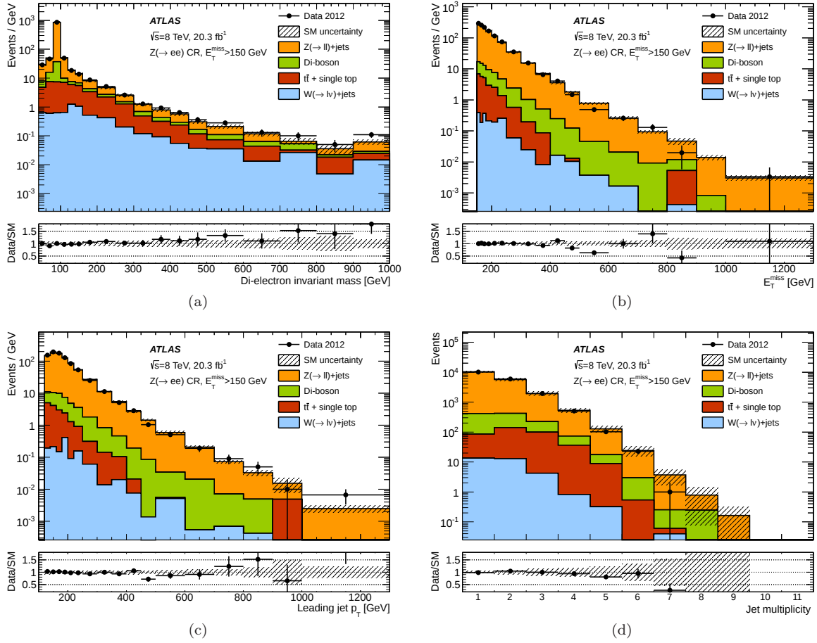
Fig. 5 Distributions of the measured (a) dilepton invariant mass, (b) E_T^{\text{miss}} , (c) leading jet p_T and (d) jet multiplicity distributions in the Z/\gamma^*(\rightarrow e^+e^-)+\text{jets} control region for the inclusive SR1 selection, compared to the background expectations. The latter include the global normalization factors extracted from the data. Where appropriate, the last bin of the distribution includes overflows. The lower panels represent the ratio of data to MC expectations. The error bands in the ratios include the statistical and experimental uncertainties on the background expectations.
