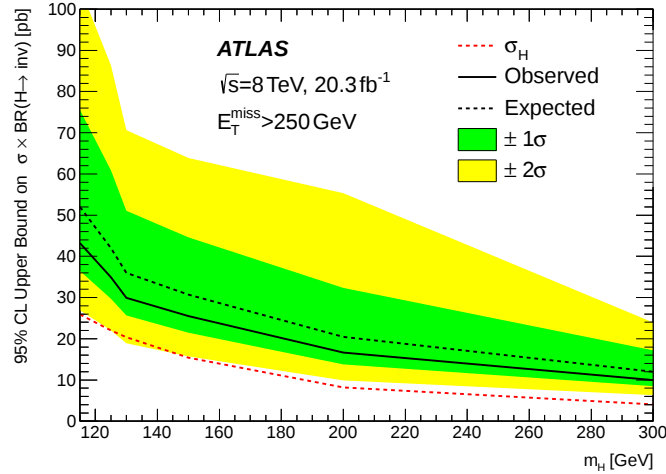
Fig. 16 The observed (solid line) and expected (dashed line) 95% CL upper limit on \sigma \times \text{BR}(H \rightarrow \text{invisible}) as a function of the boson mass m_H . The shaded areas around the expected limit indicate the expected \pm 1\sigma and \pm 2\sigma ranges of limits in the absence of a signal. The expectation for a Higgs boson with \text{BR}(H \rightarrow \text{invisible}) = 1 , \sigma_H , is also shown.
