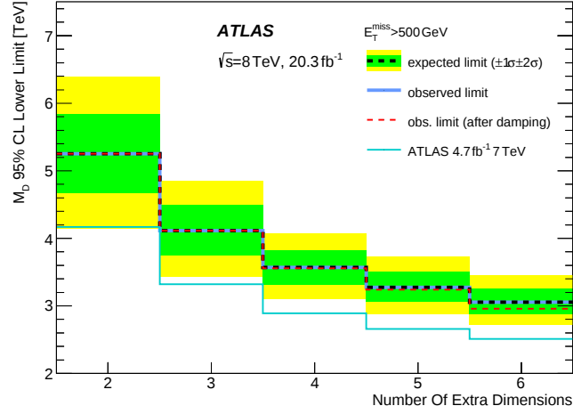
Fig. 9 Observed and expected 95% CL limit on the fundamental Planck scale in 4 + n dimensions, M_D , as a function of the number of extra dimensions. In the figure the two results overlap. The shaded areas around the expected limit indicate the expected \pm 1\sigma and \pm 2\sigma ranges of limits in the absence of a signal. Finally, the thin dashed line shows the 95% CL observed limits after the suppression of the events with \hat{s} > M_D^2 (damping) is applied, as described in the body of the text. The results from this analysis are compared to previous results from ATLAS at 7 TeV [12] without any damping applied.
