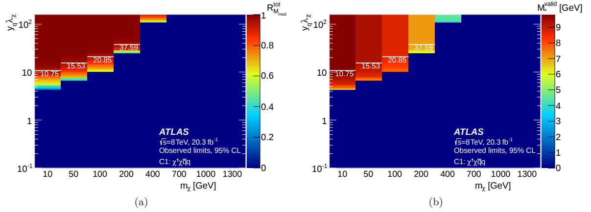
Fig. 18 (a) The fraction of valid events and (b) truncated limits for C1 at 95% CL as a function of the WIMP mass m_\chi and couplings. The white numbers correspond to the minimum coupling value for which M_*^{\text{valid}}/M_*^{\text{exp}} > 99\% . The upper perturbative coupling limit for C1 is (4\pi)^2 \zeta_\lambda , where \zeta_\lambda is taken to be 1.
