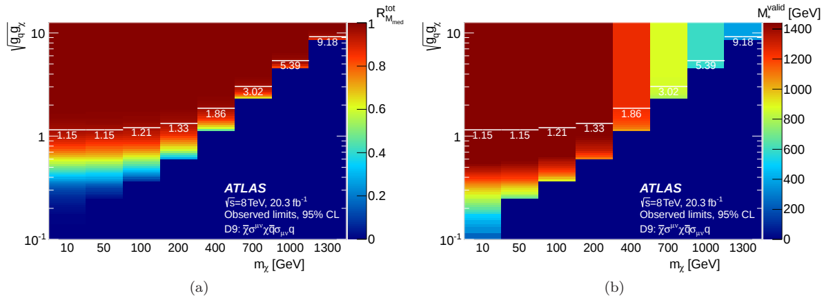
Fig. 19 (a) The fraction of valid events and (b) truncated limits for D9 at 95% CL as a function of the WIMP mass m_\chi and couplings. The white numbers correspond to the minimum coupling value for which M_*^{\text{valid}}/M_*^{\text{exp}} > 99\% . The upper perturbative coupling limit for D9 is 4\pi .
