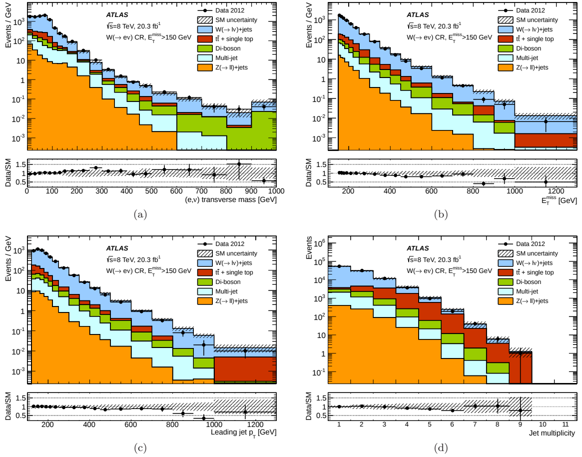
Fig. 4 Distributions of the measured (a) transverse mass of the identified electron and the missing transverse momentum, (b) E_T^{\text{miss}} , (c) leading jet p_T and (d) jet multiplicity distributions in the W(\rightarrow e\nu)+\text{jets} control region for the inclusive SR1 selection, compared to the background expectations. The latter include the global normalization factors extracted from the data. Where appropriate, the last bin of the distribution includes overflows. The lower panels represent the ratio of data to MC expectations. The error bands in the ratios include the statistical and experimental uncertainties on the background expectations.
