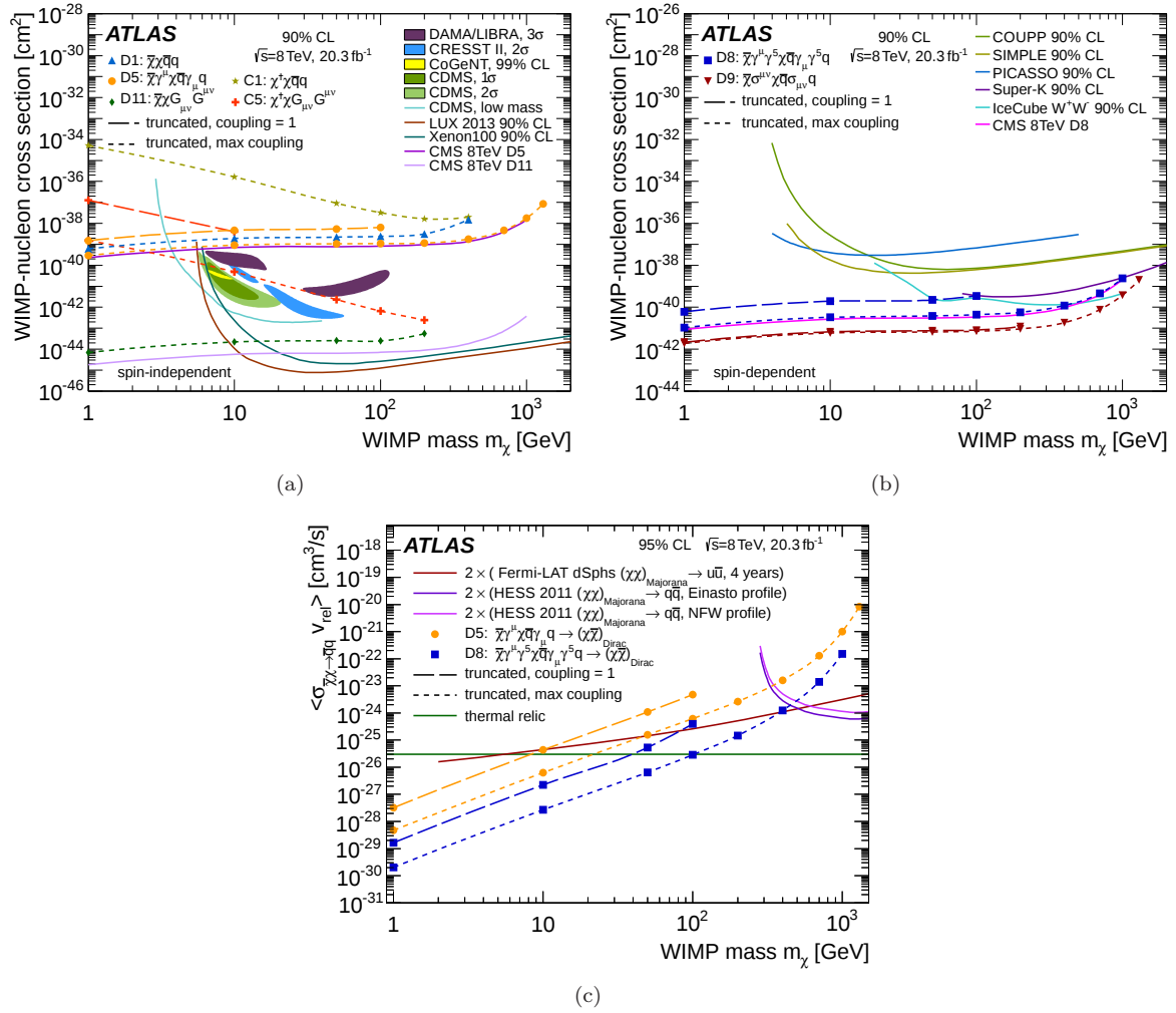
Fig. 12 Inferred 90% CL limits on (a) the spin-independent and (b) spin-dependent WIMP–nucleon scattering cross section as a function of DM mass m_\chi for different operators (see Sect. 1). Results from direct-detection experiments for the spin-independent [127–133] and spin-dependent [134–138] cross section, and the CMS (untruncated) results [14] are shown for comparison. (c) The inferred 95% CL limits on the DM annihilation rate as a function of DM mass. The annihilation rate is defined as the product of cross section \sigma and relative velocity v , averaged over the DM velocity distribution ( \langle \sigma v \rangle ). Results from gamma-ray telescopes [125, 126] are also shown, along with the thermal relic density annihilation rate [25, 26].
