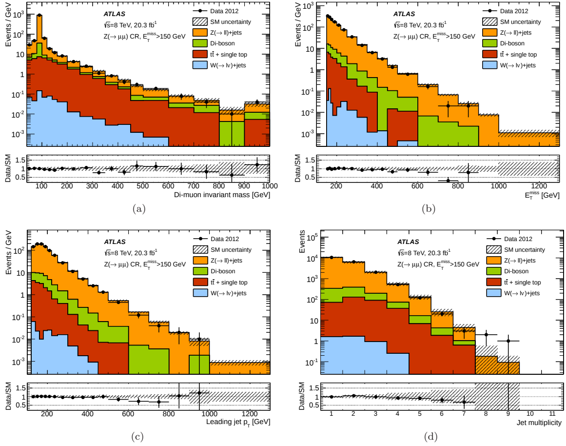
Fig. 3 Distributions of the measured (a) dilepton invariant mass, (b) E_T^{\text{miss}} , (c) leading jet p_T and (d) jet multiplicity distributions in the Z/\gamma^* \rightarrow \mu^+\mu^- + \text{jets} control region for the inclusive SR1 selection, compared to the background expectations. The latter include the global normalization factors extracted from the data. Where appropriate, the last bin of the distribution includes overflows. The lower panels represent the ratio of data to MC expectations. The error bands in the ratios include the statistical and experimental uncertainties on the background expectations.
