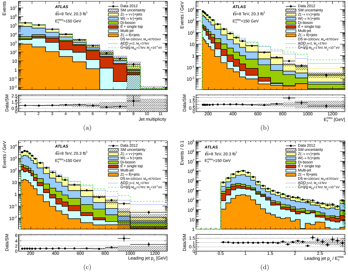
Fig. 6 Measured distributions of (a) the jet multiplicity, (b) E_T^{\text{miss}} , (c) leading jet p_T , and (d) the leading jet p_T to E_T^{\text{miss}} ratio for the SR1 selection compared to the SM expectations. The Z(\rightarrow \nu\bar{\nu}) +jets contribution is shown as constrained by the W(\rightarrow \mu\nu) +jets control sample. Where appropriate, the last bin of the distribution includes overflows. For illustration purposes, the distribution of different ADD, WIMP and GMSB scenarios are included. The error bands in the ratios shown in lower panels include both the statistical and systematic uncertainties on the background expectations.
