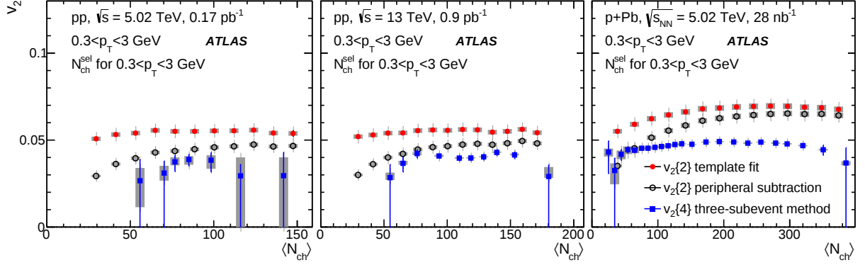
Figure 12: The v_2\{4\} values calculated for charged particles with 0.3 < p_T < 3 GeV using the three-subevent method in 5.02 TeV pp (left panel), 13 TeV pp (middle panel) and 5.02 TeV p +Pb collisions (right panel). They are compared to v_2 obtained from the 2PC analyses [10, 15] where the non-flow effects are removed by a template fit procedure (solid circles) or with a fit after subtraction with a ZYAM assumption (peripheral subtraction, open circles). The error bars and shaded boxes represent the statistical and systematic uncertainties, respectively.
