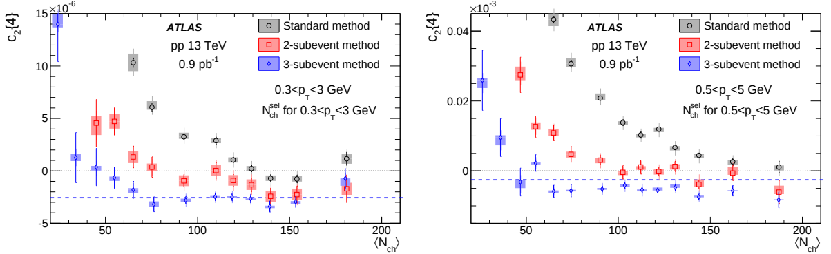
Figure 4: The c_2\{4\} values calculated for charged particles with 0.3 < p_T < 3 GeV (left panel) and 0.5 < p_T < 5 GeV (right panel) compared for the three cumulant methods from the 13 TeV pp data. The event averaging is performed for N_{\text{ch}}^{\text{sel}} calculated for the same p_T range, which is then mapped to \langle N_{\text{ch}} \rangle , the average number of charged particles with p_T > 0.4 GeV. The dashed line indicates the c_2\{4\} value corresponding to a 4% v_2 signal. The error bars and shaded boxes represent the statistical and systematic uncertainties, respectively.
