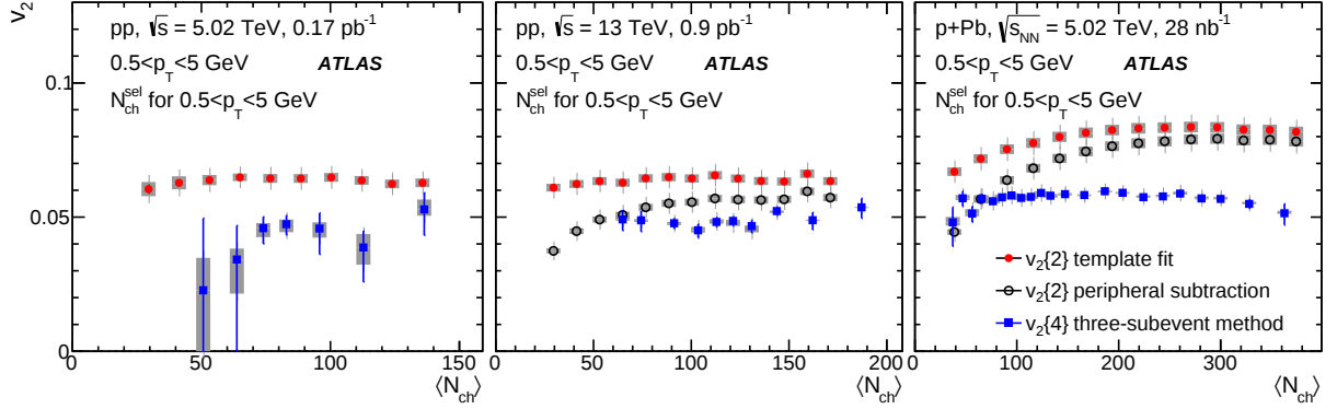
Figure 13: The v_2\{4\} values calculated for charged particles with 0.5 < p_T < 5 GeV using the three-subevent method in 5.02 TeV pp (left panel), 13 TeV pp (middle panel) and 5.02 TeV p +Pb collisions (right panel). They are compared to v_2 obtained from the 2PC analyses [10, 15] where the non-flow effects are removed by a template fit procedure (solid circles) or with a fit after subtraction with a ZYAM assumption (peripheral subtraction, open circles). The error bars and shaded boxes represent the statistical and systematic uncertainties, respectively.
