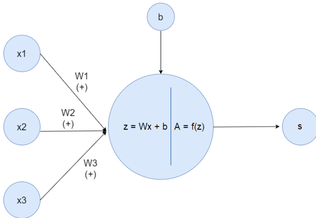
Figura 2.4: Neurona Artificial
