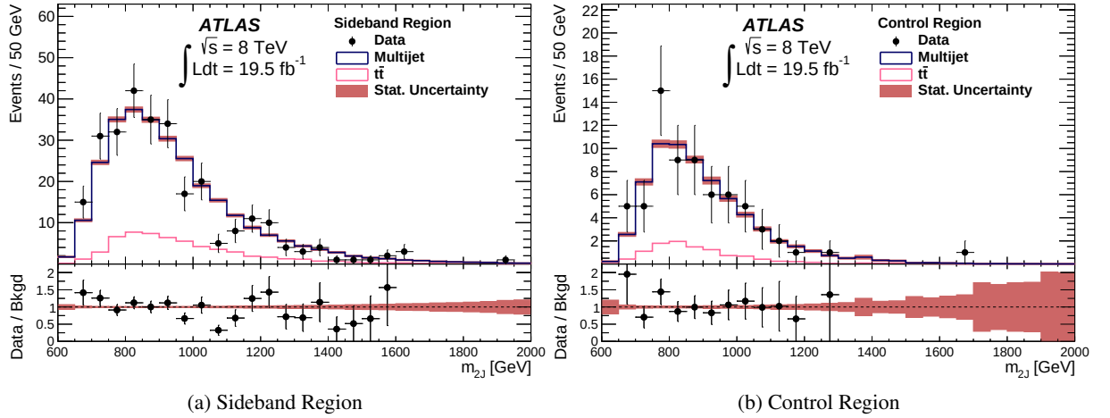
Figure 10: Dijet mass distributions for 4-tag events in the boosted analysis. (a) shows the sideband region and (b) the control region for data (points) and the expected background (histograms). The filled blocks represent the statistical uncertainty in the total background estimate.
