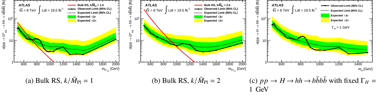
Figure 14: The combined expected and observed limit for pp \rightarrow G_{KK}^* \rightarrow hh \rightarrow b\bar{b}b\bar{b} in the bulk RS model with (a) k/\bar{M}_{Pl} = 1 and (b) k/\bar{M}_{Pl} = 2 , as well as (c) pp \rightarrow H \rightarrow hh \rightarrow b\bar{b}b\bar{b} with fixed \Gamma_H = 1 GeV. The red curves show the predicted cross-sections as a function of resonance mass for the models considered.
