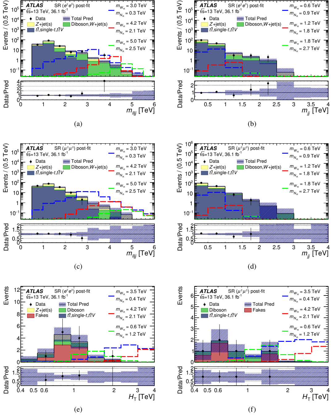
Figure 6: Distributions for data and background predictions for discriminant variables in various signal regions and channels: (a) m_{\ell\ell jj} in \text{SR}(e^+e^-) , (b) m_{jj} in \text{SR}(e^+e^-) , (c) m_{\ell\ell jj} in \text{SR}(\mu^+\mu^-) , (d) m_{jj} in \text{SR}(\mu^+\mu^-) , (e) H_T in \text{SR}(e^+e^-) , and (f) H_T in \text{SR}(\mu^+\mu^-) . The hatched bands include all post-fit systematic uncertainties. The correlation between sources of systematic uncertainties are taken into account. A few simulated signal distributions, normalised to the predicted cross-section, are overlaid on top of the background prediction in the plots. The last bin in each histogram contains the overflow.
