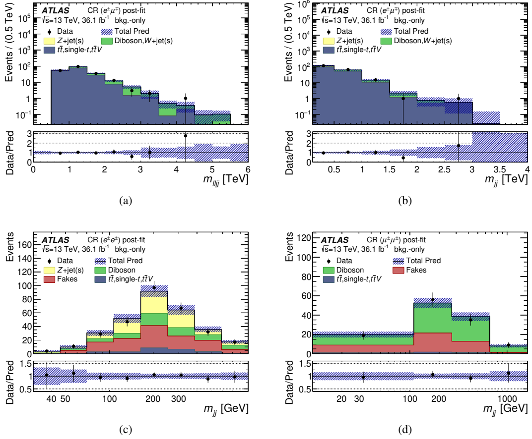
Figure 4: Distributions for data and background predictions for discriminant variables in various control regions and channels after the background-only fit: (a) m_{\ell\ell jj} in CR( e^+\mu^+ ), (b) m_{jj} in CR( e^+\mu^+ ), (c) m_{jj} in CR( e^+e^+ ), and (d) m_{jj} in CR( \mu^+\mu^+ ). The hatched bands include all post-fit systematic uncertainties. The correlation between sources of systematic uncertainties are taken into account. The last bin in each histogram contains the overflow.
