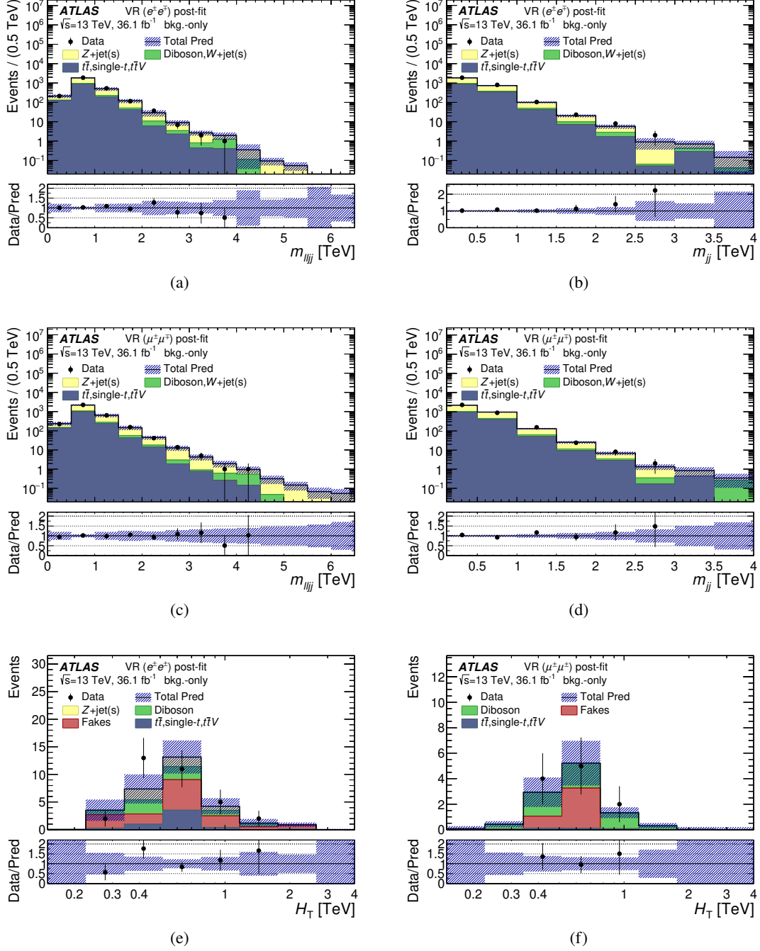
Figure 5: Distributions for data and background predictions for discriminant variables in various validation regions and channels after the background-only fit: (a) m_{\ell\ell jj} in VR( e^\pm e^\pm ), (b) m_{jj} in VR( e^\pm e^\pm ), (c) m_{\ell\ell jj} in VR( \mu^\pm \mu^\pm ), (d) m_{jj} in VR( \mu^\pm \mu^\pm ), (e) H_T in VR( e^\pm e^\pm ), and (f) H_T in VR( \mu^\pm \mu^\pm ). The hatched bands include all post-fit systematic uncertainties. The correlation between sources of systematic uncertainties are taken into account. The last bin in each histogram contains the overflow.
