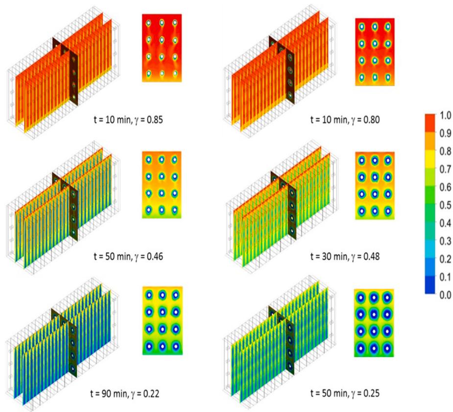
Fig. 8. Liquid mass fraction distribution at three stages of the solidification process (left: case A1; right: case A3).
