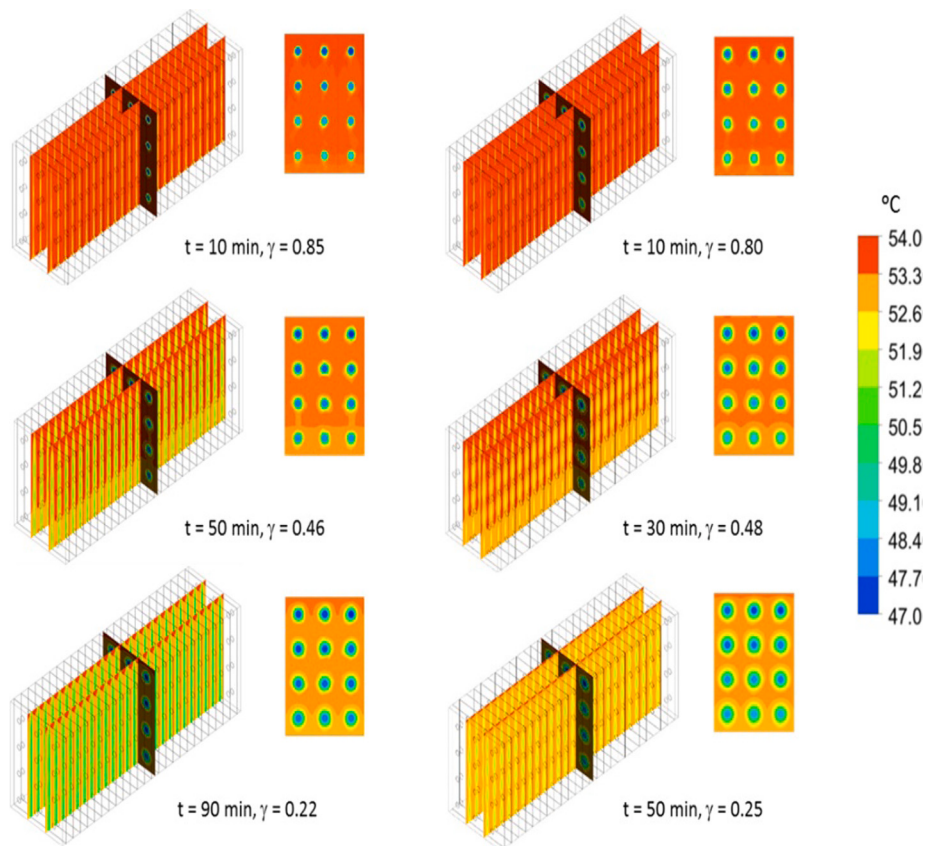
Fig. 7. Temperature distribution at three stages of the solidification process (left: case A1; right: case A3).
