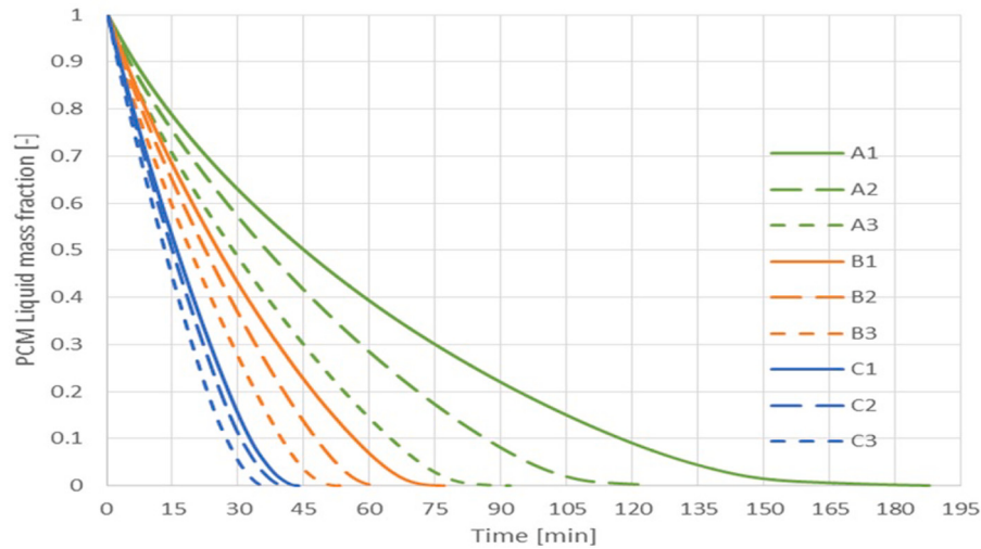
Fig. 11. Liquid fraction history.
