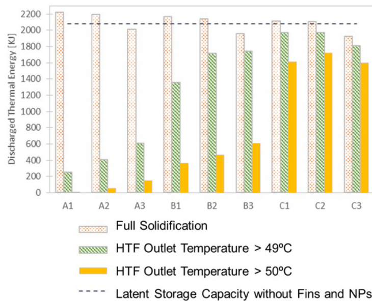
Fig. 13. Thermal energy discharge capacity at different stages of solidification.
