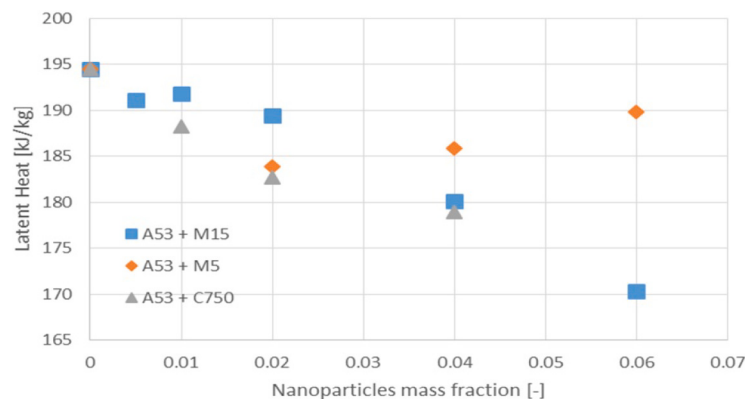
Fig. 2. Fusion latent heat of pure A53 and A53 NePCMs vs. nanoparticles mass fraction.
