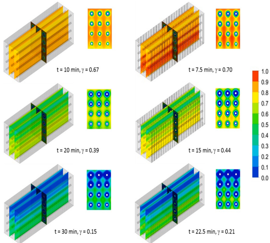
Fig. 10. Liquid mass fraction distribution at three stages of the solidification process (left: case C1; right: case C3).
