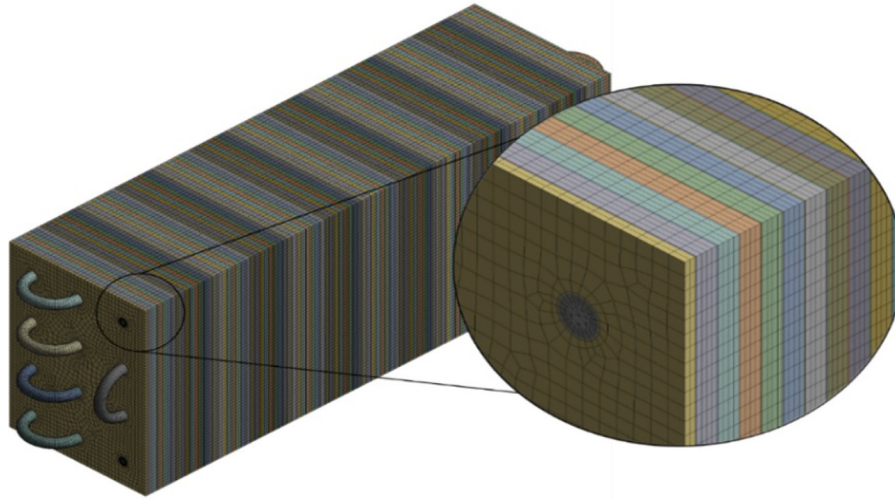
Fig. 5. Mesh and computational domain of the 5 mm fin pitch geometry.
