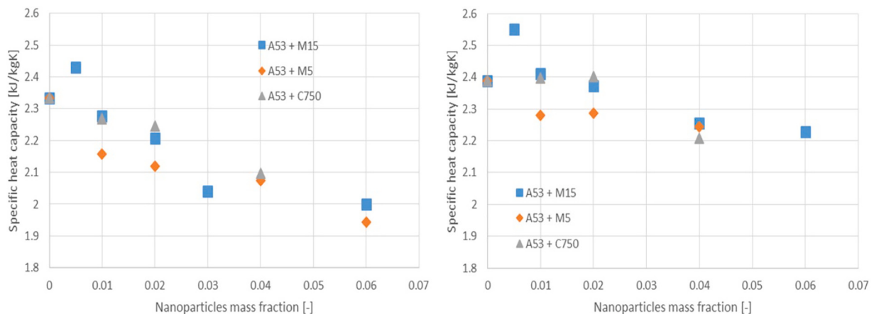
Fig. 3. Specific heat capacity of pure A53 and A53 NePCMs vs. nanoparticles mass fraction.
