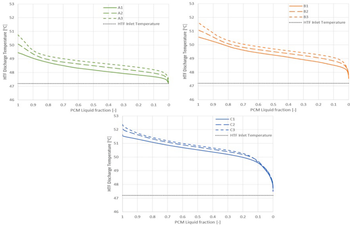
Fig. 12. HTF outlet temperature over solidification.
