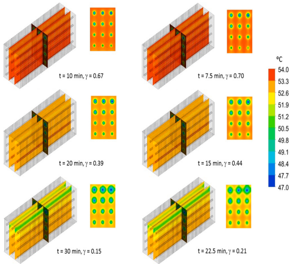
Fig. 9. Temperature distribution at three stages of the solidification process (left: case C1; right: case C3).
