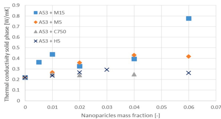
Fig. 1. Thermal conductivity of pure A53 and A53 NePCMs vs. nanoparticles mass fraction.
