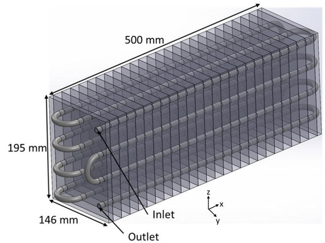
Fig. 4. LHTES simulated geometry.
