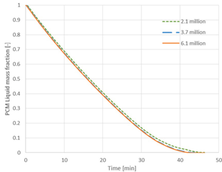
Fig. 6. Mesh independent study at 0.25 s time step (case C1).
