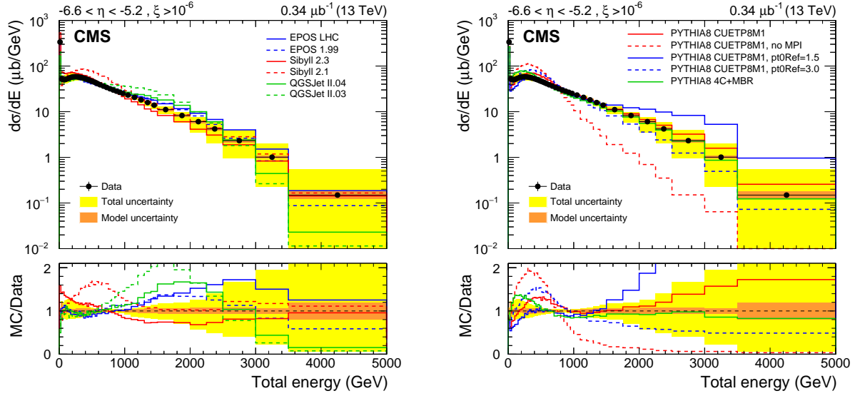
Figure 3: Differential cross section as a function of the total energy in the region -6.6 < \eta < -5.2 for events with \xi > 10^{-6} . The left panel shows the data compared to MC event generators mostly developed for cosmic ray induced air showers, and the right panel to different PYTHIA 8 tunes.
