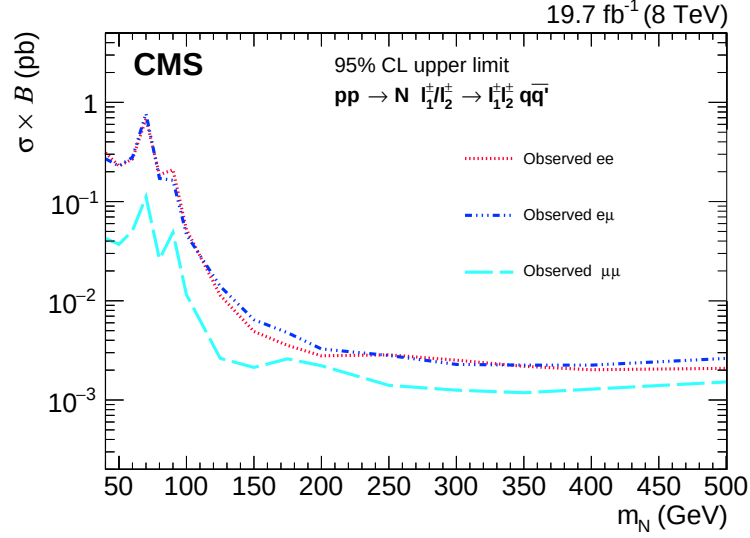
Figure 6: Comparison of observed exclusion regions at 95% CL in the cross section times branching fraction as a function of m_N for pp \rightarrow N e^\pm \rightarrow e^\pm e^\pm q\bar{q}' , pp \rightarrow N \mu^\pm \rightarrow \mu^\pm \mu^\pm q\bar{q}' , and pp \rightarrow N e^\pm/\mu^\pm \rightarrow e^\pm \mu^\pm q\bar{q}' . The result for the dimuon channel is from Ref. [30].
