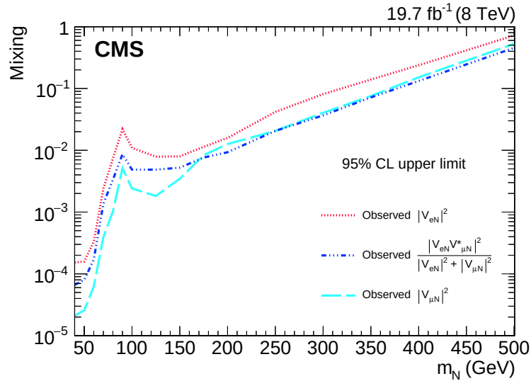
Figure 7: Comparison of observed exclusion regions at 95% CL in |V_{\mu N}|^2 , |V_{eN}|^2 , and |V_{eN}V_{\mu N}^*|^2/(|V_{eN}|^2 + |V_{\mu N}|^2) . The CMS result for |V_{\mu N}|^2 is from Ref. [30].
