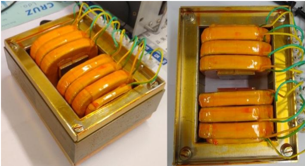
Fig. 5. Specially developed electromagnet for a NMR FFC spectrometer: 4.5 cm height built of iron standard E shaped transformer plates 13.5 cm width, 1.5 cm gap in the middle foot, six coils with 218 turns each, maximum current of 3 A and maximum achievable magnetic field of 0.328 T.
