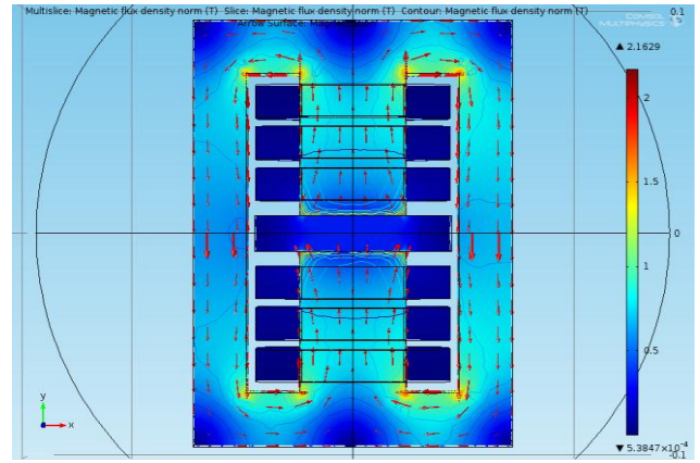
Fig. 4. Top view of magnetic field plots: Volume and Arrow line. Designed in COMSOL Multiphysics® 4.3.
