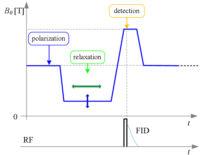
Fig. 2. Typical cycle of the main magnetic field B_0 [2].
