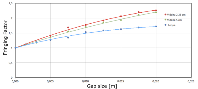
Fig. 6. Fringing ratio vs. gap size for the current case (2.25 cm distance between feet), the 5 cm feet distance, and the previously built electromagnet ( b=18 cm with 3 cm distance between feet).
