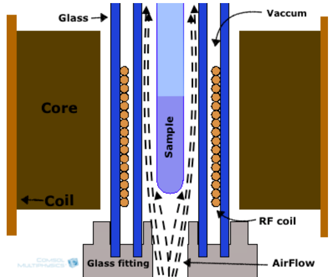
Fig. 7. Close up of the heating system.
