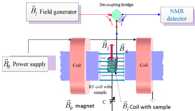
Fig. 1. Standard NMR spectrometer.
