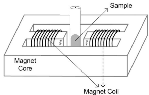
Fig. 3. Magnetic electromagnet with coils around the middle feet [9].
