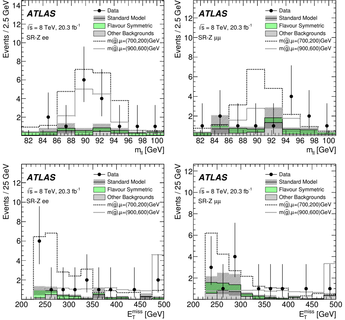
Figure 6: The dilepton mass (top) and E_T^{\text{miss}} (bottom) distributions for the electron (left) and muon (right) channel in the on-Z SRs after having applied the requirement \Delta\phi(\text{jet}_{1,2}, E_T^{\text{miss}}) > 0.4 . All uncertainties are included in the hatched uncertainty band. Two example GGM ( \tan\beta = 1.5 ) signal models are overlaid. For the E_T^{\text{miss}} distributions, the last bin contains the overflow. The backgrounds due to WZ , ZZ or rare top processes, as well as from fake leptons, are included under “Other Backgrounds”. The negligible contribution from Z +jets is omitted from these distributions.
