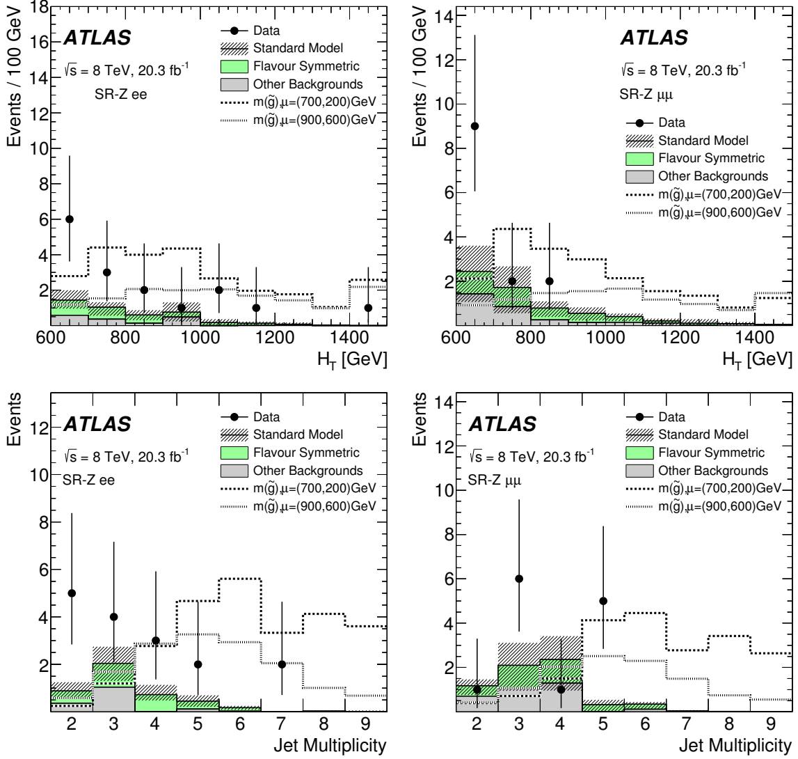
Figure 7: The H_T (top) and jet multiplicity (bottom) distributions for the electron (left) and muon (right) channel in the on-Z SRs after having applied the requirement \Delta\phi(\text{jet}_{1,2}, E_T^{\text{miss}}) > 0.4 . All uncertainties are included in the hatched uncertainty band. Two example GGM ( \tan\beta = 1.5 ) signal models are overlaid. For the H_T distributions, the last bin contains the overflow. The backgrounds due to WZ , ZZ or rare top processes, as well as from fake leptons, are included under “Other Backgrounds”. The negligible contribution from Z +jets is omitted from these distributions.
