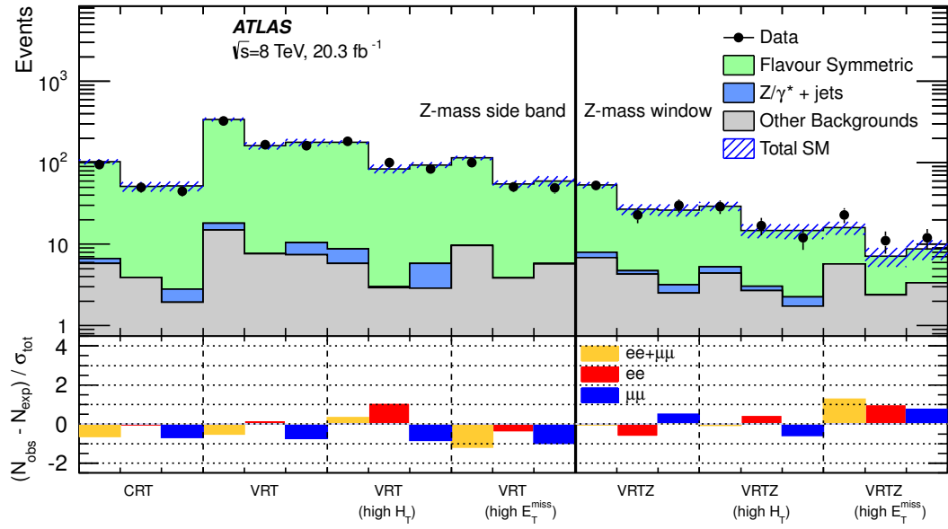
Figure 4: The observed and expected yields in CRT and the VRs in the Z boson mass sidebands (left) and the Z boson mass window (right) regions. The bottom plot shows the difference in standard deviations between the observed and expected yields. The backgrounds due to WZ , ZZ or rare top processes, as well as from lepton fakes, are included under “Other Backgrounds”.
