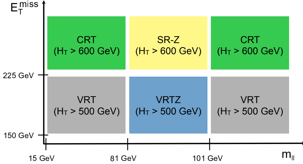
Figure 3: Diagram indicating the position in the E_T^{\text{miss}} versus dilepton invariant mass plane of SR-Z, the control region CRT, and the two validation regions (VRT and VRTZ) used to validate the sideband fit for the on-Z search. VRT and VRTZ have lower H_T thresholds than CRT and SR-Z.
