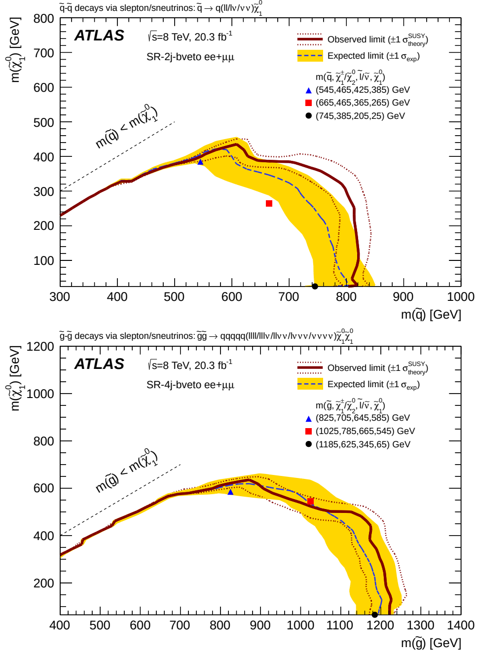
Figure 13: Excluded region in the (top) squark–LSP mass plane using the SR-2j-bveto results and (bottom) gluino–LSP mass plane using the SR-4j-bveto results. The observed, expected, and \pm 1\sigma expected exclusion contours are indicated. The observed limits obtained upon varying the signal cross section by \pm 1\sigma are also indicated. The region to the left of the diagonal dashed line has the squark mass less than the LSP mass and is hence not considered. Three signal benchmark points are shown, with their SUSY particle masses indicated in parentheses.
