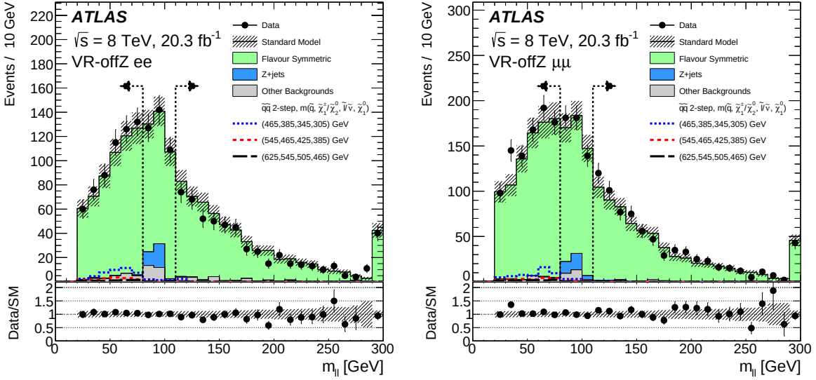
Figure 5: The observed and expected dilepton mass distributions in the electron (left) and muon (right) channel of the validation region (VR-offZ) of the off-Z search. Data (black points) are compared to the sum of expected backgrounds (solid histograms). The vertical dashed lines indicate the 80 < m_{\ell\ell} < 110 GeV region, which is used to normalise the Z + jets background. Example signal models (dashed lines) are overlaid, with m(\tilde{q}) , m(\tilde{\chi}_2^0)/m(\tilde{\chi}_1^{\pm}) , m(\tilde{\ell})/m(\tilde{\nu}) , and m(\tilde{\chi}_1^0) of each benchmark point being indicated in the figure legend. The bottom plots show the ratio of the data to expected background. The error bars indicate the statistical uncertainty in data, while the shaded band indicates the total background uncertainty. The last bin contains the overflow.
