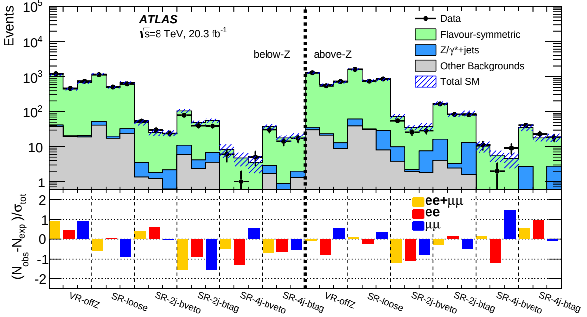
Figure 11: The observed and expected yields in the below-Z (left) and above-Z (right) dilepton mass regions, for the VR and five SRs of the off-Z search. Here below-Z is 20 < m_{\ell\ell} < 70 GeV for VR-offZ and SR-loose and otherwise 20 < m_{\ell\ell} < 80 GeV; above-Z is m_{\ell\ell} > 110 GeV. The bottom plot shows the difference in standard deviations between the observed and expected yields. Results are shown for the ee and \mu\mu channels as well as for the sum.
