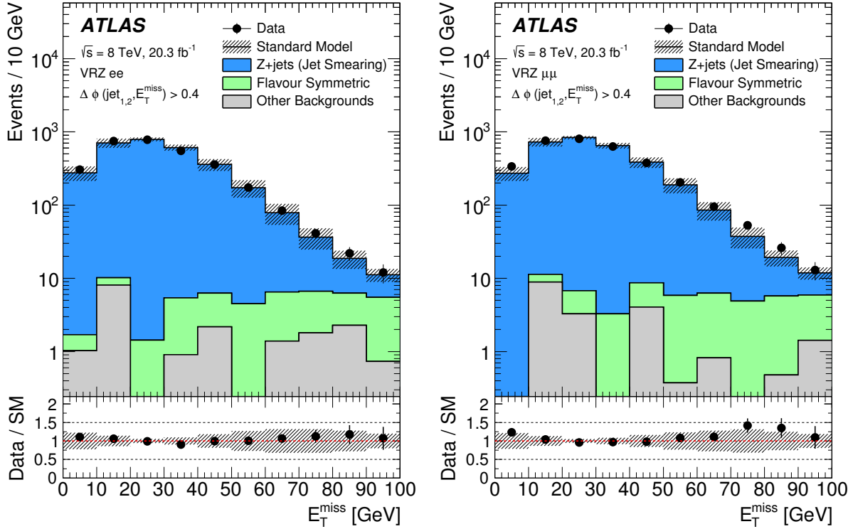
Figure 2: Distribution of E_T^{\text{miss}} in the electron (left) and muon (right) channel in VRZ of the on-Z analysis following the requirement of \Delta\phi(\text{jet}_{1,2}, E_T^{\text{miss}}) > 0.4 . Here the Z/\gamma^* + \text{jets} background (solid blue) is modelled using p_T - and \phi -smeared pseudo-data events. The hatched uncertainty band includes the statistical uncertainty on the simulated event samples and the systematic uncertainty on the jet-smearing estimate due to the jet response function and the seed selection. The backgrounds due to WZ , ZZ or rare top processes, as well as from lepton fakes, are included under “Other Backgrounds”.
