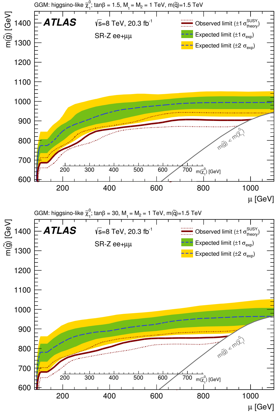
Figure 12: The 95 % CL exclusion limit from the on-Z combined same-flavour channels in the \mu versus m(\tilde{g}) plane in the GGM model with \tan\beta = 1.5 (top) and \tan\beta = 30 (bottom). The dark blue dashed line indicates the expected limits at 95 % CL and the green (yellow) bands show the \pm 1\sigma ( \pm 2\sigma ) variation on the expected limit as a consequence of the experimental and theoretical uncertainties on the background prediction. The observed limits are shown by the solid red lines, with the dotted red lines indicating the limit obtained upon varying the signal cross section by \pm 1\sigma . The region below the grey line has the gluino mass less than the lightest neutralino mass and is hence not considered. The value of the lightest neutralino mass is indicated by the x -axis inset.
