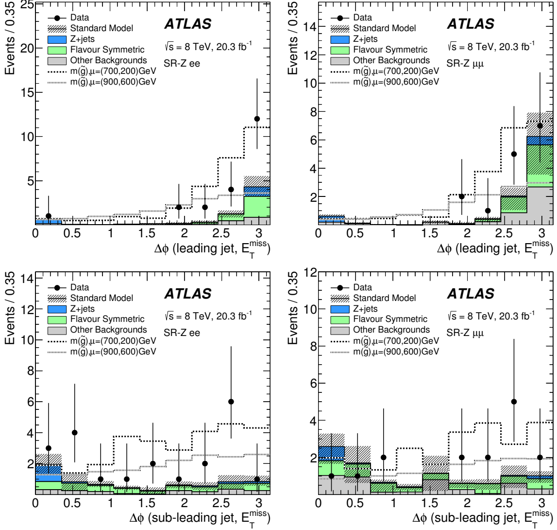
Figure 8: The distribution of the \Delta\phi between the leading jet and E_T^{\text{miss}} (top) and the sub-leading jet and E_T^{\text{miss}} (bottom) for the electron (left) and muon (right) channel in the on-Z SRs before having applied the requirement \Delta\phi(\text{jet}_{1,2}, E_T^{\text{miss}}) > 0.4 . All uncertainties are included in the hatched uncertainty band. Two example GGM ( \tan\beta = 1.5 ) signal models are overlaid. The backgrounds due to WZ , ZZ or rare top processes, as well as from fake leptons, are included under "Other Backgrounds".
