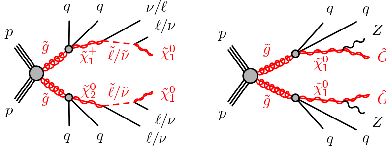
Figure 1: Decay topologies for example signal processes. A simplified model involving gluino pair production, with the gluinos following two-step decays via sleptons to neutralino LSPs is shown on the left. The diagram on the right shows a GGM decay mode, where gluinos decay via neutralinos to gravitino LSPs.
