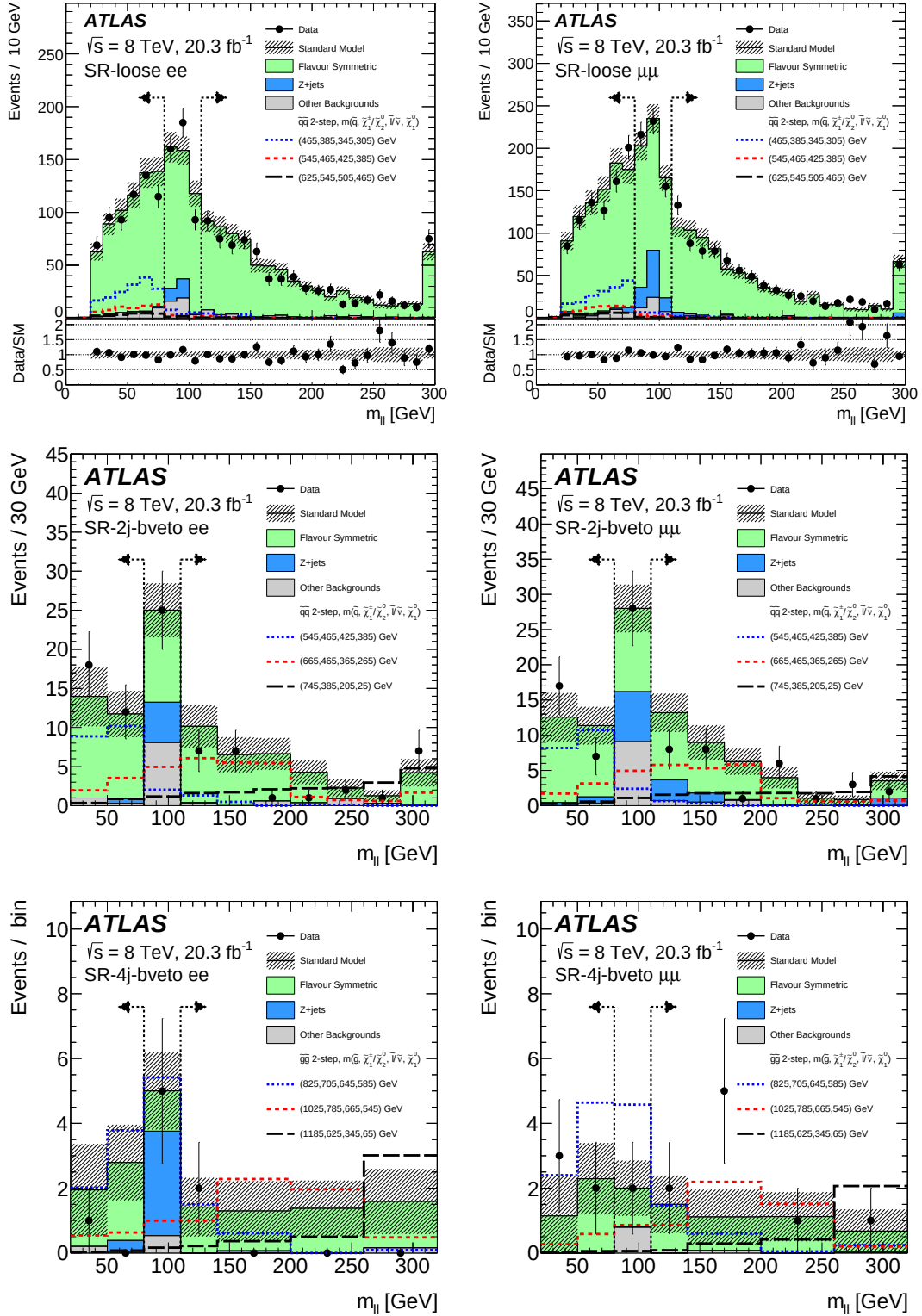
Figure 9: The observed and expected dilepton mass distributions in the off-Z SR-loose (top), SR-2j-bveto (middle), and SR-4j-bveto (bottom). The vertical dashed lines indicate the 80 < m_{\ell\ell} < 110 GeV region, which is used to normalise the Z + jets background and is thus not treated as a search region. Example signal models (dashed lines) are overlaid, with m(\tilde{q})/m(\tilde{g}) , m(\tilde{\chi}_2^0)/m(\tilde{\chi}_1^\pm) , m(\tilde{\ell})/m(\tilde{\nu}) , and m(\tilde{\chi}_1^0) of each benchmark point being indicated in the figure legend. The last bin contains the overflow. All uncertainties are included in the hatched uncertainty band.
