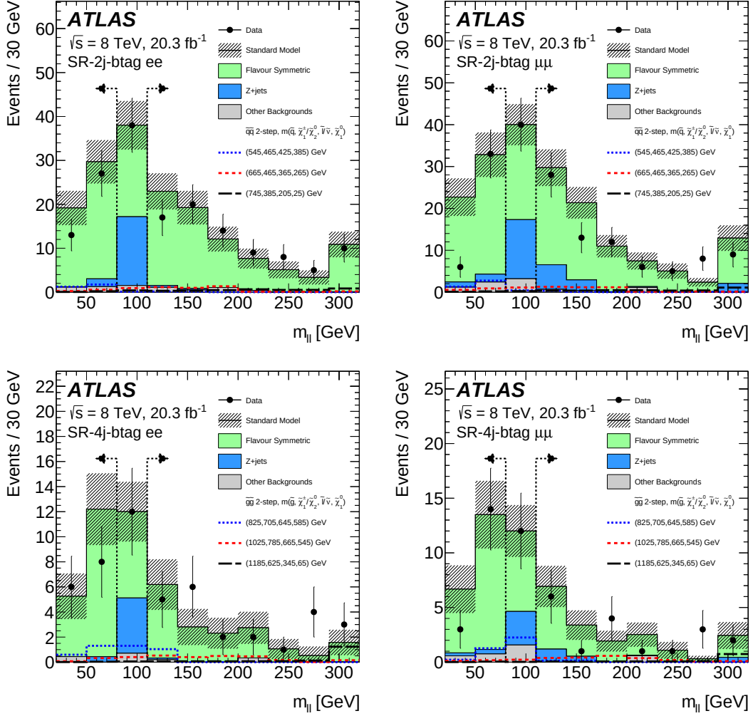
Figure 10: The observed and expected dilepton mass distributions in the SR-2j-btag (top) and SR-4j-btag (bottom) signal regions of the off-Z search. The vertical dashed lines indicate the 80 < m_{\ell\ell} < 110 GeV region, which is used to normalise the Z + jets background and is thus not treated as a search region. Example signal models of squark- or gluino-pair production (dashed lines) are overlaid, with m(\tilde{g}) , m(\tilde{\chi}_2^0)/m(\tilde{\chi}_1^\pm) , m(\tilde{\ell})/m(\tilde{\nu}) , and m(\tilde{\chi}_1^0) of each benchmark point being indicated in the figure legend. The last bin contains the overflow. All uncertainties are included in the hatched uncertainty band.
