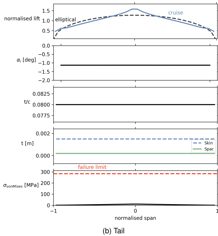
Figure 5.2: Baseline parameter distribution along wingspan
