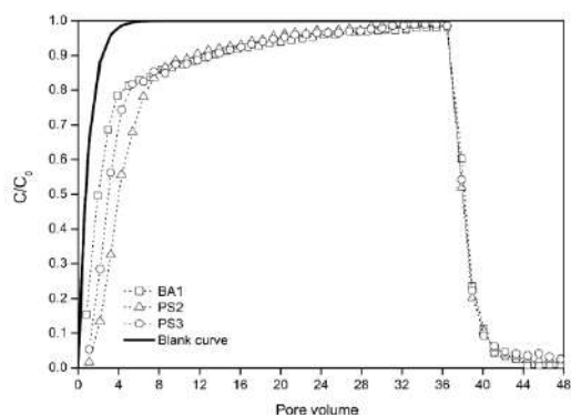
Figura 3 As curvas BTCs obtidas a pH 4 ( [U(VI)] = 1,0 \times 10^{-4} \text{ M} ) (Guimarães et al., 2016b).
