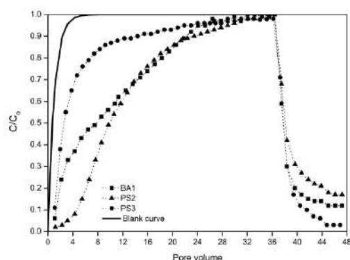
Figura 4 As curvas BTCs obtidas a pH 6 ( [U(VI)] = 1,00 \times 10^{-4} \text{ M} ) (Guimarães et al., 2016b).
