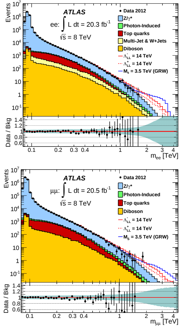
Fig. 1 Reconstructed dielectron (top) and dimuon (bottom) mass distributions for data and the SM background estimate. Also shown are the predictions for a benchmark \Lambda value in the LL contact interaction model and benchmark M_S value in the GRW ADD model. The distribution bin width is constant in \log(m_{\ell\ell}) . The ratio is presented with the total systematic uncertainty overlaid as a band.
