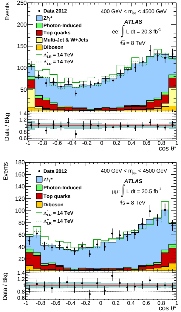
Fig. 2 Reconstructed \cos \theta^* distributions for data and the SM background estimate in the dielectron (top) and dimuon (bottom) channels. Results are shown for the contact interaction signal region for dilepton masses between 400 GeV and 4500 GeV. Also shown are the predictions for a benchmark \Lambda value in the LR contact interaction model. The ratio is presented with the total systematic uncertainty overlaid as a band.
