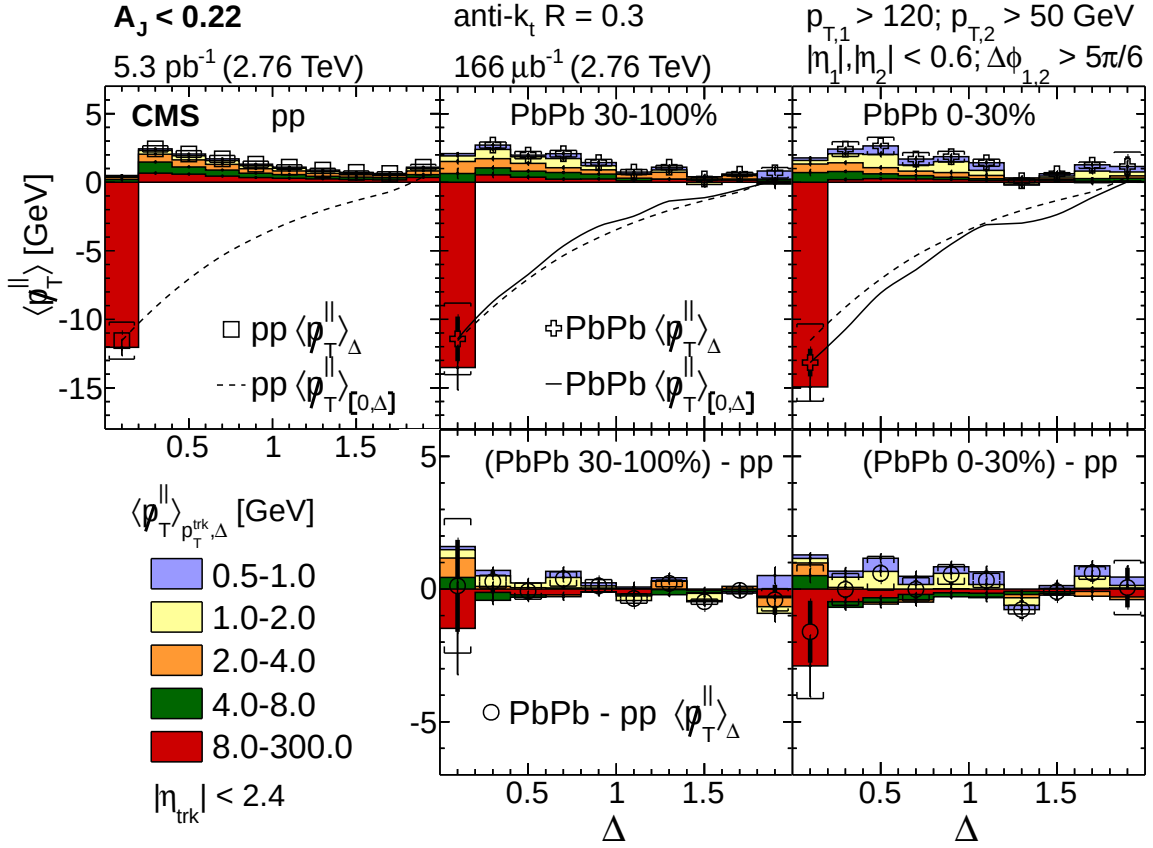
Figure 2: (Color online) Same as Fig. 1, but with a balanced dijet selection ( A_J < 0.22 ). Upper row: \langle p_T^\parallel \rangle_{p_T^{\text{trk}}, \Delta} distributions for pp, and for 30–100% and 0–30% PbPb data for five track p_T ranges (colored boxes), as a function of \Delta . Also shown is \langle p_T^\parallel \rangle_\Delta as a function of \Delta for pp (open squares) and for PbPb data (open plus symbols). Dashed lines (pp) and solid lines (PbPb) show \langle p_T^\parallel \rangle_{[0, \Delta]} (i.e. integrating the \langle p_T^\parallel \rangle_\Delta over \Delta from \Delta = 0 up to the point of interest). Lower row: Difference in the \langle p_T^\parallel \rangle_{p_T^{\text{trk}}, \Delta} distributions for the PbPb and pp according to the range in p_T , as a function of \Delta (colored boxes), and difference of \langle p_T^\parallel \rangle_\Delta as a function of \Delta (open circles). Error bars and brackets represent statistical and systematic uncertainties, respectively. The y-axis range on the top panels are smaller than in Fig. 1.
