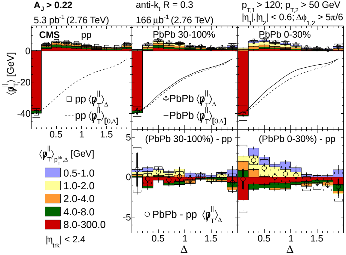
Figure 3: (Color online) Same as Fig. 1, but with an unbalanced dijet selection ( A_J > 0.22 ). Upper row: \langle p_T^\parallel \rangle_{p_T^{\text{trk}}, \Delta} distributions for pp, and for 30–100% and 0–30% PbPb data for five track p_T ranges, as a function of \Delta . Also shown is \langle p_T^\parallel \rangle_\Delta as a function of \Delta for pp and for PbPb data. Dashed lines (pp) and solid lines (PbPb) show \langle p_T^\parallel \rangle_{[0, \Delta]} (i.e. integrating the \langle p_T^\parallel \rangle_\Delta over \Delta from \Delta = 0 up to the point of interest). Lower row: Difference in the \langle p_T^\parallel \rangle_{p_T^{\text{trk}}, \Delta} distributions for the PbPb and pp. Error bars and brackets represent statistical and systematic uncertainties, respectively. The y -axis range on the top panels are larger than in Fig. 1.
