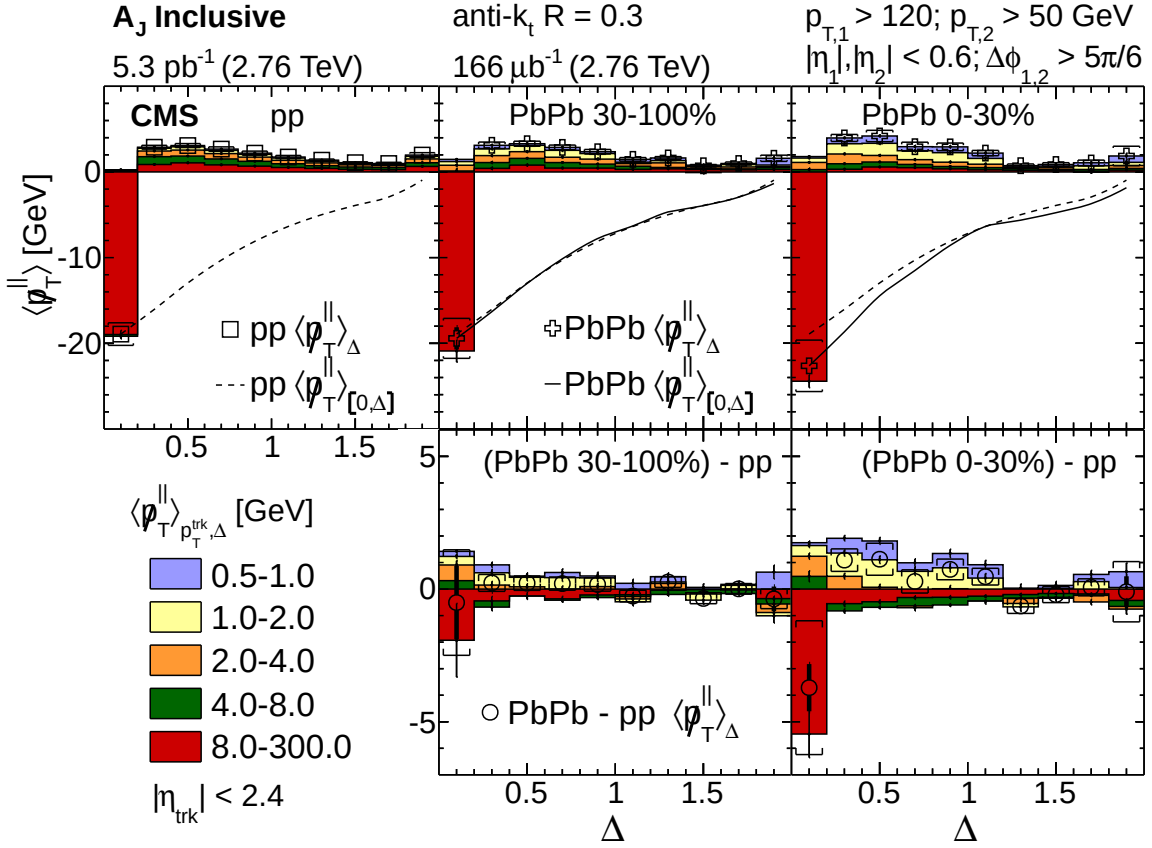
Figure 1: (Color online) Upper row: \langle p_T^\parallel \rangle_{p_T^{\text{trk}}, \Delta} distributions for pp, and for 30–100% and 0–30% PbPb data for five track- p_T ranges (colored boxes), for momentum ranges from 0.5 < p_T < 1 GeV (light blue) to 8 < p_T < 300 GeV (red), as a function of \Delta . Also shown is \langle p_T^\parallel \rangle_{\Delta} as a function of \Delta for pp (open squares) and PbPb data (open plus symbols). Dashed lines (pp) and solid lines (PbPb) show \langle p_T^\parallel \rangle_{[0, \Delta]} (i.e. integrating the \langle p_T^\parallel \rangle_{\Delta} over \Delta from \Delta = 0 up to the point of interest). Lower row: Difference between the PbPb and pp \langle p_T^\parallel \rangle_{p_T^{\text{trk}}, \Delta} distributions according to the range in p_T , as a function of \Delta (colored boxes), and difference of \langle p_T^\parallel \rangle_{\Delta} as a function of \Delta (open circles), error bars and brackets represent statistical and systematic uncertainties, respectively.
