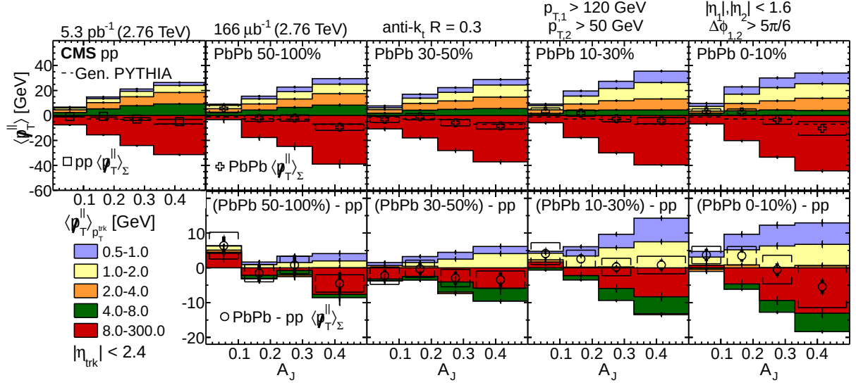
Figure 4: (Color online) Upper row has \langle p_T^\parallel \rangle_{p_{T}^{\text{trk}}} and \langle p_T^\parallel \rangle_\Sigma in pp collisions (leftmost) and in four selections of PbPb for collision centralities from 50–100% to 0–10%. The open markers show \langle p_T^\parallel \rangle_\Sigma , p_T balance for tracks with 0.5 < p_T < 300 GeV, while the colored boxes show the \langle p_T^\parallel \rangle_{p_{T}^{\text{trk}}} contributions for different track p_T ranges. For each panel, \langle p_T^\parallel \rangle_{p_{T}^{\text{trk}}} and \langle p_T^\parallel \rangle_\Sigma values are shown as a function of dijet asymmetry. The lower row shows the difference between \langle p_T^\parallel \rangle_{p_{T}^{\text{trk}}} and \langle p_T^\parallel \rangle_\Sigma for PbPb and pp data. Error bars and brackets represent statistical and systematic uncertainties, respectively.
