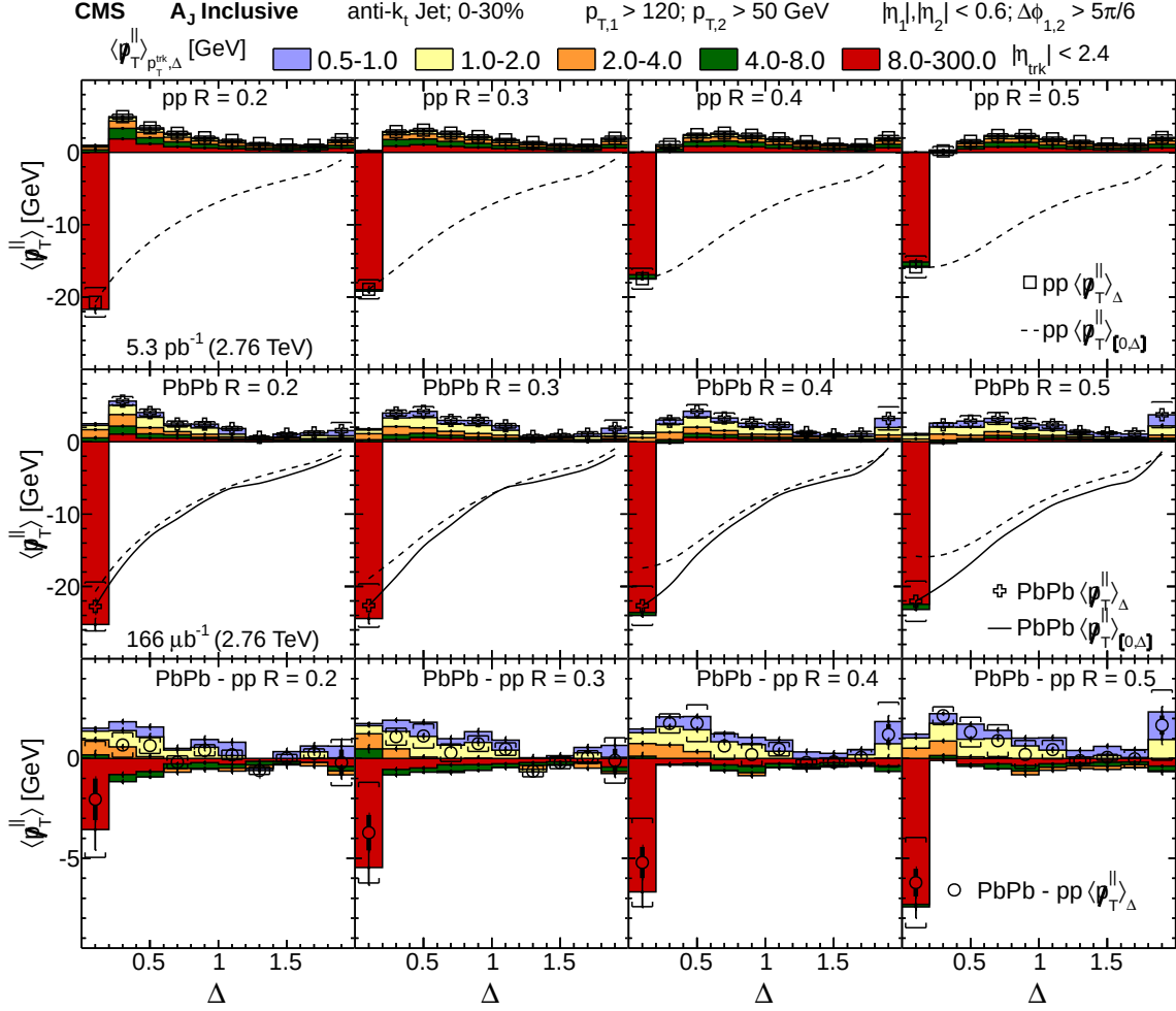
Figure 6: (Color online) Upper row shows \langle \not{p}_T^\parallel \rangle_{p_T^{\text{trk}}, \Delta} in pp collisions as a function of \Delta , for a distance parameter R = 0.2, 0.3, 0.4 , and 0.5 , from left to right for different ranges of track p_T , and \langle \not{p}_T^\parallel \rangle_{\Delta} (i.e. \langle \not{p}_T^\parallel \rangle_{p_T^{\text{trk}}, \Delta} summed over all p_T for a given \Delta bin). Dashed lines indicate cumulative results for \langle \not{p}_T^\parallel \rangle_{[0, \Delta]} in pp, for each distance parameter (i.e. integrating \langle \not{p}_T^\parallel \rangle_{\Delta} over the \Delta range from \Delta = 0 to the point of interest). Middle row provides \langle \not{p}_T^\parallel \rangle_{p_T^{\text{trk}}, \Delta} and \langle \not{p}_T^\parallel \rangle_{\Delta} in PbPb collisions of centrality range 0–30% as a function of \Delta , for distance parameters R = 0.2, 0.3, 0.4 , and 0.5 from left to right. Solid line indicates \langle \not{p}_T^\parallel \rangle_{[0, \Delta]} in PbPb for each distance parameter. Lower row has the difference between PbPb and pp. Error bars and brackets represent statistical and systematic uncertainties, respectively. The results are inclusive in the dijet asymmetry parameter A_J .
