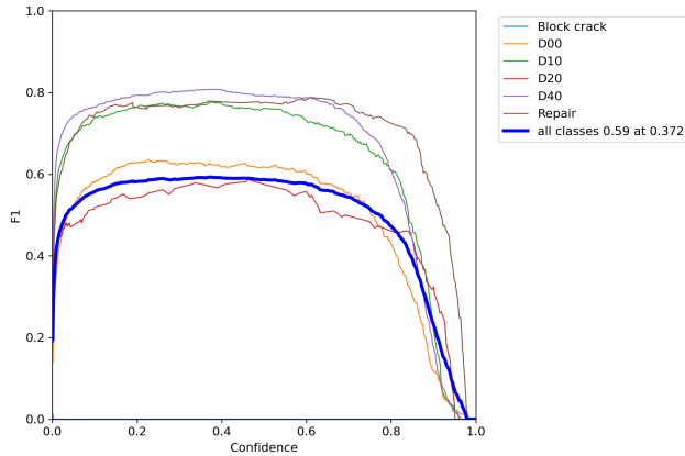
FIGURE 10. F1-Confidence Curve
