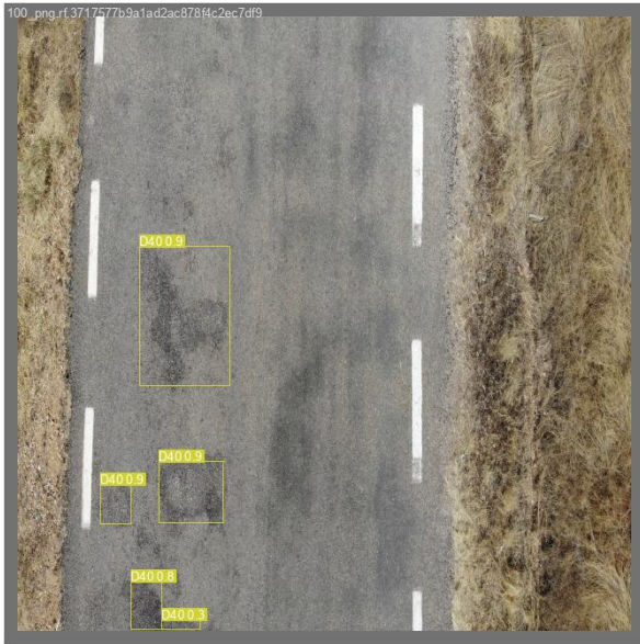
FIGURE 13. Validation YOLOv5
