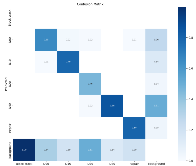
FIGURE 6. Confusion Matrix for the YOLOv5 Model
