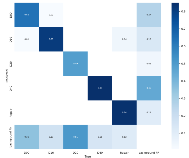
FIGURE 11. Confusion Matrix for the YOLOv5 + Transformers Prediction Head Model
