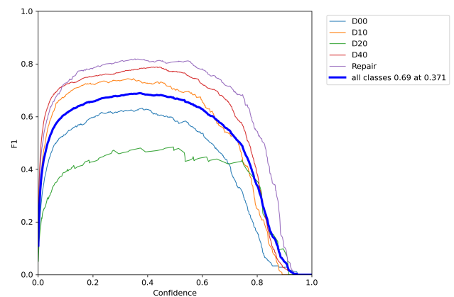
FIGURE 12. F1-Confidence Curve
