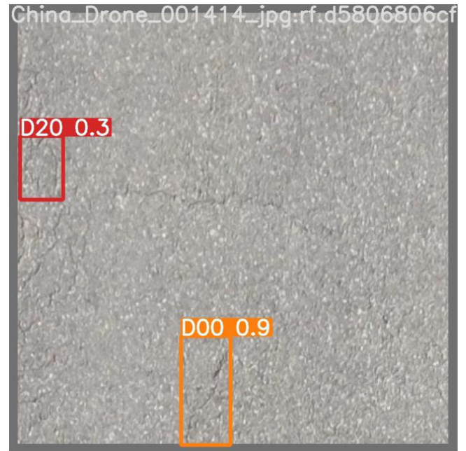
FIGURE 15. Validation YOLOv7
