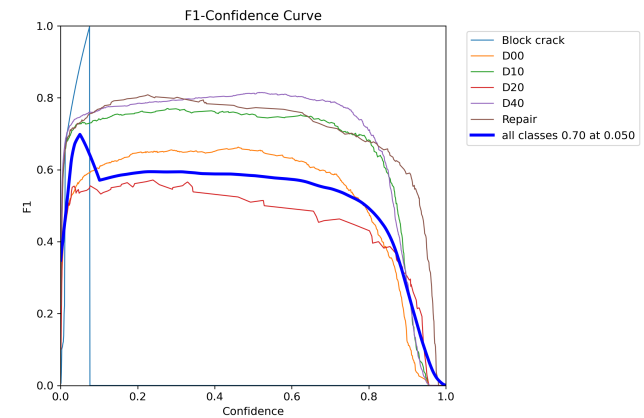
FIGURE 7. F1-Confidence Curve
