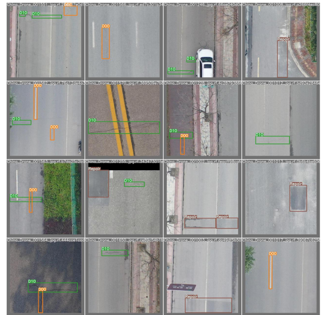
FIGURE 16. Validation YOLOv7X-W6
