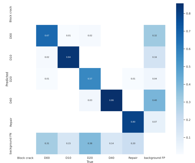
FIGURE 9. Confusion Matrix for the YOLOv7 Model
