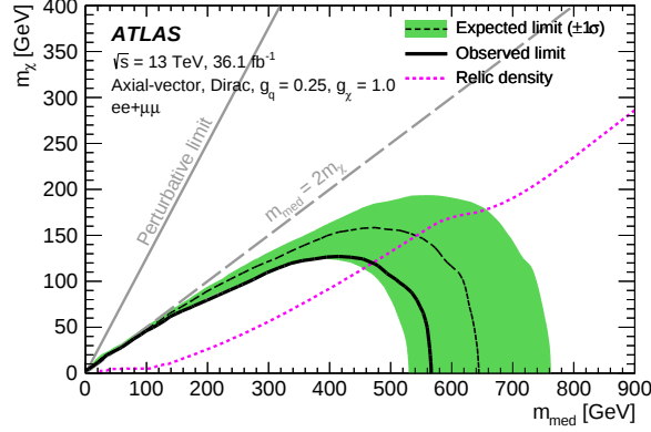
Figure 3: DM exclusion limit in the two-dimensional phase space of WIMP mass m_\chi vs mediator mass m_{\text{med}} determined using the combined ee + \mu\mu channel. Both the observed and expected limits are presented, and the 1\sigma uncertainty band for the expected limits is also provided. Regions bounded by the limit curves are excluded at the 95% CL. The grey line labelled with “ m_{\text{med}} = 2m_\chi ” indicates the kinematic threshold where the mediator can decay on-shell into WIMPs, and the other grey line gives the perturbative limit [86]. The relic density line [86] illustrates the combination of m_\chi and m_{\text{med}} that would explain the observed DM relic density.
