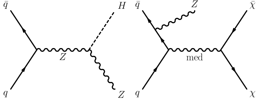
Figure 1: Leading tree-level diagrams for the ZH production (left) and the WIMP pair production in the benchmark model (right).
