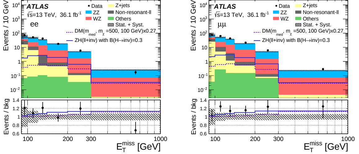
Figure 2: Observed E_T^{\text{miss}} distribution in the ee (left) and \mu\mu (right) channel compared to the signal and background predictions. The error band shows the total statistical and systematic uncertainty on the background prediction. The background predictions are presented as they are before being fit to the data. The ratio plot gives the observed data yield over the background prediction (black points) as well as the signal-plus-background contribution divided by the background prediction (blue or purple line) in each E_T^{\text{miss}} bin. The rightmost bin contains the overflow contributions. The ZH \rightarrow \ell\ell + \text{inv} signal distribution is shown with B_{H \rightarrow \text{inv}} = 0.3 , which is the value most compatible with data. The simulated DM distribution with m_{\text{med}} = 500 GeV and m_\chi = 100 GeV is also scaled (with a factor of 0.27) to the best-fit contribution.
