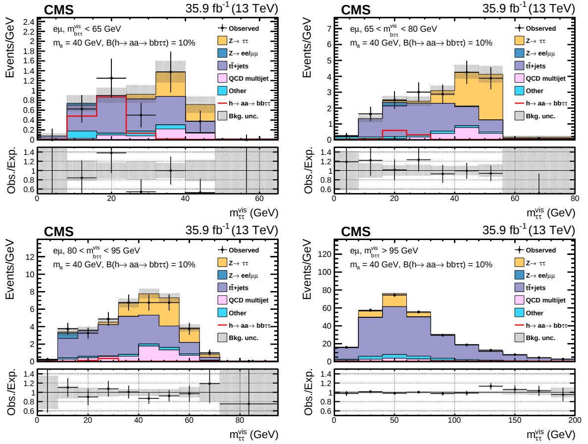
Figure 4: Distributions of m_{\tau\tau}^{\text{vis}} in the four categories of the e\mu channel. The “Other” contribution includes events from single top quark, diboson, SM Higgs boson, and W + \text{jets} productions. The signal histogram corresponds to the SM production cross section for ggh, VBF, and Vh processes, and assumes \mathcal{B}(h \rightarrow aa \rightarrow 2\tau 2b) = 10\% . The normalizations of the predicted background distributions correspond to the result of the global fit.
