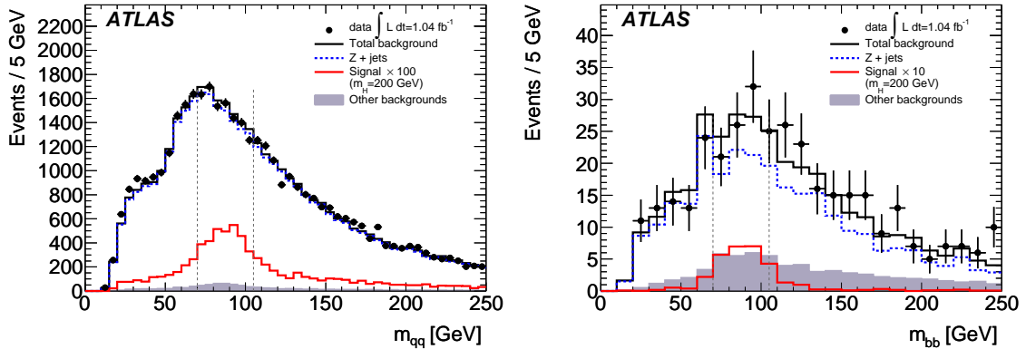
Figure 1: Distributions of the invariant mass of selected dijet pairs, m_{jj} , for the data and the MC simulation, for the untagged (left) and tagged (right) samples. The signal has been scaled up to make it more visible. The vertical lines show the range of the m_{jj} selection.
