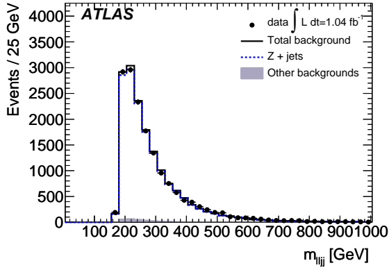
(a) m_{jj} sidebands, untagged sample.
