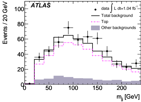
(c) m_{\ell\ell} sidebands, E_T^{\text{miss}} > 50 GeV, untagged sample.
