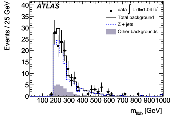
(b) m_{jj} sidebands, tagged sample.
