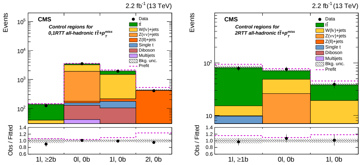
Figure 7: Observed data, and prefit and fitted background-only event yields in the control regions associated with the 0,1RTT (left) and 2RTT (right) all-hadronic t\bar{t} + p_T^{\text{miss}} signal regions. The 1 lepton, \geq 2 b tag control region (hadA in Table 2) constrains \ell + \text{jets } t\bar{t} background in the 0,1RTT signal region. This process is constrained in the 2RTT signal region using the 1 lepton, \geq 1 b tag control region (hadE). The \leq 1 lepton, 0 b tag control regions (hadB, hadC, hadF, hadG) constrain W + jets and Z + jets backgrounds, while the 2 lepton, 0 b tag control region (hadD) provides an additional constraint on the Z + jets background. The lower panels show the ratios of observed to fitted background yields. In both panels, the statistical uncertainties of the data are indicated as vertical error bars and the fit uncertainties as hatched bands. Prefit yields and the ratios of prefit to fitted background expectations are shown as dashed magenta histograms.
