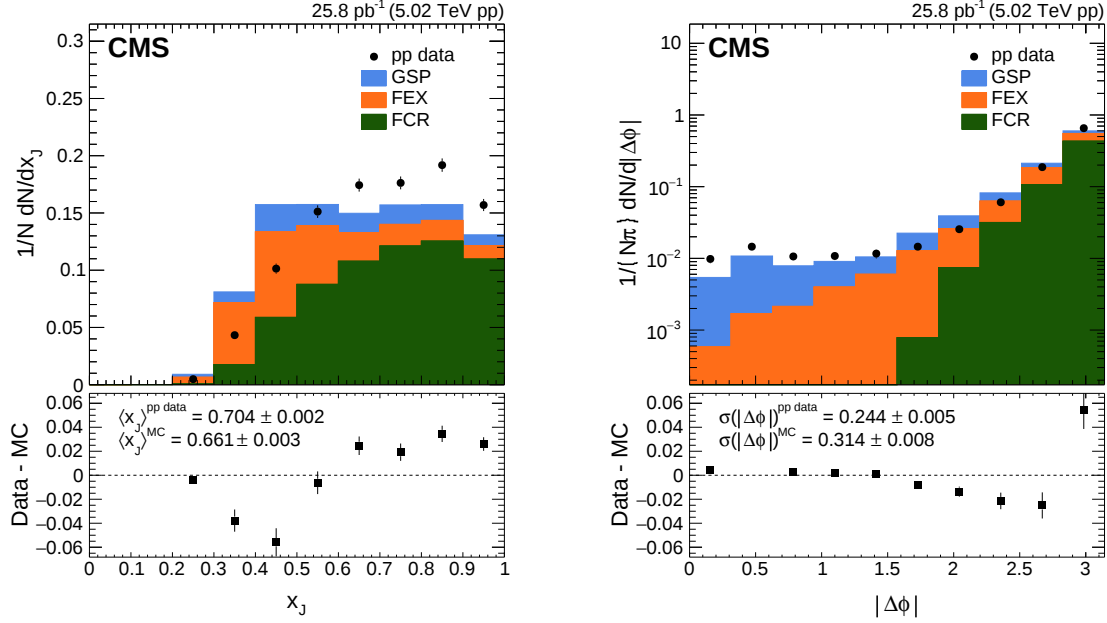
Figure 7: The distributions of x_j (left) and \Delta\phi (right) in pp collisions before flavor process reweighting. Data are shown in solid points, while the stacked histograms show the contributions of different processes in PYTHIA 6 (see text for details). The bottom set of panels show the difference between data and simulation (MC).
