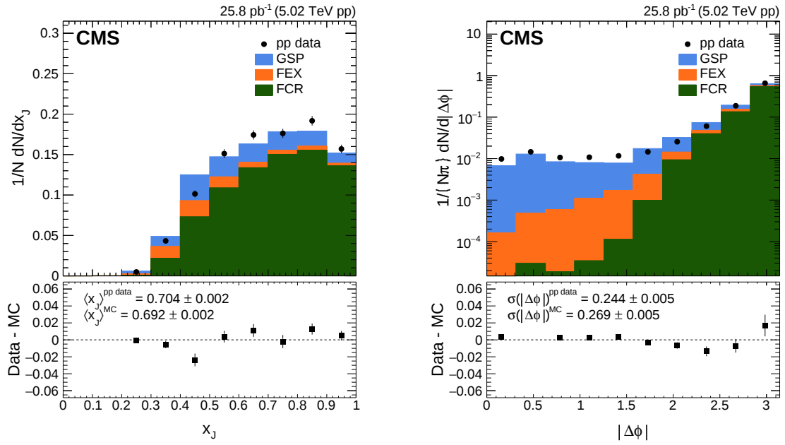
Figure 8: The distributions of x_J (left) and |\Delta\phi| (right) in pp collisions after flavor process reweighting. Data are shown in solid points, while the stacked histograms show the contributions of different processes in PYTHIA 6 (see text for details). The bottom set of panels show the difference between data and simulation (MC).
