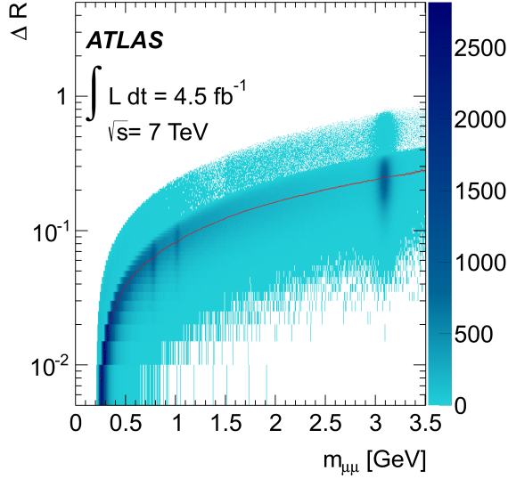
Figure 2: The opening angle \Delta R vs invariant mass for all muon pairs in the 4.5 \text{ fb}^{-1} data sample. The overlaid red points show the profile of the \Delta R distribution for each dimuon mass bin. The position of each point is the mean value of the vertical slice and its width is the RMS. The secondary distribution running along the top of the distribution arises from events with more than two muons, where a third muon triggers at a higher p_T , allowing for combinations of dimuon pairs with a larger opening angle.
