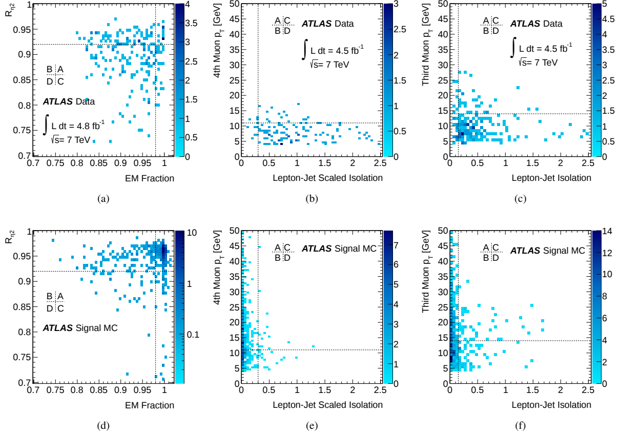
Figure 3: Variables used for ABCD-likelihood method from data (top) and MC signal (bottom) using \alpha_d = 0.1 and m_{\gamma_D} = 300 MeV for the electron channel and \alpha_d = 0.0 and m_{\gamma_D} = 300 MeV for the two muon channels. The dashed black lines show the cuts used to define the four regions. Shown are (left) Electron-jet: R_{\eta 2} vs EM fraction; (centre) double muon-jet: scaled isolation vs p_T of the fourth muon; (right) single muon-jet: scaled isolation vs p_T of the third muon.
