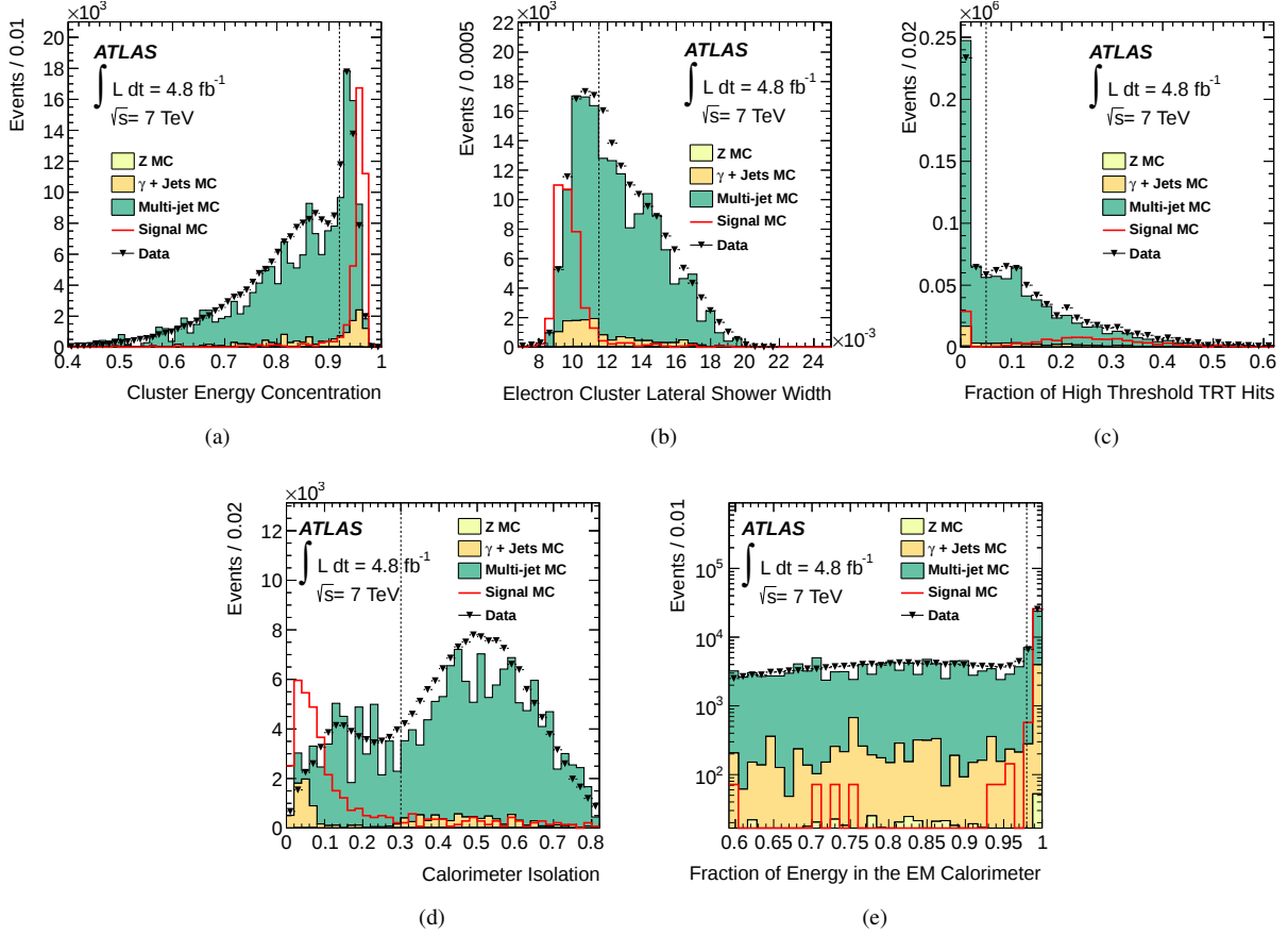
Figure 1: Distributions of the five discriminating variables used after selection of events which have passed the trigger and contain two or more electron-jet candidates, shown separately for the multi-jet, Z \rightarrow ee and \gamma + \text{jets} backgrounds as well as for the signal sample with \alpha_d = 0.0 and m_{\gamma_D} = 150 MeV. The signal MC normalization is arbitrary. The dashed black vertical line shows the cut values at (a) cluster energy concentration R_{\eta_2} \geq 0.92 , (b) electron cluster lateral shower width w_{\eta_2} \leq 0.0115 , (c) fraction of high threshold TRT hits f_{HT} \geq 0.05 , (d) calorimeter isolation \leq 0.3 , and (e) fraction of energy in the EM calorimeter f_{EM} \geq 0.98 . The hadronic jet and \gamma + \text{jets} distributions are shown here from PYTHIA MC for illustrative purposes.
