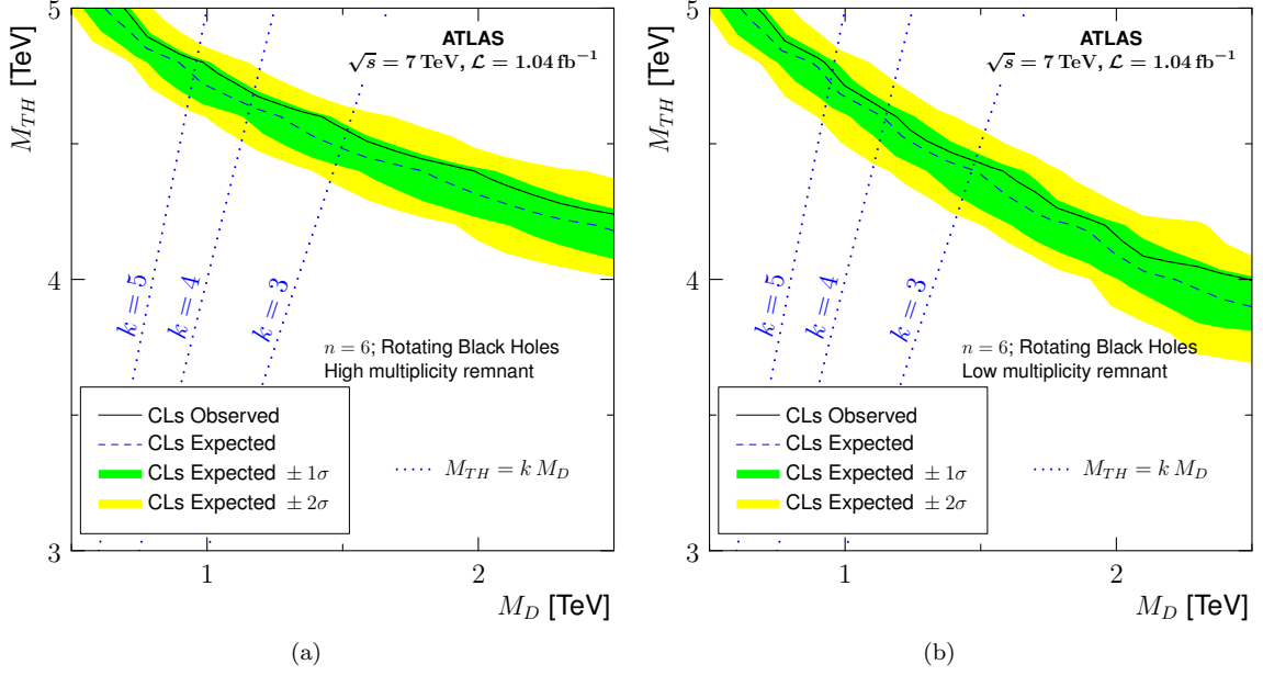
Figure 4: The exclusion limit in the M_{TH} - M_D plane, with electron and muon channels combined, for rotating black hole models with six extra dimensions. The black hole decays result in a high-multiplicity remnant state generated with BLACKMAX (a), and a low-multiplicity remnant state generated by CHARYBDIS (b). The solid (dashed) line shows the observed (expected) 95% C.L. limits, with the dark and light bands illustrating the expected 1\sigma and 2\sigma variations of the expected limits. The dotted lines indicate constant k = M_{TH}/M_D .
