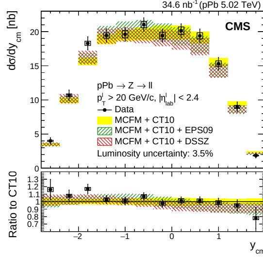
Figure 2: Differential cross section of the Z bosons in pPb collisions as a function of rapidity in the fiducial region for the combined leptonic decay channel. Colored boxes are predictions from the MCFM generator, scaled by 208 (see text), and using nuclear (EPS09 and DSSZ) or free (CT10) PDF sets. The bottom panel shows the ratio of the data and the nPDF predictions to the CT10 PDF set. The vertical bars (boxes) represent the statistical (systematic) uncertainties.
