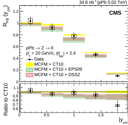
Figure 3: Forward-backward asymmetry R_{FB} distribution of the Z bosons in pPb collisions as a function of rapidity in the fiducial region for the combined leptonic decay channel compared to the predictions from the MCFM generator with nuclear (EPS09 and DSSZ) or free (CT10) PDF sets. The bottom panel shows the ratio of the data and the nPDF predictions to the CT10 PDF set. The vertical bars (boxes) represent the statistical (systematic) uncertainties.
