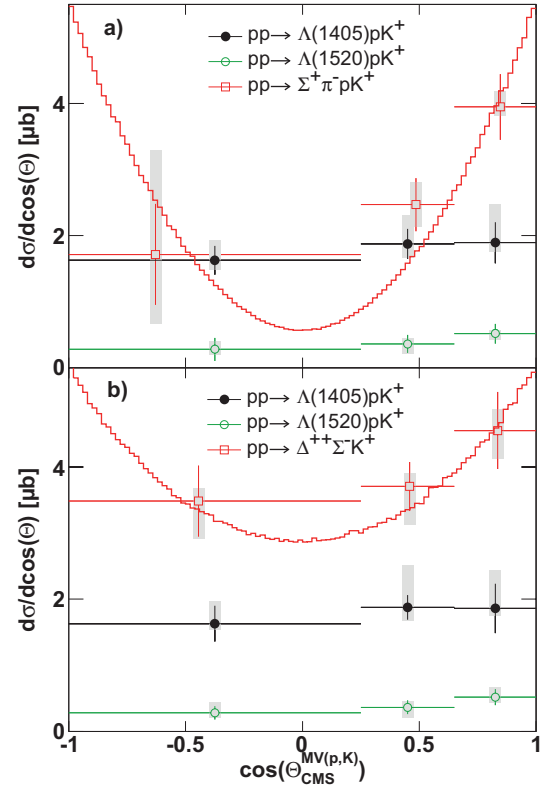
FIG. 3. (Color online) Differential cross-section for the different simulated reaction channels as a function of \cos(\theta_{\text{CMS}}^{\text{MV}(p, K)}) for the \Sigma^+\pi^- decay channel a) and the \Sigma^-\pi^+ decay channel b). The cross-sections are obtained by integrating the simulations, which have been fitted to the experimental data. The gray boxes indicate the systematic errors. The solid histograms show the angular distribution used to fold the simulation of the reactions p + p \rightarrow \Sigma^+ + \pi^- + p + K^+ and p + p \rightarrow \Delta^{++} + \Sigma^- + K^+ , respectively.
