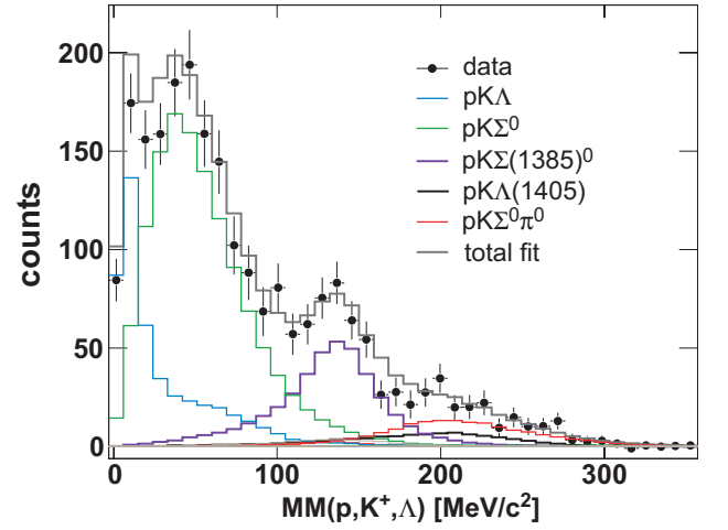
FIG. 2. (Color online) Missing mass to the p , \Lambda and K^+ particles. The colored histograms show the contributions of the simulated channels 6-9. The experimental data are uncorrected. See the text for details.
