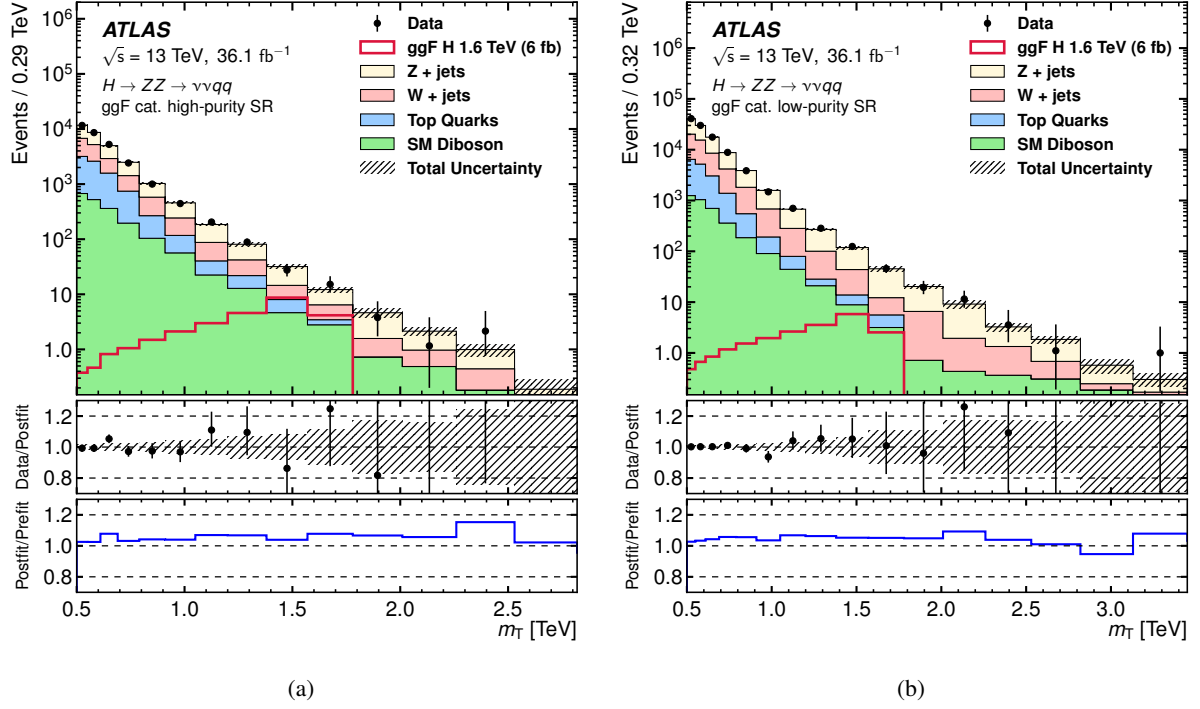
Figure 10: Comparisons of the observed data and expected background distributions of m_T in the ggF category of the H \rightarrow ZZ \rightarrow \nu\nu qq search: (a) high-purity and (b) low-purity signal regions. For illustration, expected distributions from the ggF production of a 1.6 TeV Higgs boson with \sigma \times \mathcal{B}(H \rightarrow ZZ) = 6 fb are also shown. The middle panes show the ratios of the observed data to the background predictions. The uncertainty in the total background prediction, shown as bands, combines statistical and systematic contributions. The blue triangles in the middle panes indicate bins where the ratio is nonzero and outside the vertical range of the plot. The bottom panes show the ratios of the post-fit and pre-fit background predictions.
