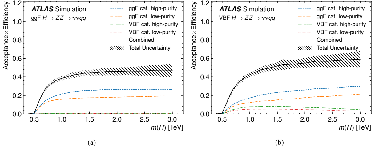
Figure 6: Selection acceptance times efficiency for the H \rightarrow ZZ \rightarrow \nu\nu qq events from MC simulations as a function of the Higgs boson mass for (a) ggF and (b) VBF production, combining the HP and LP signal regions. The hatched band represents the total statistical and systematic uncertainties.
