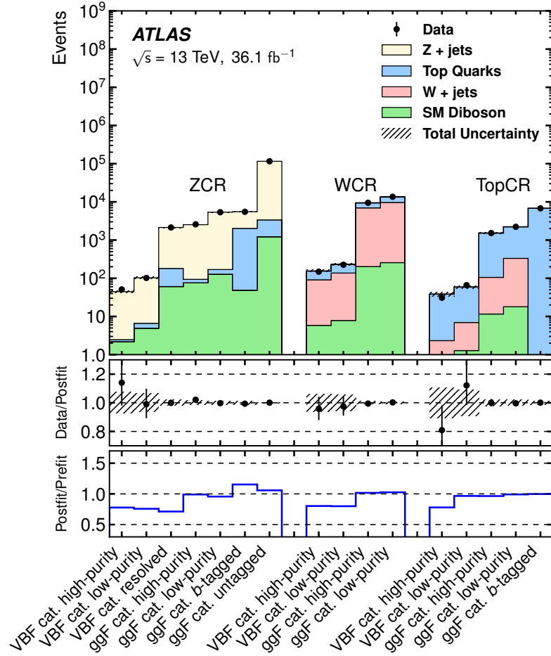
Figure 11: Comparisons of the observed data and expected background event yields in each control region. The middle pane shows the ratios of the observed data to the post-fit background predictions. The uncertainty in the total background prediction, shown as bands, combines statistical and systematic contributions. The bottom pane shows the ratios of the post-fit and pre-fit background predictions.
