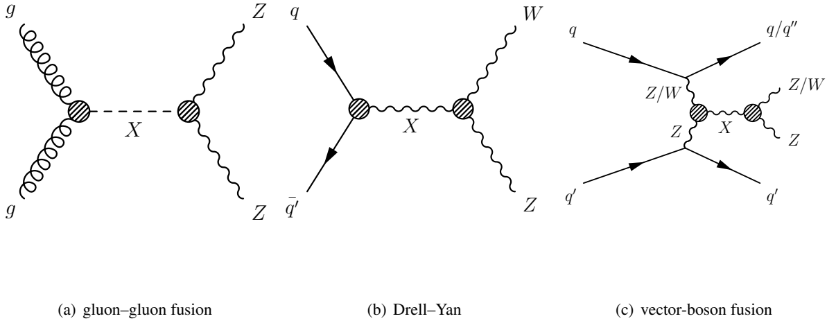
Figure 1: Representative Feynman diagrams for the production of heavy resonances X with their decays into a pair of vector bosons.
