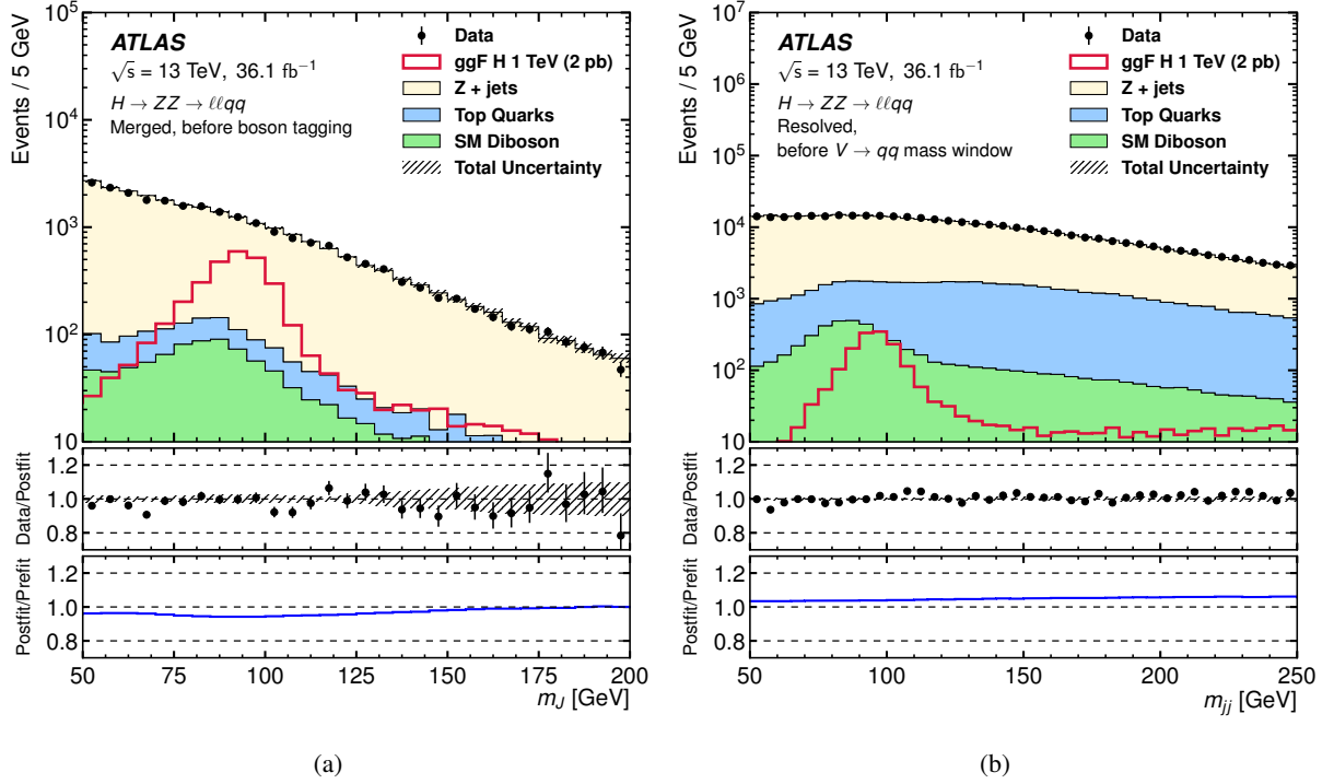
Figure 3: Observed and expected distributions of (a) the large- R jet mass m_J of the ZV \rightarrow \ell\ell J candidate and (b) the dijet mass m_{jj} of the ZV \rightarrow \ell\ell jj candidate. These distributions are for the H \rightarrow ZZ search before the identification of the V \rightarrow qq decay, combining VBF and ggF/DY categories. Background contributions are obtained from the combined likelihood fit to the data, as explained in Section 8. For illustration, expected distributions from the ggF production of a 1 TeV Higgs boson with \sigma \times \mathcal{B}(H \rightarrow ZZ) = 2 pb are also shown. The middle panes show the ratios of the observed data to the background predictions. The uncertainty in the total background prediction, shown as bands, combines statistical and systematic contributions. The bottom panes are the ratios of the post-fit and pre-fit background predictions.
