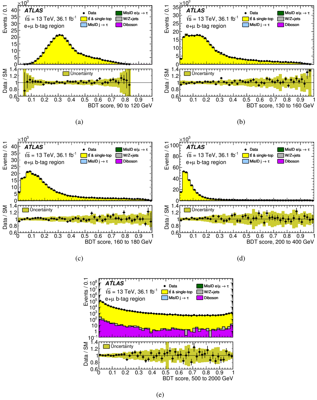
Figure 3: BDT score distribution for the predicted backgrounds and data in a region with the same event selection as for the \tau_{\text{had-vis}} + \text{lepton} channel, except for the requirement of an e\mu pair instead of the e/\mu + \tau_{\text{had-vis}} pair (as described in the text). The five H^+ mass range trainings are shown. The lower panel of each plot shows the ratio of data to the SM background prediction. The uncertainty bands include all statistical and systematic uncertainties.
