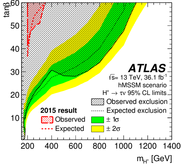
Figure 9: 95% CL exclusion limits on \tan\beta as a function of m_{H^+} , shown in the context of the hMSSM, for the regions in which theoretical predictions are available ( 0.5 \leq \tan\beta \leq 60 ). In the case of the expected limits, one- and two-standard-deviation uncertainty bands are also shown. As a comparison, the red curves near the upper-left corner show the observed and expected exclusion limits based on the dataset of 3.2 \text{ fb}^{-1} collected in 2015 at \sqrt{s} = 13 \text{ TeV} [22].
