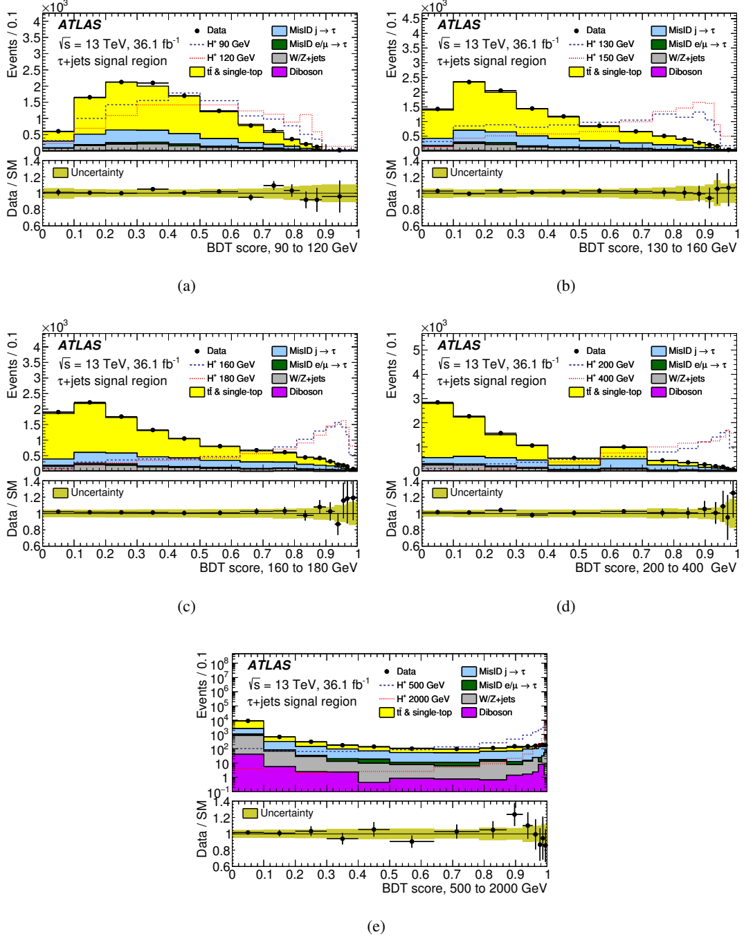
Figure 5: BDT score distributions in the signal region of the \tau_{\text{had-vis}}+\text{jets} channel, in the five mass ranges used for the BDT trainings, after a fit to the data with the background-only hypothesis. The lower panel of each plot shows the ratio of data to the SM background prediction. The uncertainty bands include all statistical and systematic uncertainties. The normalisation of the signal (shown for illustration) corresponds to the integral of the background.
