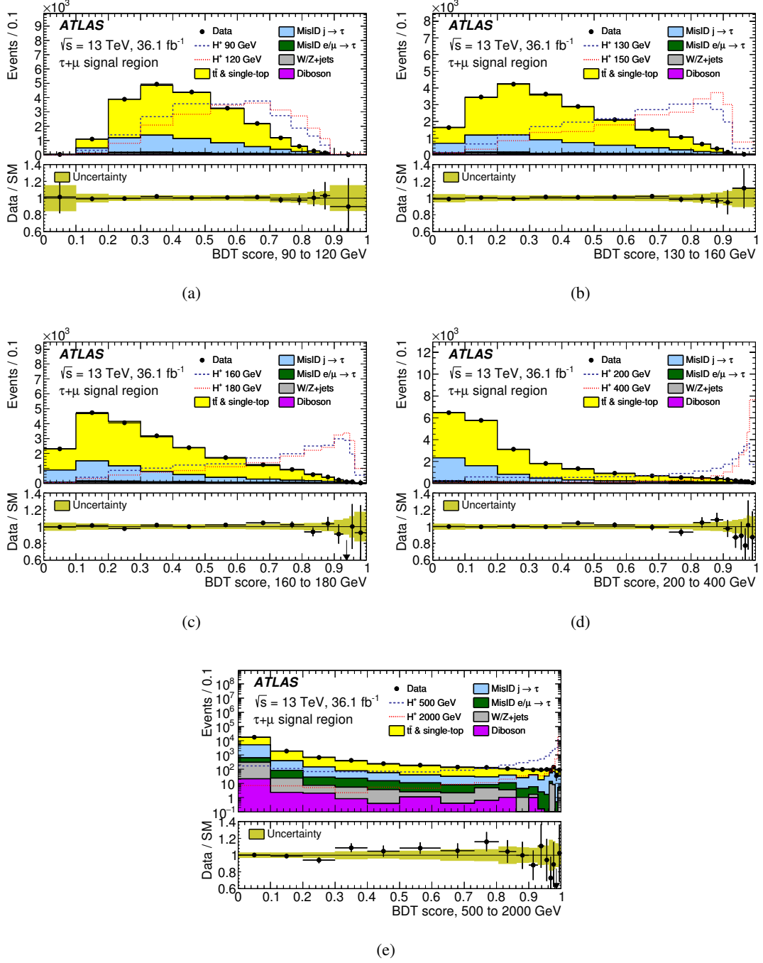
Figure 7: BDT score distributions in the signal region of the \tau_{\text{had-vis}}+\mu\text{on} sub-channel, in the five mass ranges used for the BDT trainings, after a fit to the data with the background-only hypothesis. The lower panel of each plot shows the ratio of data to the SM background prediction. The uncertainty bands include all statistical and systematic uncertainties. The normalisation of the signal (shown for illustration) corresponds to the integral of the background.
