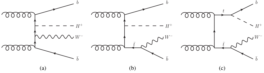
Figure 1: Examples of leading-order Feynman diagrams contributing to the production of charged Higgs bosons in pp collisions: (a) non-resonant top-quark production, (b) single-resonant top-quark production that dominates at large H^+ masses, (c) double-resonant top-quark production that dominates at low H^+ masses. The interference between these three main diagrams becomes most relevant in the intermediate-mass region.
