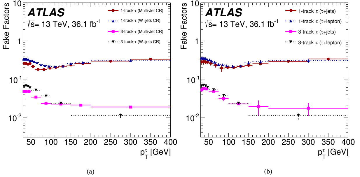
Figure 2: Fake factors parameterised as a function of p_T^\tau and the number of charged \tau decay products (two categories: 1-prong and 3-prong), as obtained (a) in the multi-jet and W+\text{jets} CRs, (b) after reweighting by \alpha_{MJ} in the \tau_{\text{had-vis}}+\text{jets} and \tau_{\text{had-vis}}+\text{lepton} channels. Details about the computation of fake factors in the different control regions are given in the text. The errors shown represent the statistical uncertainty in a given p_T^\tau bin (a) and with additional systematic uncertainties obtained from the combination in a given p_T^\tau bin (b).
