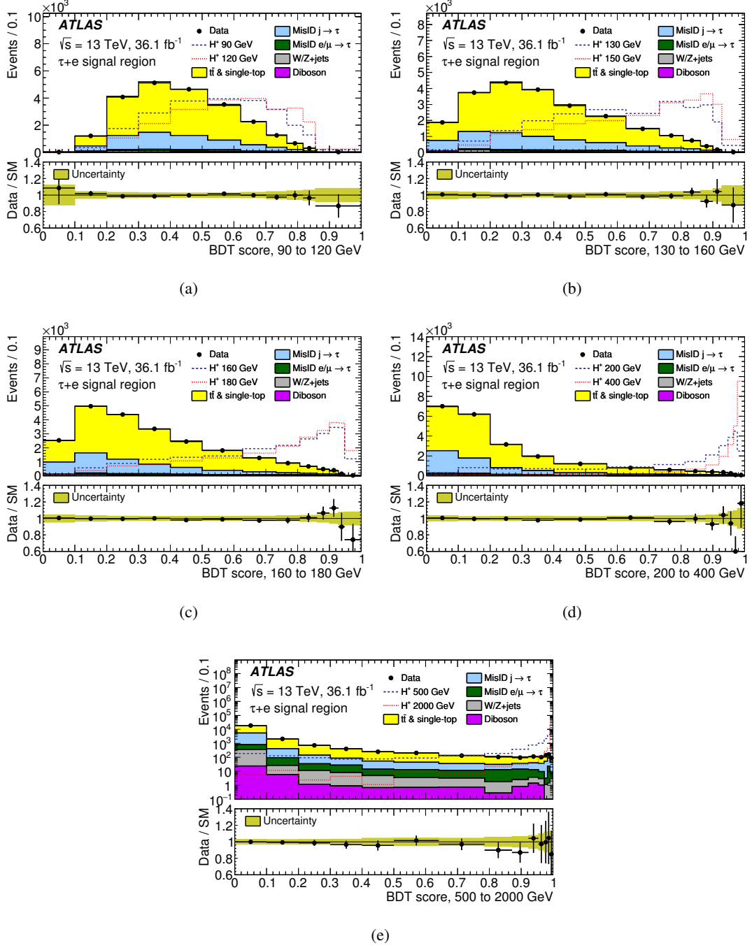
Figure 6: BDT score distributions in the signal region of the \tau_{\text{had-vis}} + \text{electron} sub-channel, in the five mass ranges used for the BDT trainings, after a fit to the data with the background-only hypothesis. The lower panel of each plot shows the ratio of data to the SM background prediction. The uncertainty bands include all statistical and systematic uncertainties. The normalisation of the signal (shown for illustration) corresponds to the integral of the background.
