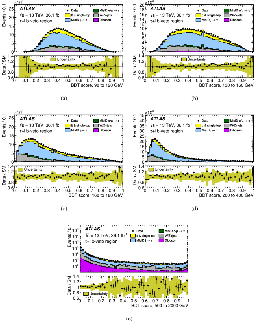
Figure 4: BDT score distribution for the predicted backgrounds and data in a region with the same event selection as for the \tau_{\text{had-vis}}+\text{lepton} channel, except that it has exactly zero b -tagged jet (as described in the text). The five H^+ mass range trainings are shown. The lower panel of each plot shows the ratio of data to the SM background prediction. The uncertainty bands include all statistical and systematic uncertainties.
