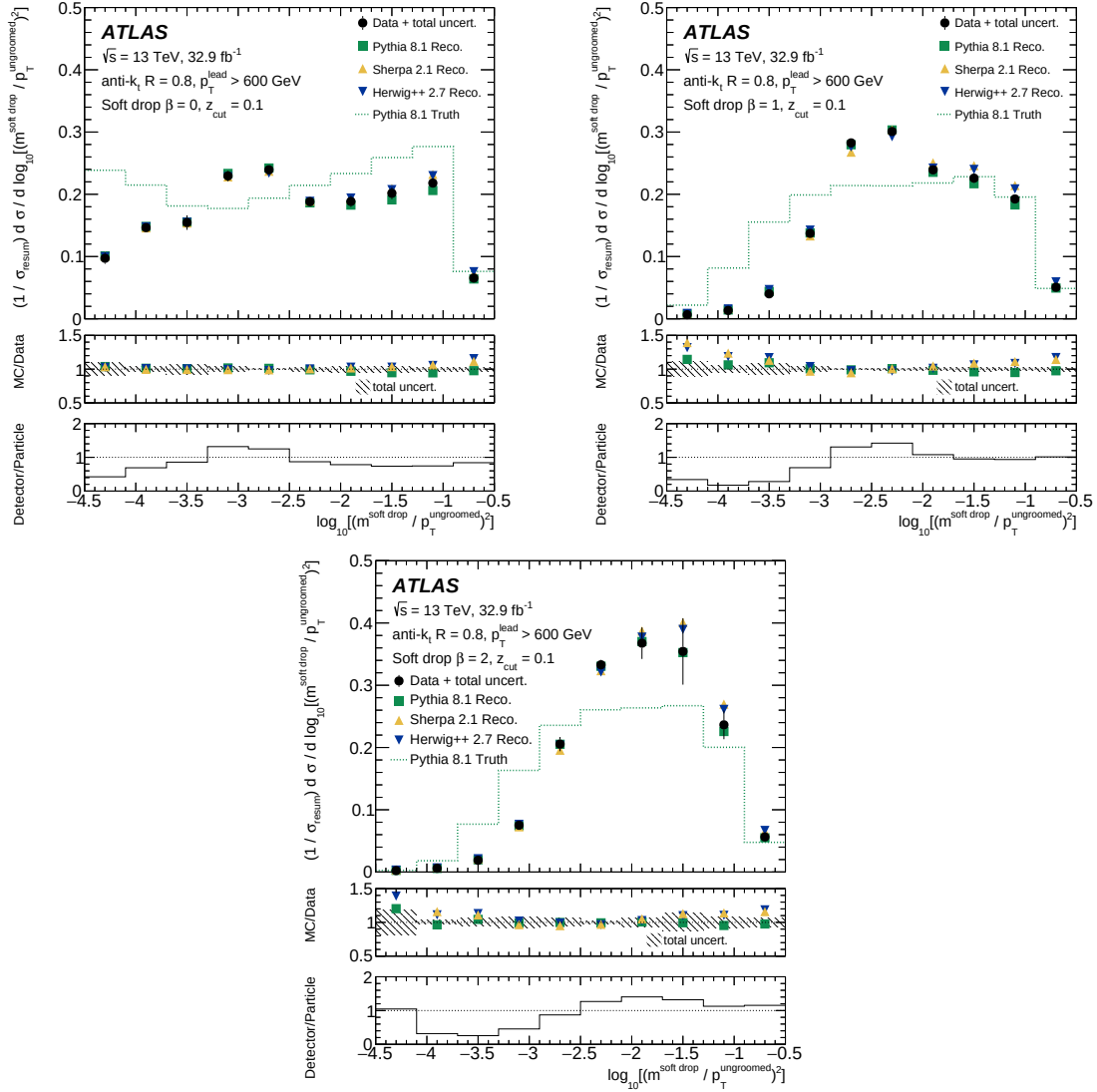
Figure 1: Distributions of \log_{10}(\rho^2) in data compared to reconstructed detector-level (Reco.) PYTHIA, SHERPA, and HERWIG++, and particle-level (Truth) PYTHIA simulations for \beta = 0 (left), \beta = 1 (right), and \beta = 2 (bottom). The ratio of the three detector-level MC predictions to the data is shown in the middle panel, and the size of the detector \rightarrow particle-level corrections for PYTHIA is shown as the ratio in the bottom panel. The error bars on the data points and in the first ratio include the experimental systematic uncertainties in the cluster energy, angular resolution, and efficiency. The distributions are normalized to the integrated cross-section, \sigma_{\text{resum}} , measured in the resummation region, -3.7 < \log_{10}(\rho^2) < -1.7 .
