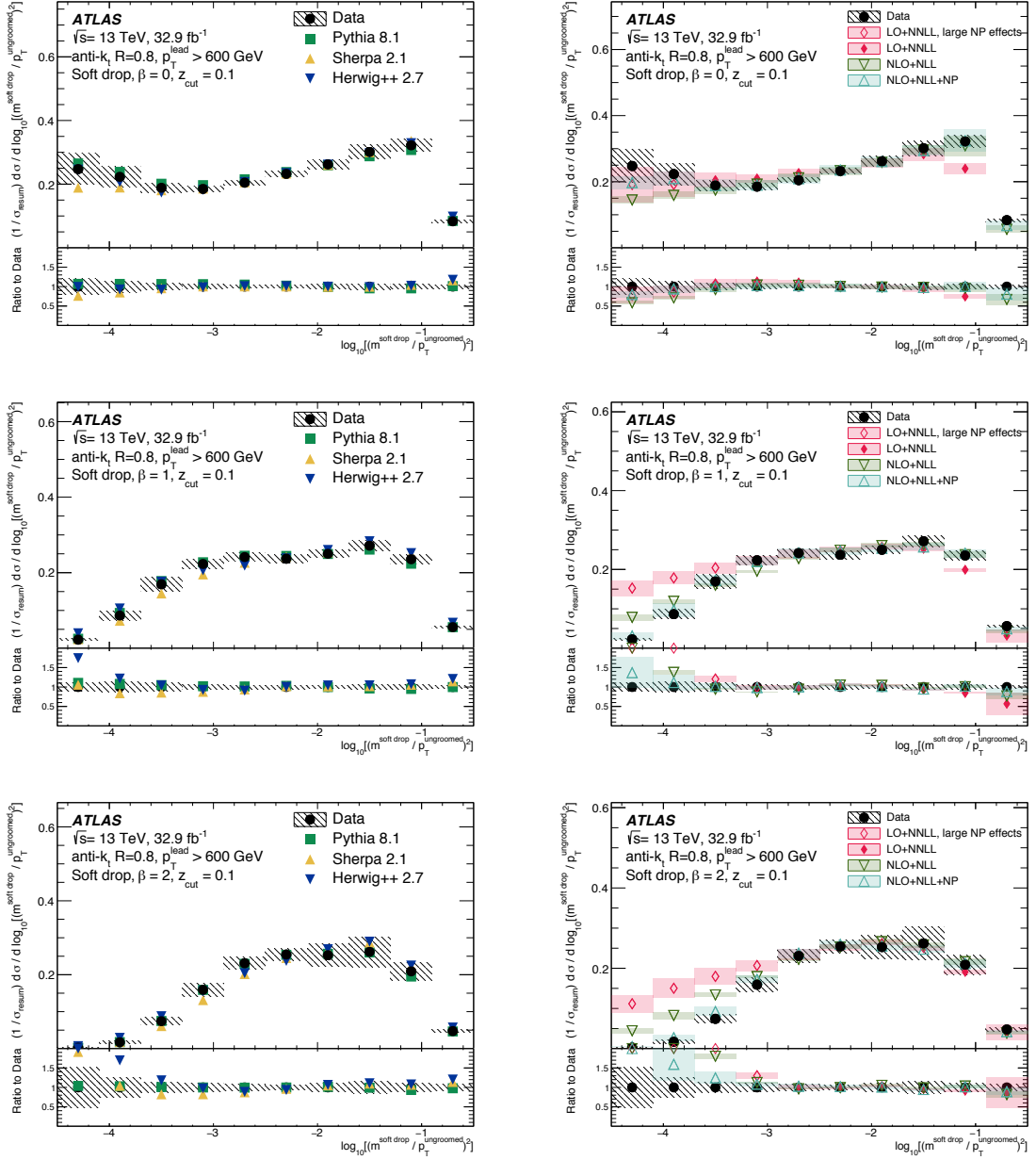
Figure 3: The unfolded \log_{10}(\rho^2) distribution for anti- k_T , R = 0.8 jets with p_T^{\text{lead}} > 600 GeV, after the soft drop algorithm is applied for \beta \in \{0, 1, 2\} , in data compared to PYTHIA, SHERPA, and HERWIG++ particle-level (left), and NLO+NLL(+NP) [15] and LO+NNLL [17, 18] theory predictions (right). The LO+NNLL calculation does not have non-perturbative (NP) corrections; the region where these are expected to be large is shown in an open marker (but no correction is applied), while regions where they are expected to be small are shown with a filled marker. All uncertainties described in the text are shown on the data; the uncertainties from the calculations are shown on each one. The distributions are normalized to the integrated cross section, \sigma_{\text{resum}} , measured in the resummation region, -3.7 < \log_{10}(\rho^2) < -1.7 . The NLO+NLL+NP cross-section in this resummation regime is 0.14, 0.19, and 0.21 nb for \beta = 0, 1, 2 , respectively [15].
