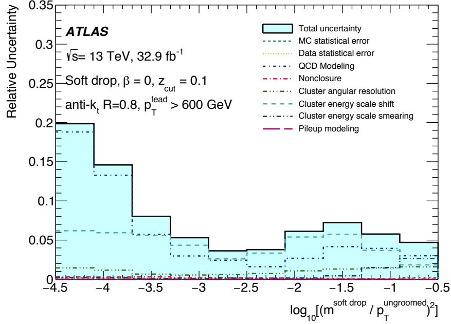
Figure 2: The breakdown of systematic and statistical uncertainties as a function of \log_{10}(\rho^2) for \beta = 0 .
