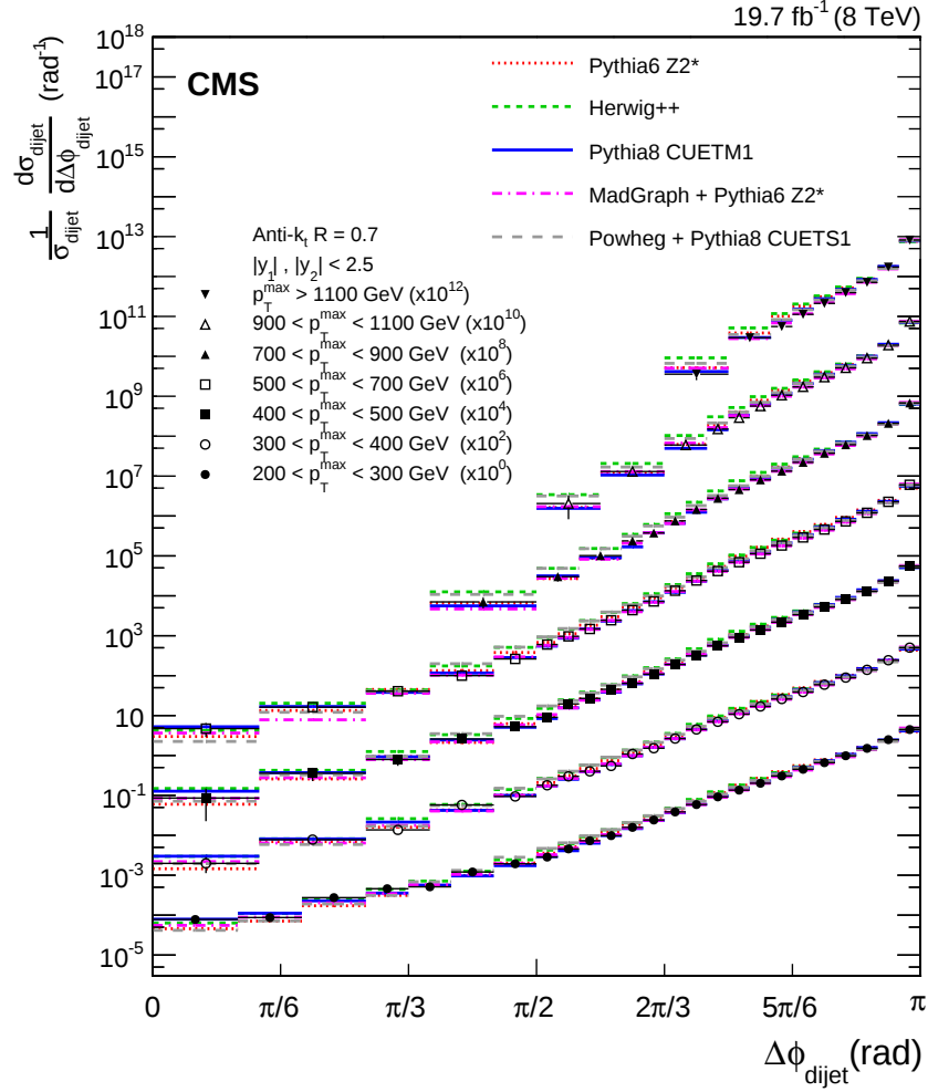
Figure 4: Normalized dijet cross section differential in \Delta\phi_{\text{dijet}} for seven p_T^{\text{max}} regions, scaled by multiplicative factors for presentation purposes. The error bars on the data points include statistical and systematic uncertainties. Overlaid on the data are predictions from the PYTHIA6, HERWIG++, PYTHIA8, MADGRAPH + PYTHIA6, and POWHEG + PYTHIA8 event generators.
