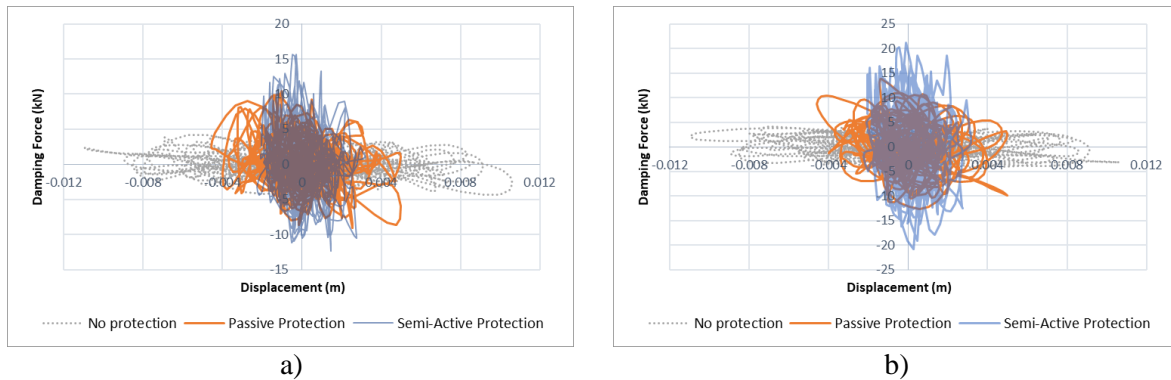
Fig. 11 – Force-Displacement Graph under seismic action Type 2: a) Storey 1; b) Storey 2
