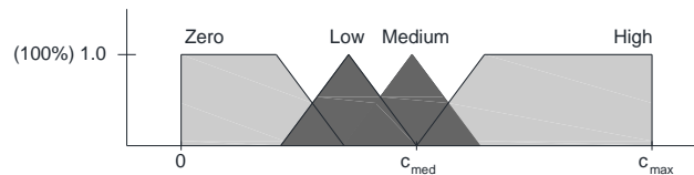
Fig. 3 – Output membership functions
