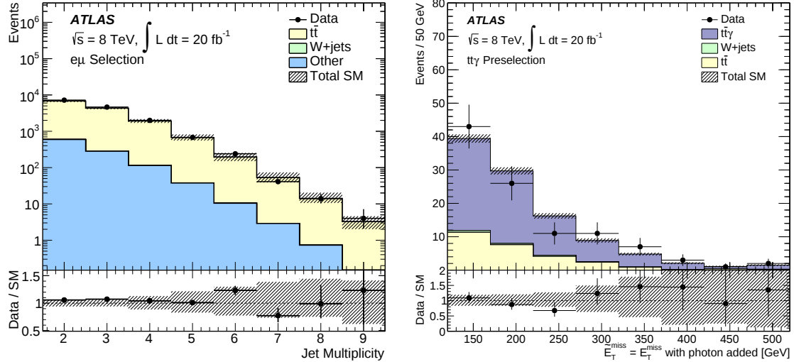
Figure 12. Left: Jet multiplicity distribution for events with one opposite charged electron-muon pair and at least two jets of which one or more is b -tagged. Other processes include single top quark production, t\bar{t} production in association with a vector boson, Z +jets, and diboson production. Right: Missing transverse momentum where photons are treated as invisible particles ( \tilde{E}_T^{\text{miss}} ) for an event selection of t\bar{t} + \text{photon} (described in the text). Both plots: The uncertainty band includes all statistical and experimental uncertainties, and the last bins include overflows.
