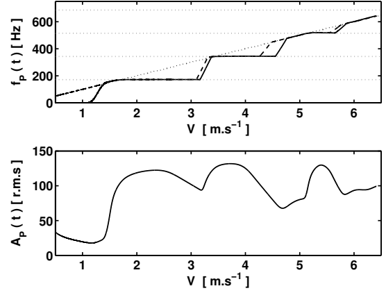
Figure 1: Increasing linear velocity sweep on the characteristic frequency of the vortex oscillators for a perfectly tuned 101-oscillator pipe. Case for strong coupling. A=0.005 , B=0.0001 , C=-200 , \alpha=3 . Instantaneous frequency and amplitude of the internal pressure at the oscillator location x_{10}=0.0982 m. The frequency of the oscillator has been superposed with dashed line (- -) to highlight the lock-in stages. The dots in the diagonal represents the Strouhal law. Horizontal dots are for the pipe modal frequencies.
