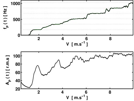
Figure 4: Increasing linear velocity sweep on the characteristic frequency of the vortex oscillators for a mistuned 101-oscillator pipe. Weak coupling C=-30 . Standard deviation of St , \sigma=0.02 . Same legend as in Figure 1.
