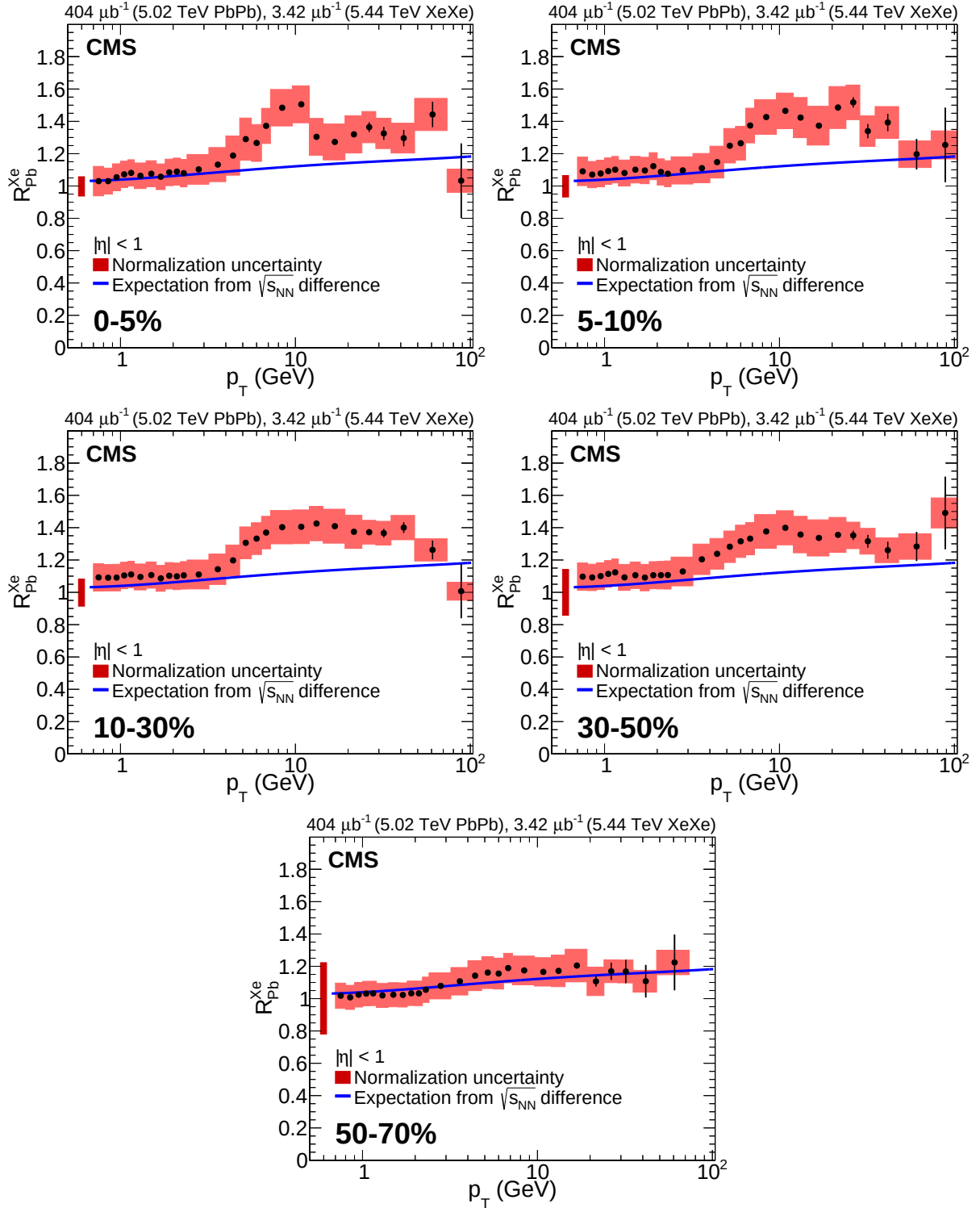
Figure 5: The measurement of R_{\text{Pb}}^{\text{Xe}} in five centrality classes using the results of this analysis and data from Ref. [17]. The blue line represents the expected deviation from unity caused by the different center-of-mass energies of the two collision systems. The solid pink boxes represent the systematic uncertainties.
