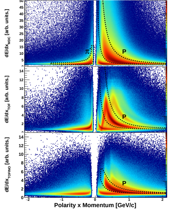
FIG. 2. (Color online). Specific energy loss measured by the MDCs (upper row) as well as TOF (middle row) / TOFINO (bottom row) versus the product of the polarity and momentum of the particle. Particles are selected by two-dimensional graphical cuts depicted as dashed lines.
