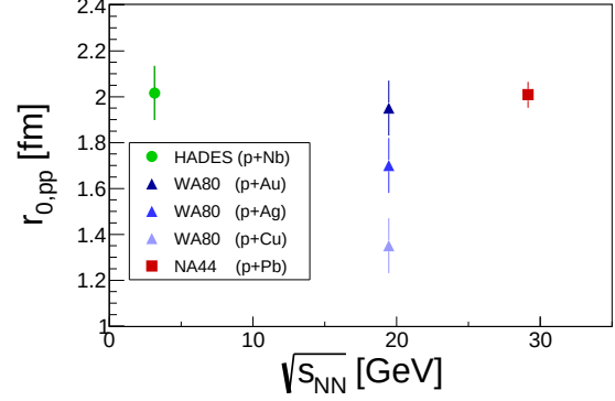
FIG. 8. (Color online). Gaussian source radii evaluated from pp correlations in p+A systems as a function of the nucleon-nucleon center-of-mass energy. The (green) full circle corresponds to the HADES measurement, blue triangles to data of WA80 [51] and the (red) square was derived by NA44 [52].
