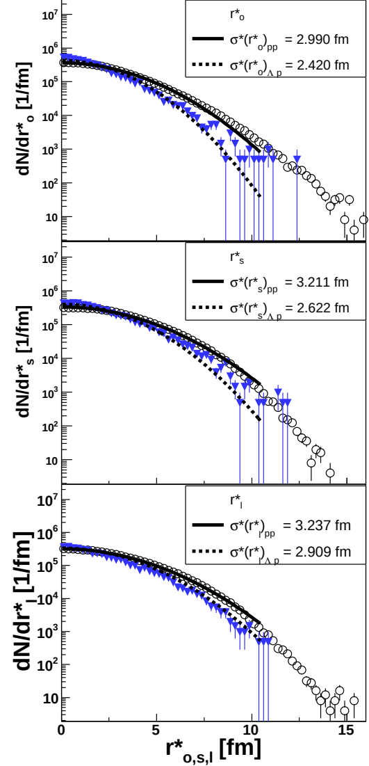
FIG. 10. (Color online). Distribution of the relative distances obtained from URQMD simulations calculated in the PRF. Full triangles depict the outcome for \Lambda p pairs (scaled to be shown with pp in one plot) and open circles are the result for pp pairs. The dotted and solid lines represent results of corresponding Gaussian fits according to Eq. (11).
