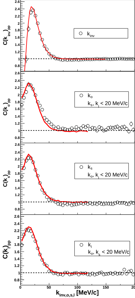
FIG. 9. (Color online). Comparison of the experimental pp correlation function (open circles) with predictions from URQMD+CRAB ((red) solid line).
