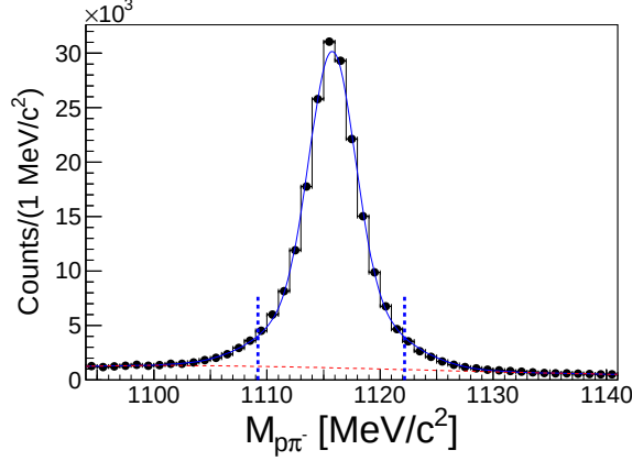
FIG. 3. (Color online). Invariant mass distribution of p\pi^- pairs after using topological cuts (comb. 3 in Table I). Dots are for data, while the curve shows the (blue) solid curve represents the fit of the signal and the (red) dashed line the background contribution. The two vertical (blue) dashed lines correspond to the two sigma region with \sigma_\Lambda = 3.24 \pm 0.01 \text{ MeV}/c^2 .
