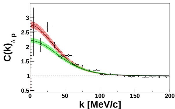
FIG. 11. (Color online). Comparison of the experimental \Lambda p correlation function (open circles with error bars) to the LO (green) and NLO (red) scattering parameter set included in Eq. (4). The error bands in the theory curves correspond to the errors of the \Lambda p source size determination.
