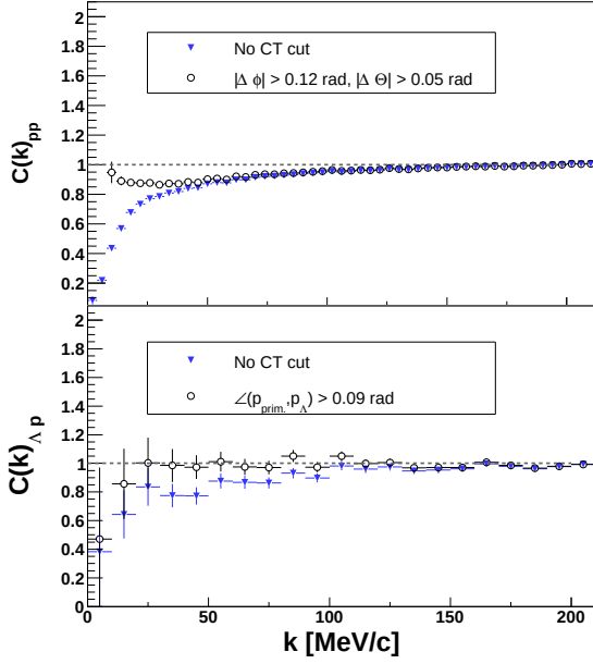
FIG. 1. (Color online). Influence of the close track (CT) rejection on simulated 1D correlation functions for uncorrelated pp (top - URQMD) and \Lambda p pairs (bottom - GiBUU). Open circles represent the correlation functions after the applied rejection cuts for close pairs while the (blue) triangles depict correlation signals without employing CT cuts.
