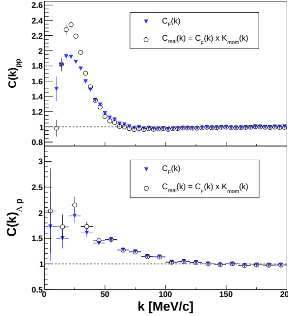
FIG. 5. (Color online). Influence of the finite momentum resolution on the experimental correlation function for pp pairs (top) and \Lambda p (bottom). Open circles display the unsmearing and (blue) triangles the smeared experimental correlation functions.
