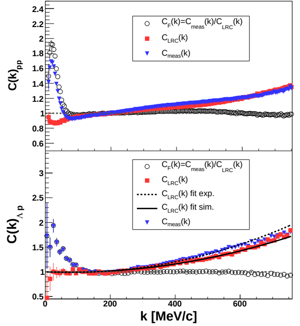
FIG. 4. (Color online). Effects due to long range correlations on the correlation function for pp pairs (top) and \Lambda p pairs (bottom). The open circles depict the experimental correlation function corrected for long range correlations. (Blue) triangles show the experimental function with long range correlations inside and (red) squares the correlation function obtained from transport simulations. The solid and dashed lines in the lower panel show the fit with polynomial functions to the simulated and experimental LRC, respectively. See text for details.
