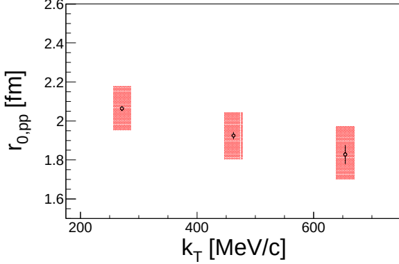
FIG. 7. (Color online). Source size of pp pairs as a function of the total transverse momentum of the pair.
