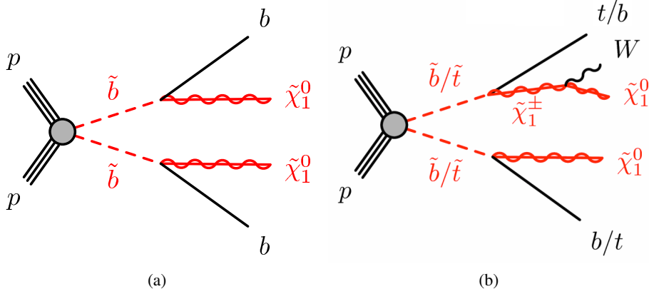
Figure 1: Diagrams illustrating the signal scenarios considered for the pair production of bottom and top squarks targeted by the (a) zero-lepton and (b) one-lepton channel selections. In (a) bottom squarks decay to a bottom quark and the lightest neutralino. In (b), decays via intermediate charginos are kinematically available and compete. If the mass difference \Delta m(\tilde{\chi}_1^\pm, \tilde{\chi}_1^0) is small, the W bosons from chargino decays are off-shell.
