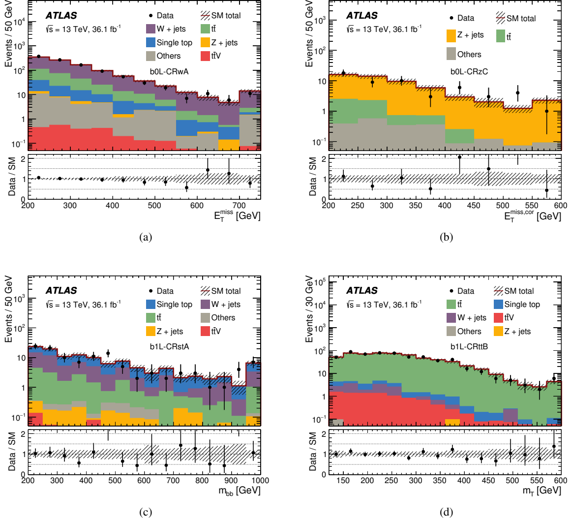
Figure 2: Example kinematic distributions in some of the control regions. (a) E_T^{\text{miss}} in b0L-CRwA, (b) E_T^{\text{miss,cor}} in b0L-CRzC, (c) m_{bb} in b1L-CRstA and (d) m_T in b1L-CRttB. In all distributions the MC normalization is rescaled using the results from the background-only fit, showing good agreement between data and the predicted SM shapes. The contributions from diboson, multijet and rare backgrounds are collectively called “Others”. The shaded-grey band shows the detector-related systematic uncertainties and the statistical uncertainties of the MC samples as detailed in Section 7 and the last bin includes overflow events.
