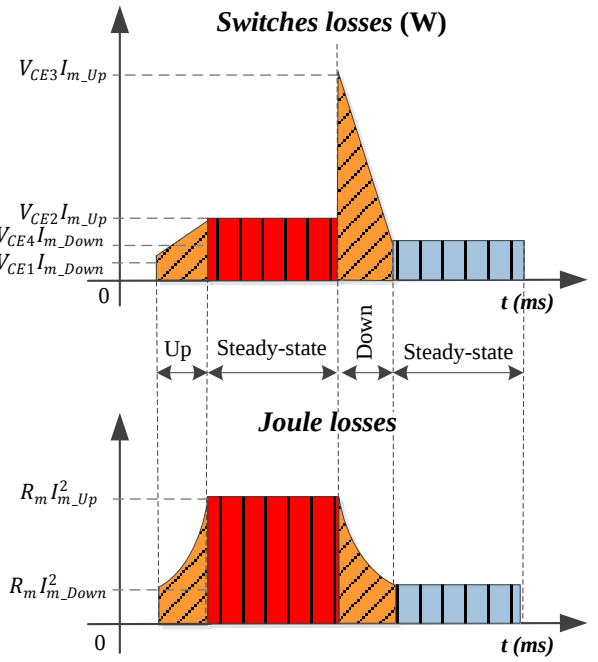
Fig. 11. Power losses along a current cycle ( V_{CE} – voltage drop of the switches; i_{m\_Up} – steady-state magnet current during the Up mode; i_{m\_Down} – steady-state magnet current during the Down mode)
