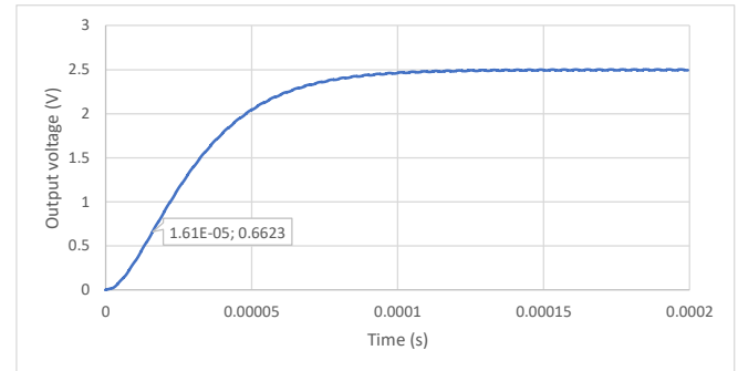
Figure 12. Step response.
