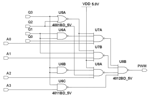
Figure 8. Pulse filter sub-circuit.
