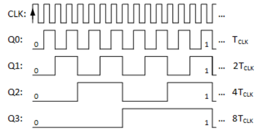
Figure 6. Output of the binary counter. The width of the pulses increases as a power of 2.
