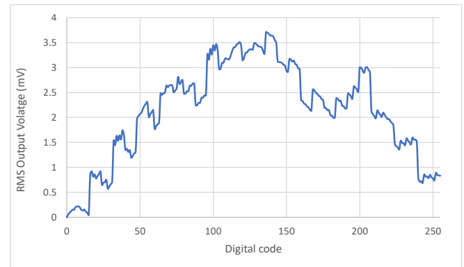
Figure 10. Noise figure.
