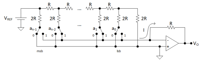
Figure 2. R-2R ladder network.
