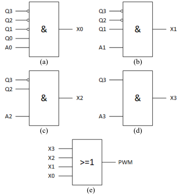
Figure 7. Pulse filtering from the LSB ( X_0 ) to the MSB ( X_3 ) followed by adding (OR gate).
