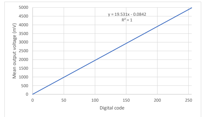
Figure 9. Static characteristic.
