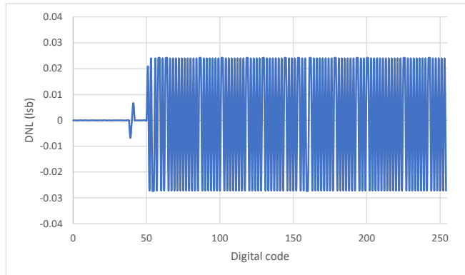
Figure 11. DNL.
