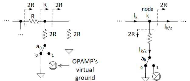
Figure 3. Detail of single node of the R-2R ladder network.
