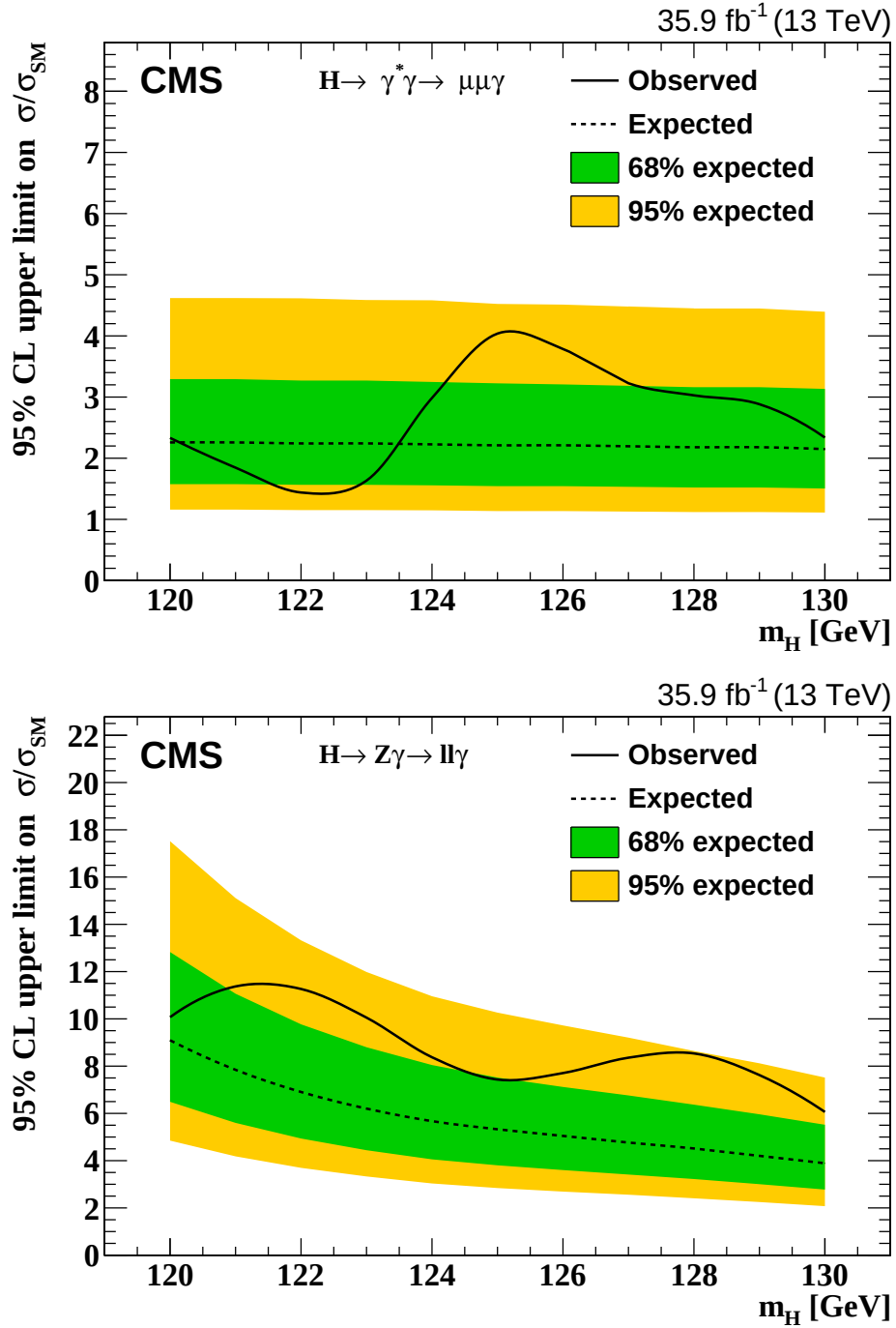
Figure 6: Exclusion limit, at 95% CL, on the cross section of the H \rightarrow \gamma^* \gamma \rightarrow \mu\mu\gamma process (upper plot) and the H \rightarrow Z\gamma \rightarrow \ell\ell\gamma process (lower plot) relative to the SM prediction, as a function of the Higgs boson mass.
