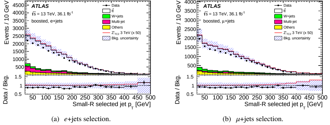
Figure 6: The distribution of the transverse momentum of the hardest small- R jet with \Delta R(\ell, \text{jet}) < 1.5 in the (a) boosted e +jets, and (b) boosted \mu +jets selections. The SM background components are shown as stacked histograms. The shaded areas indicate the total systematic uncertainties. The lower panels in each plot show the ratio of data (points) and a signal example (line) to the background expectation.
