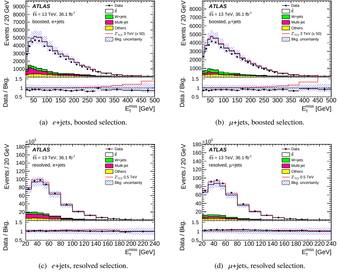
Figure 5: The distribution of the E_T^{\text{miss}} in the (a) boosted e +jets, (b) boosted \mu +jets, (c) resolved e +jets, and (d) resolved \mu +jets selections. The SM background components are shown as stacked histograms. The shaded areas indicate the total systematic uncertainties. The lower panels in each plot show the ratio of data (points) and a signal example (line) to the background expectation.
