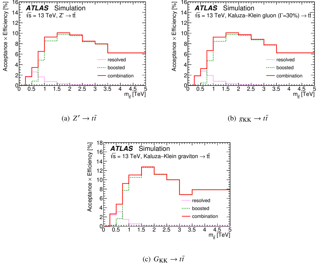
Figure 2: Acceptance times efficiency ( A \times \epsilon ), including the branching ratio for MC simulated BSM particles decaying into t\bar{t} , as a function of the t\bar{t} invariant mass m_{t\bar{t}} (computed before parton radiation) for simulated signal events. The signal samples shown here include events from generated masses ranging from 0.4 TeV to 5 TeV. All t\bar{t} decay modes are simulated. The e and \mu channel efficiencies are combined.
