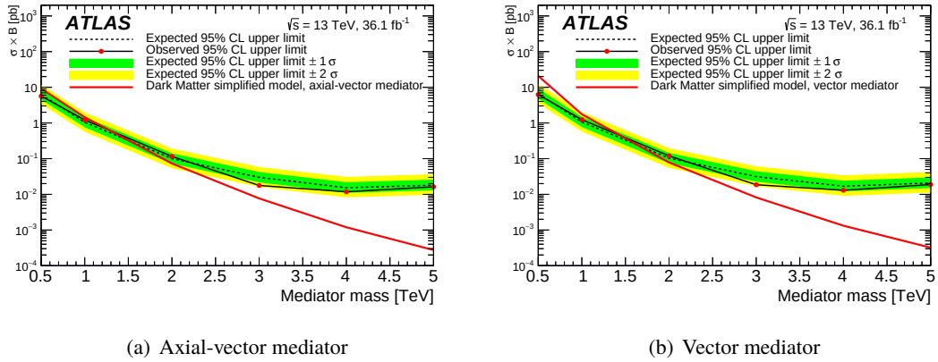
Figure 15: The observed and expected cross-section 95% CL upper limits on the (a) Z'_{DM,ax} and (b) Z'_{DM,vec} signals. The theoretical predictions for the production cross-section times branching ratio of Z'_{DM} \rightarrow t\bar{t} at the corresponding masses are also shown.
