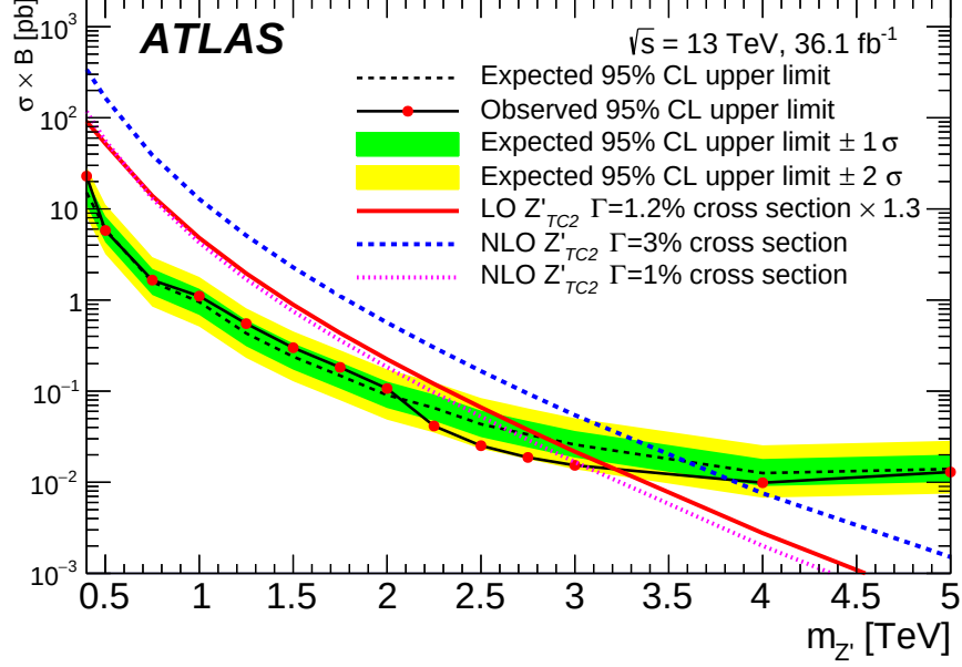
Figure 14: The observed and expected cross-section 95% CL upper limits on the Z'_{TC2} signal. The theoretical predictions for the production cross-section times branching ratio of Z'_{TC2} \rightarrow t\bar{t} at the corresponding masses are also shown.
