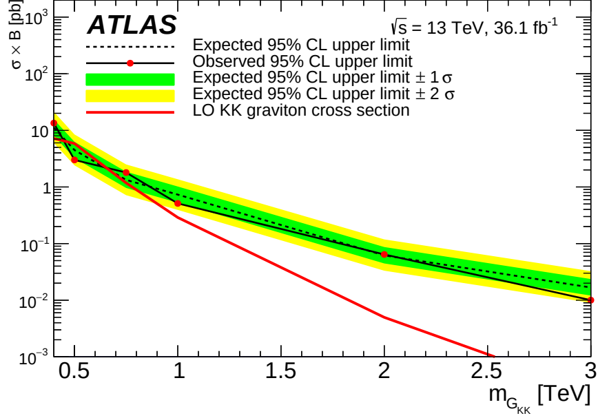
Figure 16: The observed and expected cross-section 95% CL upper limits on the G_{KK} signal. The theoretical predictions for the production cross-section times branching ratio of G_{KK} \rightarrow t\bar{t} at the corresponding masses are also shown.
