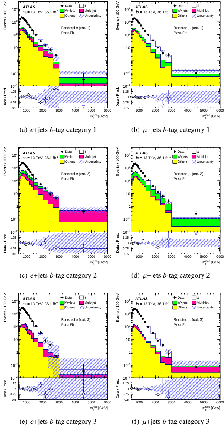
Figure 12: The m_{t\bar{t}}^{\text{reco}} distributions, after a likelihood fit under the background-only hypothesis, for the boosted selection. The SM background components are shown as stacked histograms. The shaded areas indicate the total systematic uncertainties. The ratio of the data to the final fitted expectation is shown in the lower panel, open triangles indicate that the ratio point would appear outside the panel.
