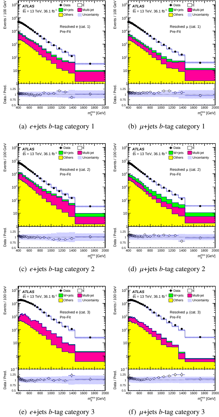
Figure 11: The m_{t\bar{t}}^{\text{reco}} distribution before the likelihood fit in the resolved selection. The SM background components are shown as stacked histograms. The shaded areas indicate the total systematic uncertainties. The ratio of the data to the total expectation from background processes is shown in the lower panel.
