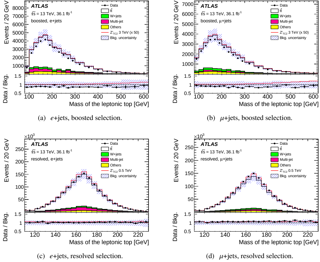
Figure 8: The distribution of the reconstructed mass of the leptonic-top candidate in the (a) boosted e +jets, (b) boosted \mu +jets, (c) resolved e +jets, and (d) resolved \mu +jets selections. The SM background components are shown as stacked histograms. The shaded areas indicate the total systematic uncertainties. The lower panels in each plot show the ratio of data (points) and a signal example (line) to the background expectation.
