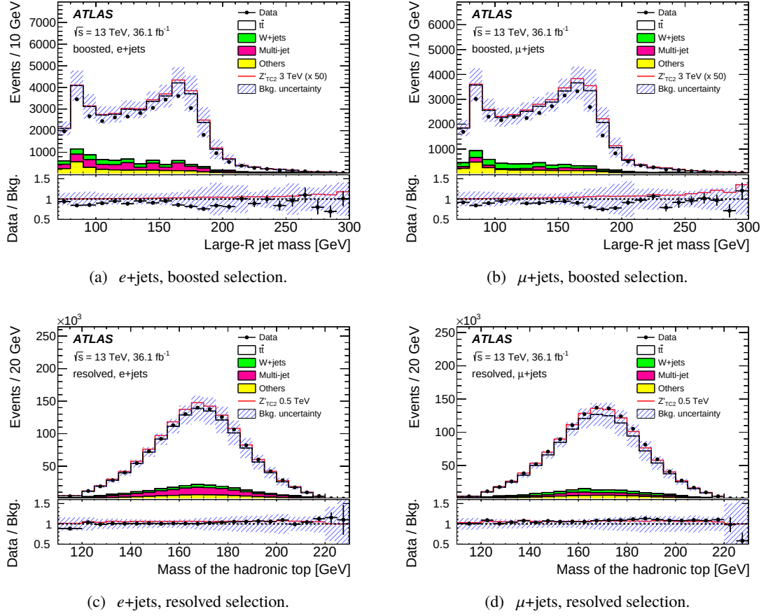
Figure 9: The distribution of the mass of the large- R jet in the (a) boosted e +jets, and (b) boosted \mu +jets selections. The mass of the hadronic-top candidate in the (c) resolved e +jets, and (d) resolved \mu +jets selections. The SM background components are shown as stacked histograms. The shaded areas indicate the total systematic uncertainties. The lower panels in each plot show the ratio of data (points) and a signal example (line) to the background expectation.
