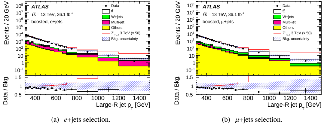
Figure 7: The distribution of the transverse momentum of the large- R jet in the (a) boosted e +jets, and (b) boosted \mu +jets selections. The SM background components are shown as stacked histograms. The shaded areas indicate the total systematic uncertainties. The lower panels in each plot show the ratio of data (points) and a signal example (line) to the background expectation.
