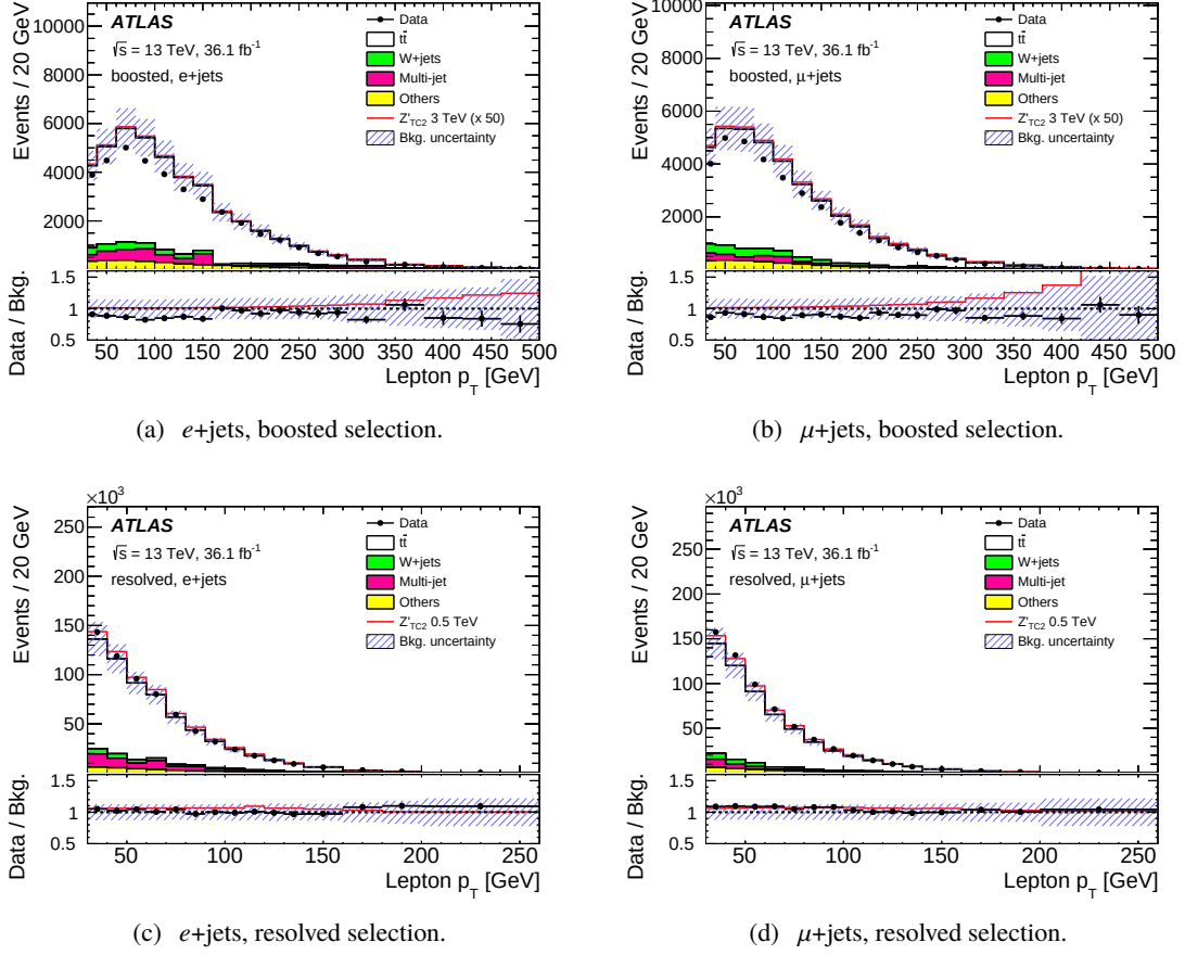
Figure 4: The distribution of the transverse momentum of the lepton in the (a) boosted e +jets, (b) boosted \mu +jets, (c) resolved e +jets, and (d) resolved \mu +jets selections. The SM background components are shown as stacked histograms. The shaded areas indicate the total systematic uncertainties. The lower panels in each plot show the ratio of data (points) and a signal example (line) to the background expectation.
