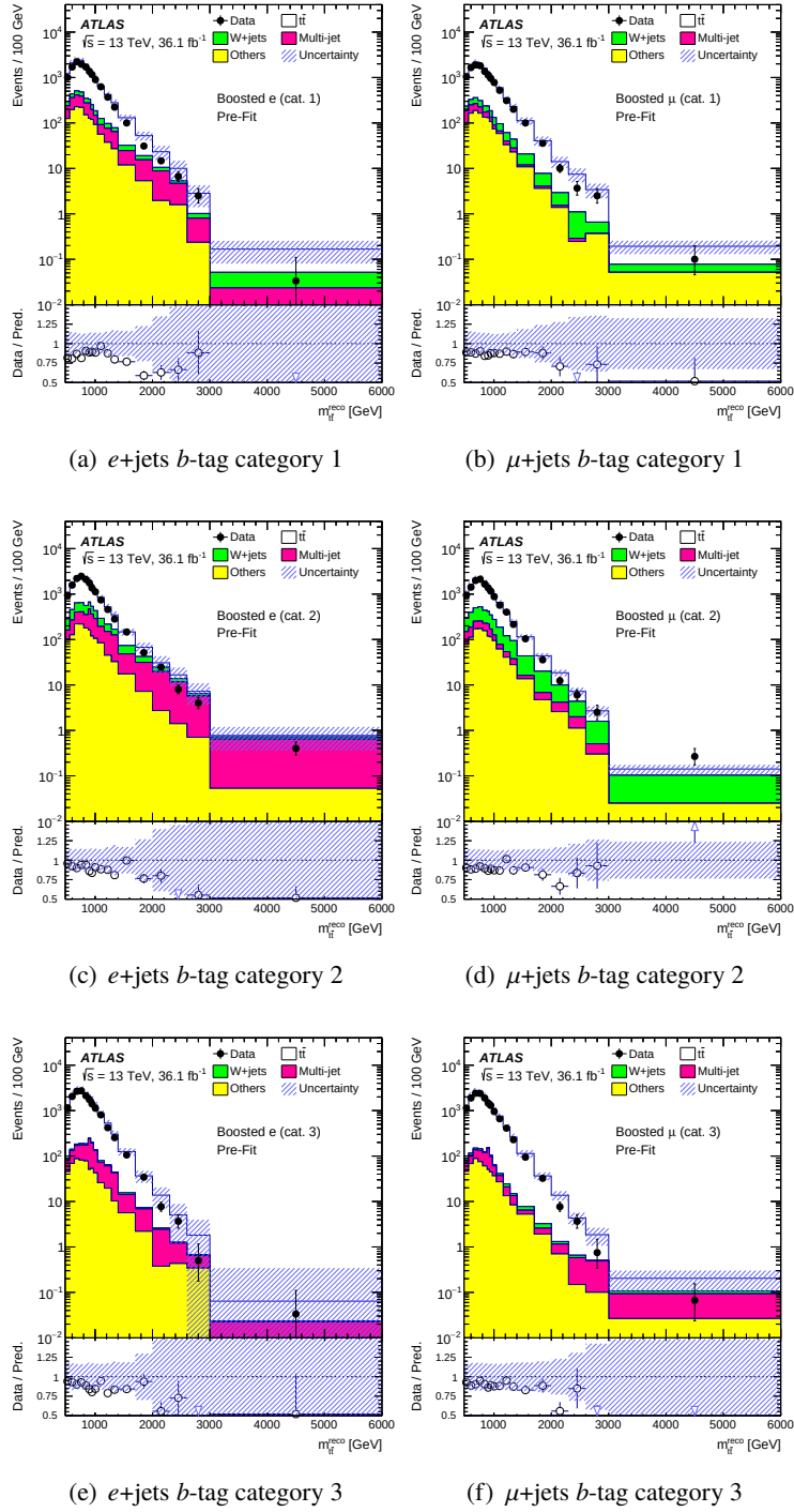
Figure 10: The m_{t\bar{t}}^{\text{reco}} distribution before the likelihood fit in the boosted selection. The SM background components are shown as stacked histograms. The shaded areas indicate the total systematic uncertainties. The ratio of the data to the total expectation from background processes is shown in the lower panel, open triangles indicate that the ratio point would appear outside the panel.
