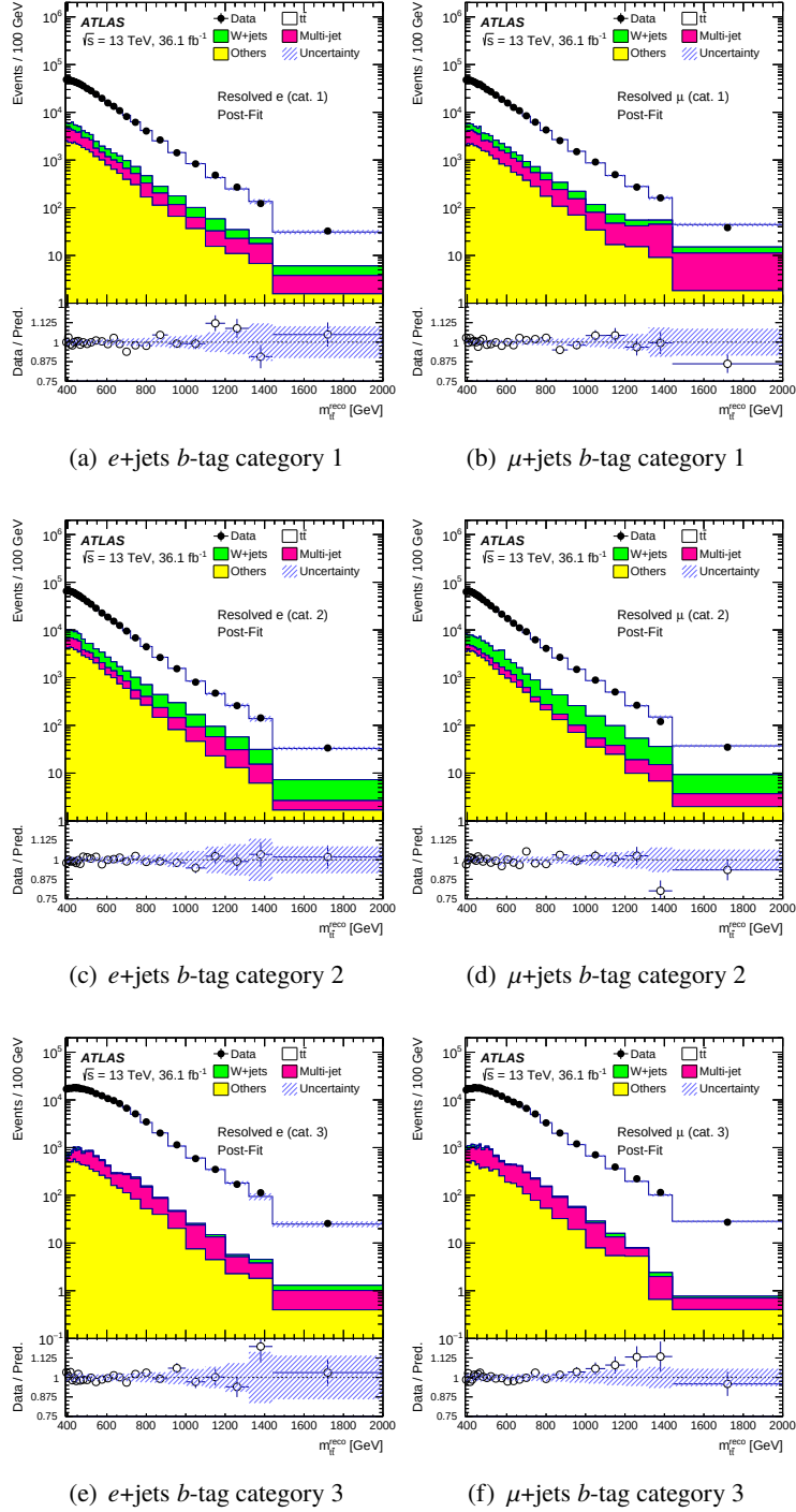
Figure 13: The m_{t\bar{t}}^{\text{reco}} distributions, after a likelihood fit under the background-only hypothesis, for the resolved selection. The SM background components are shown as stacked histograms. The shaded areas indicate the total systematic uncertainties. The ratio of the data to the final fitted expectation is shown in the lower panel.
