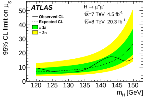
Figure 4: Observed (solid) and expected (dashed) 95% CL upper limits on the H \rightarrow \mu^+\mu^- signal strength as a function of m_H over the mass range 120–150 GeV. The dark- and light-shaded regions indicate the \pm 1\sigma and \pm 2\sigma uncertainty bands on the expected limit, respectively.
