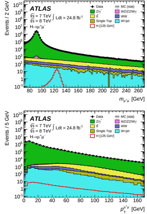
Figure 1: The distribution of the dimuon invariant mass (top) and dimuon momentum (bottom) for 7 TeV and 8 TeV data with all the selection requirements described in Section 3. The expected signal is shown for m_H = 125 GeV.
