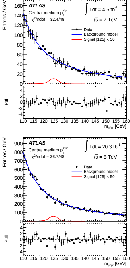
Figure 2: The background model fits to the m_{\mu^+\mu^-} distribution for the central medium p_T^{\mu^+\mu^-} category for 7 TeV (top) and 8 TeV (bottom) data. The statistical uncertainties are given for the data points. The expected signal is shown for m_H = 125 GeV and is scaled by a factor of 50.
