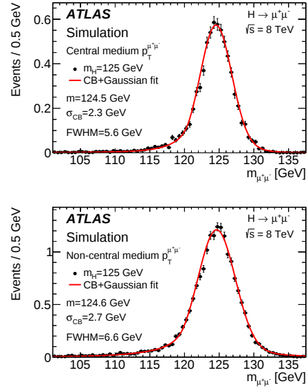
Figure 3: The signal model fit to the m_{\mu^+\mu^-} distribution for the central (top) and non-central (bottom) simulated Higgs boson events for m_H = 125 GeV in the medium p_T^{\mu^+\mu^-} category for \sqrt{s} = 8 TeV.
