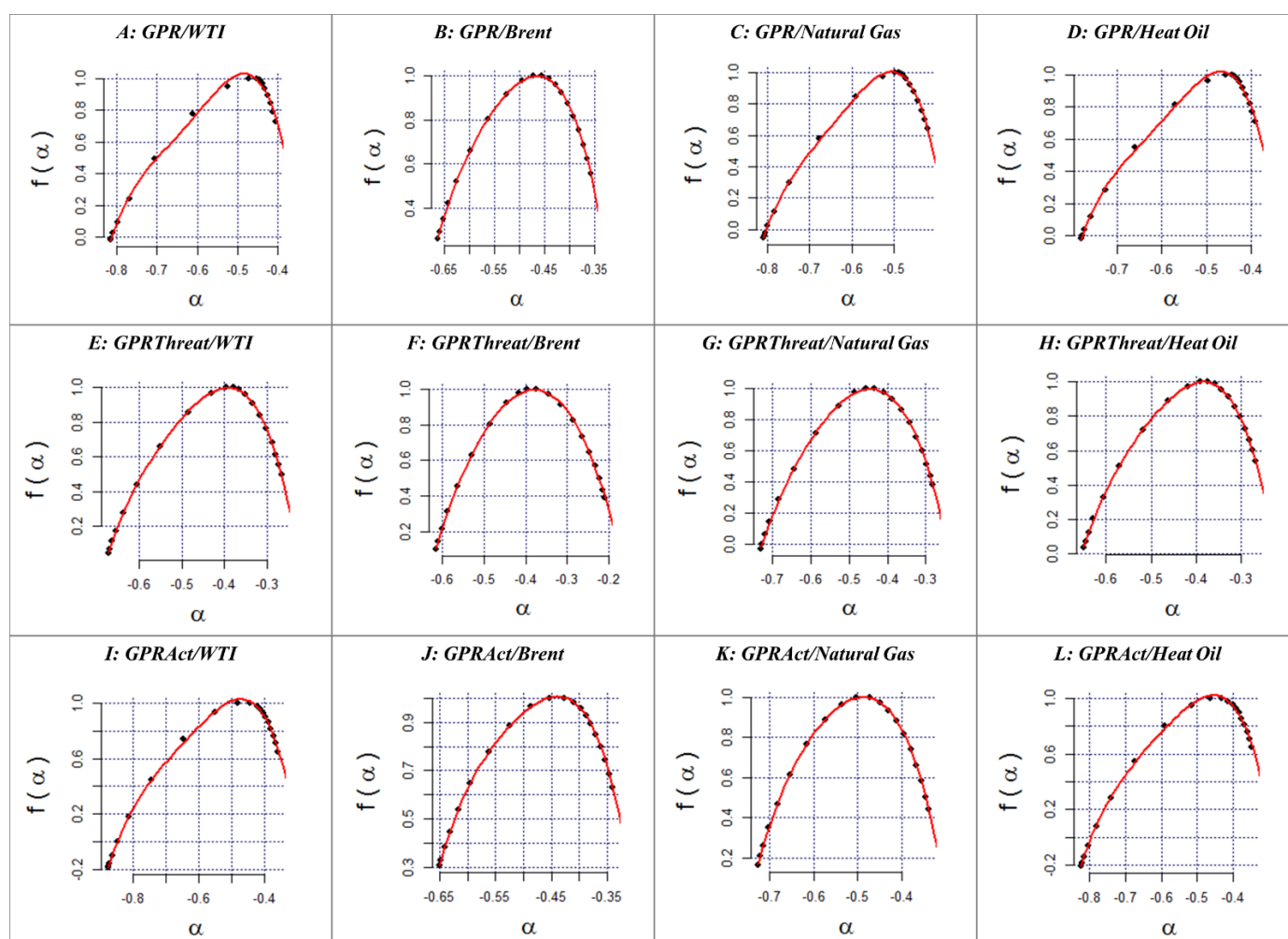
Figure 6. Multifractal spectrum.
