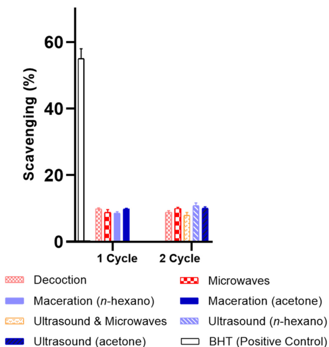
Figure 2. Graph of the antioxidant activity from the percentages of absorbance obtained by the extracts of each method.
