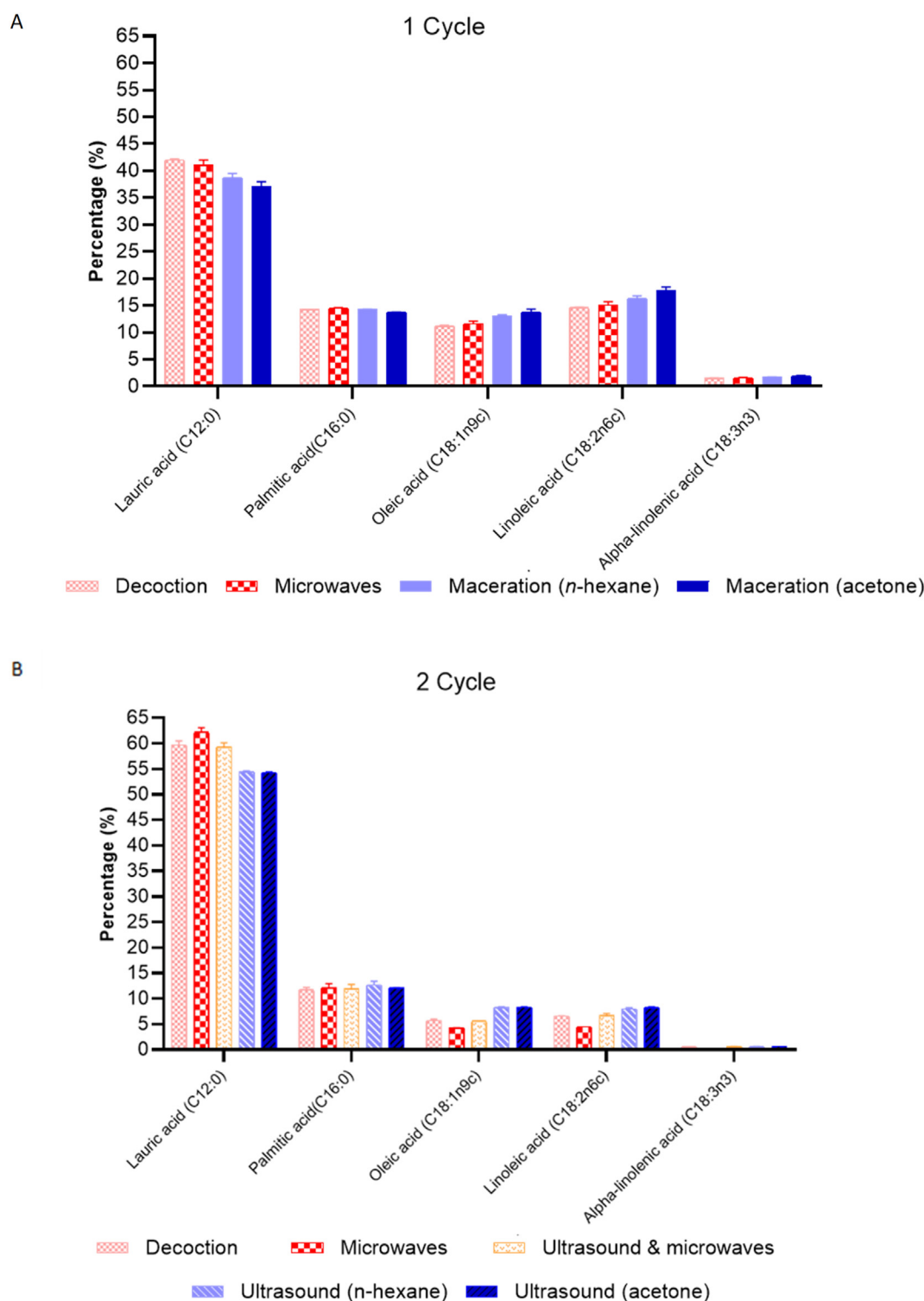
Figure 4. The main fatty acids composition in the BSF larvae lipid extracts. A) The first cycle of extraction; B) The second cycle of extraction.
