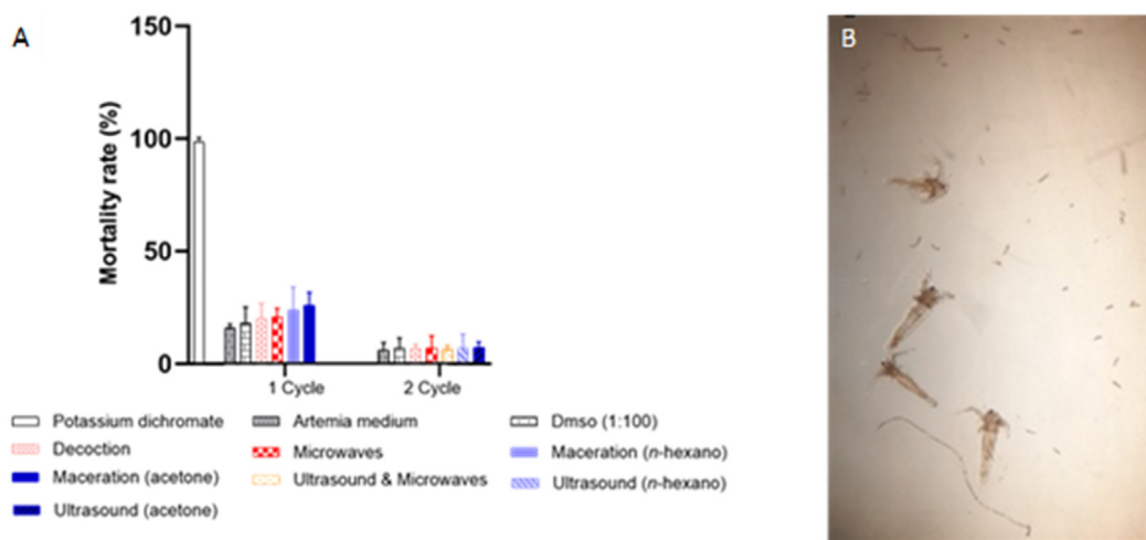
Figure 3. General Toxicity bioassay using A. salina . A) Graph with the mortality rate of nauplii; B) Alive A. salina nauplii.
