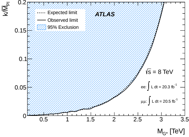
FIG. 8. Expected and observed 95% CL limits in the plane of the coupling strength of the Randall-Sundrum G^* to SM particles ( k/\bar{M}_{Pl} ) versus G^* mass for the combination of the dielectron and dimuon channels. The region above the curve is excluded at 95% CL.
