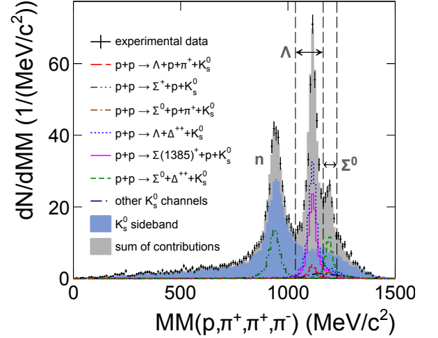
FIG. 2. Color online. Missing mass distribution with respect to the p , \pi^+ , \pi^+ and \pi^- with a cut on the K_S^0 mass in the \pi^+\pi^- -invariant mass spectrum (Fig. 1). The gray histogram corresponds to the sum of simulated contributions plus the background defined by the sideband sample. The double arrows indicate the so-called \Lambda -cut and \Sigma^0 -cut, respectively. See text for details.
