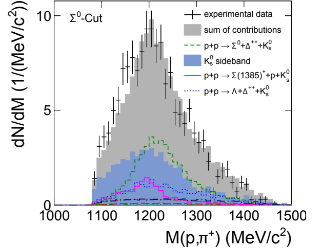
FIG. 8. Color online. p\pi^+ -invariant mass distribution after the \Sigma^0 -cut on the MM(p,\pi^+,\pi^+,\pi^-) distribution (Fig. 2) and with a cut on the K_s^0 mass in the \pi^+\pi^- -invariant mass spectrum (Fig. 1). The gray histogram corresponds to the sum of simulated contributions plus the background defined by the sideband sample. The same color code and line styles are used as in Figs. 2, 3 and 6.
