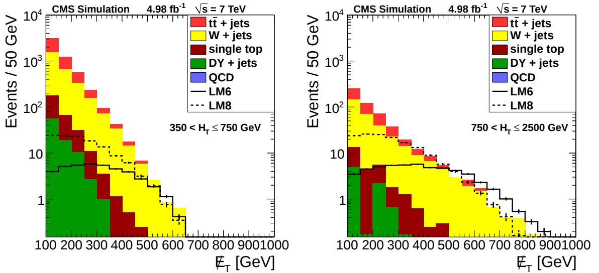
Figure 3: Distribution of E_T in the muon channel: simulation of backgrounds and two reference SUSY signals (LM6 and LM8) for (left) 350 < H_T \leq 750 GeV and (right) 750 < H_T \leq 2500 GeV. No requirements are imposed on the number of b jets.
