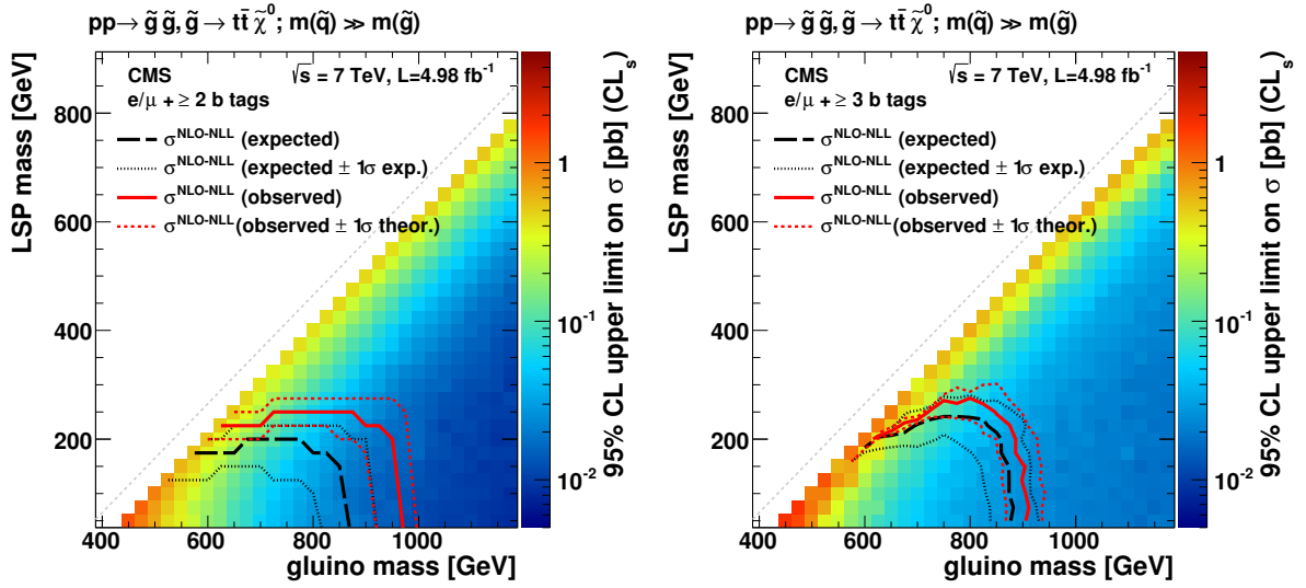
Figure 10: The 95% CL upper limit on the cross section using the CL_s technique for the simplified model shown in Fig. 1 for (left) the E_T template method, where at least two b tags are required, and (right) the factorization method with three or more b tags. The area below the thick solid red line is excluded. The thick dashed black line represents the expected limit. The diagonal dashed line marks the lower kinematical limit of the LSP mass.
