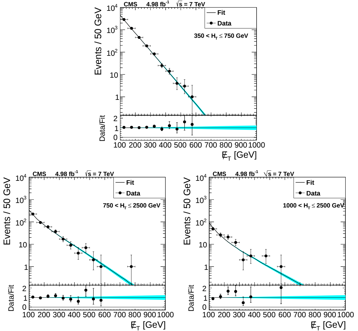
Figure 7: Distribution of E_T in the muon channel: data (points) and fit result of the template method (line) for (top) 350 < H_T < 750 GeV; data and prediction obtained from the fit for (bottom left) 750 < H_T < 2500 GeV and for (bottom right) 1000 < H_T < 2500 GeV. The bands around the fit correspond to the statistical uncertainty on the parameter \alpha . The systematic uncertainties have been calculated for E_T > 250, 350 and 450 GeV and range from 16 – 32% (24 – 42%) for H_T > 750 (1000) GeV as reported in Tab. 9. The lower panels show the ratio between the fitted model and data.
