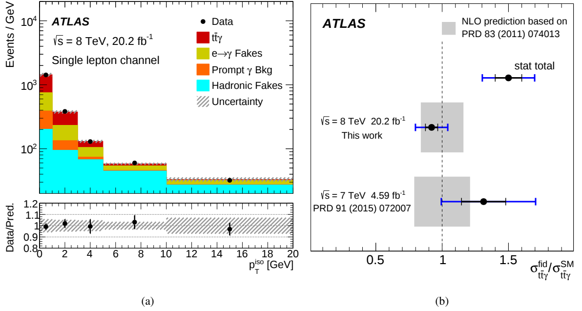
Figure 3: (a) Post-fit track isolation distribution for the inclusive cross-section measurement. The last bin includes the overflow. The uncertainty band includes all uncertainties. (b) Summary of fiducial measurements of t\bar{t}\gamma production in pp collisions at 7 TeV [8] and 8 TeV, normalised to the expected cross section, calculated at NLO accuracy [9].
