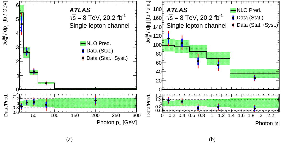
Figure 4: Measured differential cross section in (a) p_T and (b) |\eta| and the corresponding theoretical prediction.
